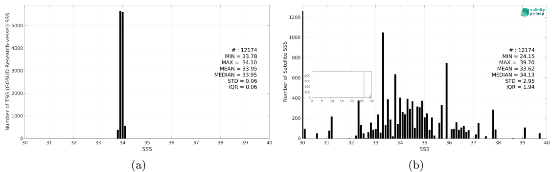
Figure 3: Histograms of SSS from TSG (GOSUD-Research-vessel) (a) and SMAP SSS L2 v5.0 (JPL) (b) considering all match-up pairs per bins of 0.1 over the Southern Ocean Pi-MEP region and for the full satellite product period.
