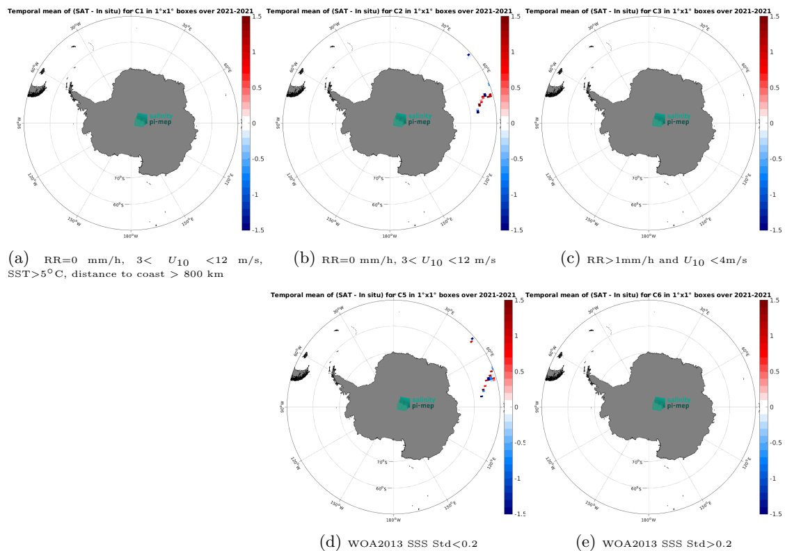
Figure 14: Temporal mean gridded over spatial boxes of size 1^\circ \times 1^\circ of \Delta\text{SSS} (SMAP SSS L2 v5.0 (JPL) - TSG (GOSUD-Research-vessel)) for 5 different subdatasets corresponding to:RR=0 mm/h, 3 < U_{10} < 12 m/s, SST>5°C, distance to coast > 800 km (a), RR=0 mm/h, 3 < U_{10} < 12 m/s (b), RR>1mm/h and U_{10} < 4 m/s (c), WOA2013 SSS Std<0.2 (d), WOA2013 SSS Std>0.2 (e).
