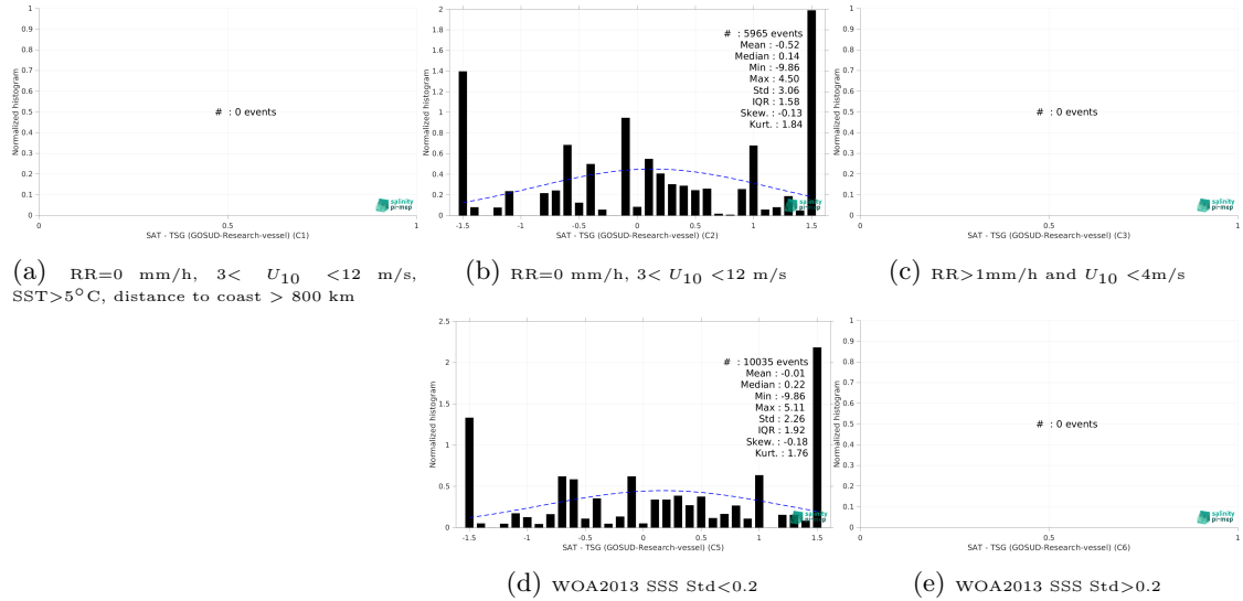
Figure 15: Normalized histogram of \Delta SSS (SMAP SSS L2 v5.0 (JPL) - TSG (GOSUD-Research-vessel)) for 5 different subdatasets corresponding to: RR=0 mm/h, 3 < U_{10} < 12 m/s, SST > 5°C, distance to coast > 800 km (a), RR=0 mm/h, 3 < U_{10} < 12 m/s (b), RR > 1mm/h and U_{10} < 4 m/s (c), WOA2013 SSS Std < 0.2 (d), WOA2013 SSS Std > 0.2 (e).
