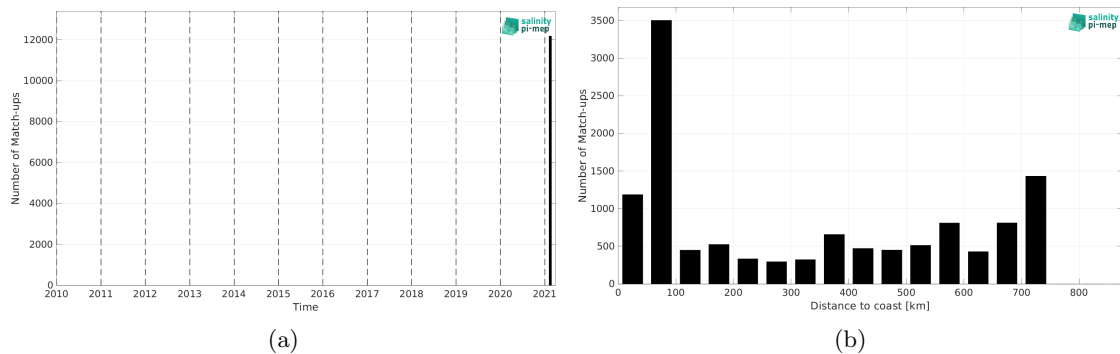
Figure 2: Number of match-ups between TSG (GOSUD-Research-vessel) and SMAP SSS L2 v5.0 (JPL) SSS as a function of time (a) and as function of the distance to coast (b) over the Southern Ocean Pi-MEP region and for the full satellite product period.
