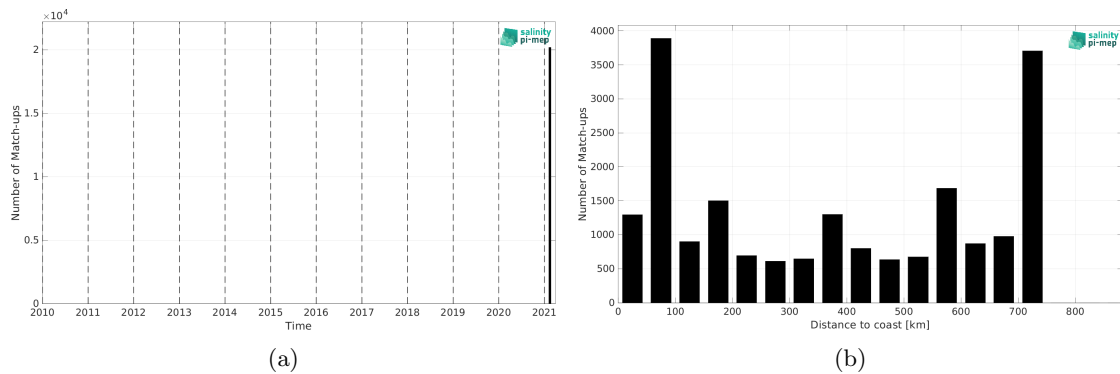
Figure 1: Number of match-ups between TSG (GOSUD-Research-vessel) and SMAP SSS L2 v5.0 (JPL) SSS as a function of time (a) and as function of the distance to coast (b) over the Southern Ocean Pi-MEP region and for the full satellite product period.
