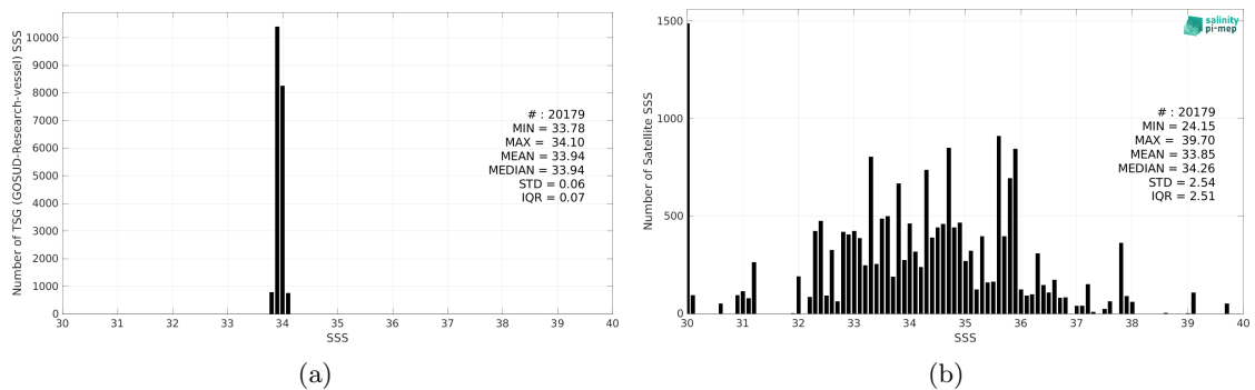
Figure 2: Histograms of SSS from TSG (GOSUD-Research-vessel) (a) and SMAP SSS L2 v5.0 (JPL) (b) considering all match-up pairs per bins of 0.1 over the Southern Ocean Pi-MEP region and for the full satellite product period.
