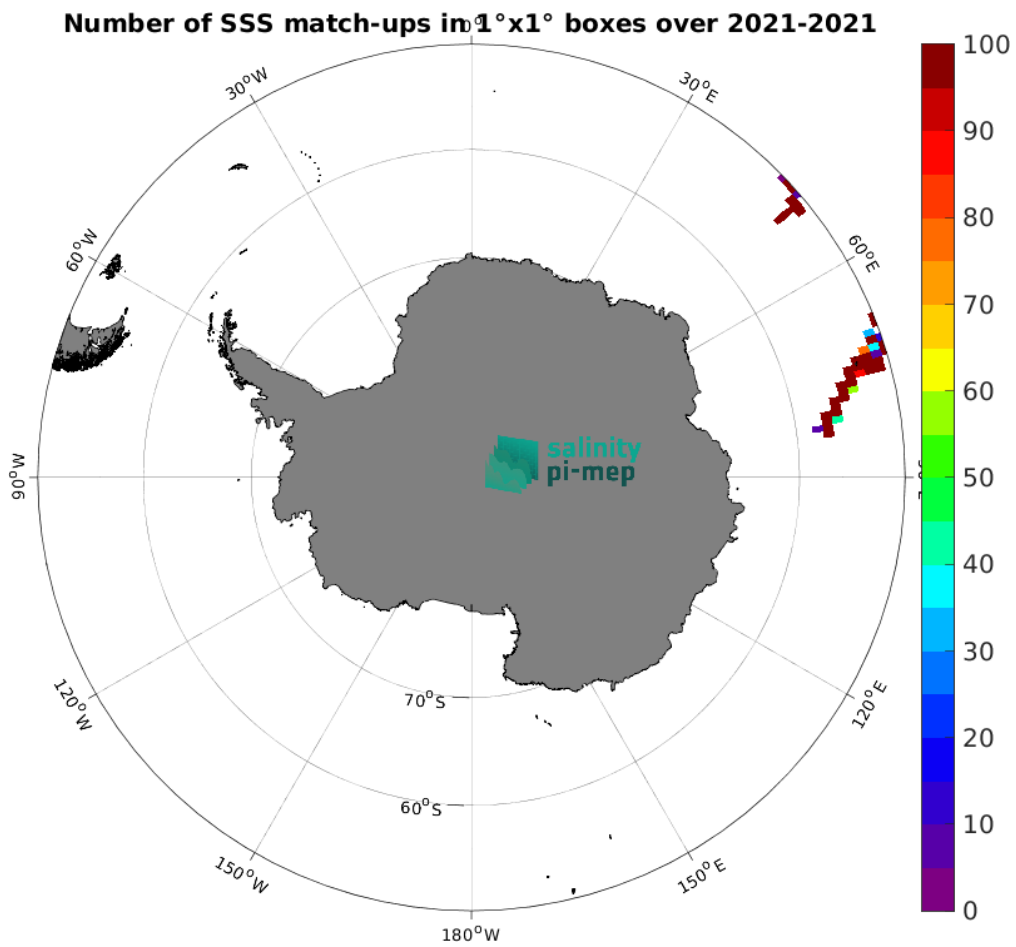
Figure 4: Number of SSS match-ups between TSG (GOSUD-Research-vessel) SSS and the SMAP SSS L2 v5.0 (JPL) SSS product for the Southern Ocean Pi-MEP region over 1^\circ \times 1^\circ boxes and for the full satellite product period.
