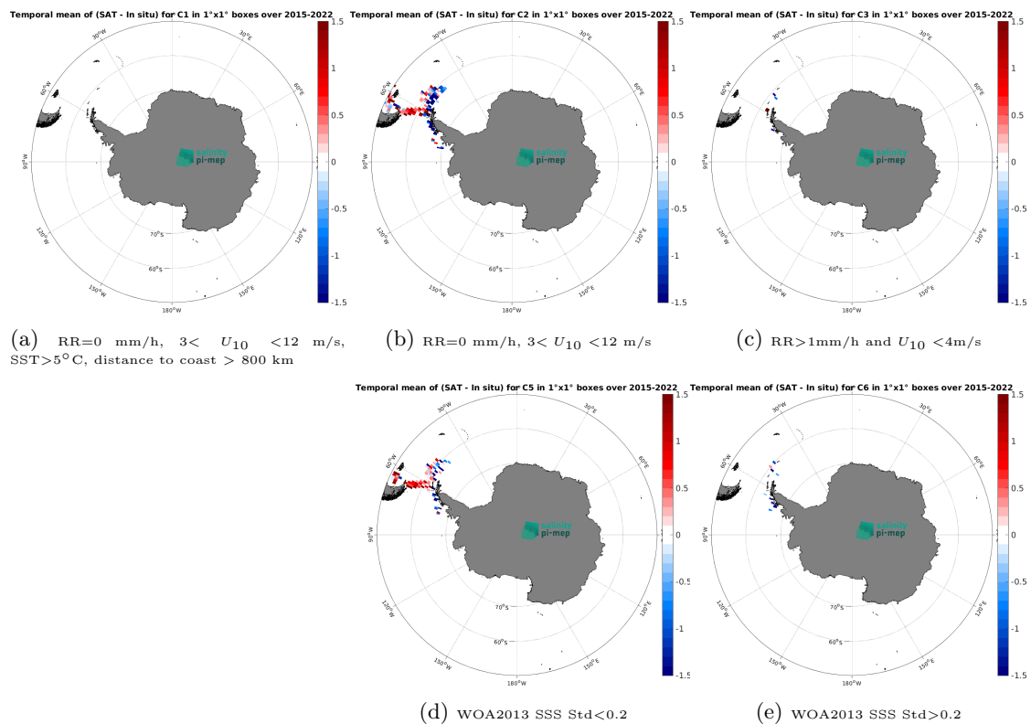
Figure 14: Temporal mean gridded over spatial boxes of size 1^\circ \times 1^\circ of \Delta SSS (SMAP SSS L2 v5.0 (JPL) - TSG (CSIC-UTM)) for 5 different subdatasets corresponding to:RR=0 mm/h, 3 < U_{10} < 12 m/s, SST >5^\circ\text{C} , distance to coast > 800 km (a), RR=0 mm/h, 3 < U_{10} < 12 m/s (b), RR >1 mm/h and U_{10} < 4 m/s (c), WOA2013 SSS Std <0.2 (d), WOA2013 SSS Std >0.2 (e).
