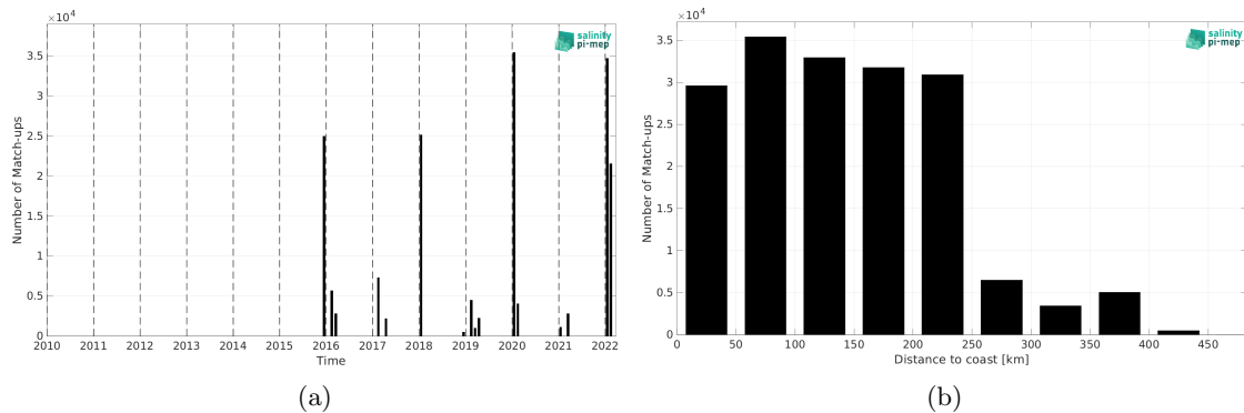
Figure 2: Number of match-ups between TSG (CSIC-UTM) and SMAP SSS L2 v5.0 (JPL) SSS as a function of time (a) and as function of the distance to coast (b) over the Southern Ocean Pi-MEP region and for the full satellite product period.
