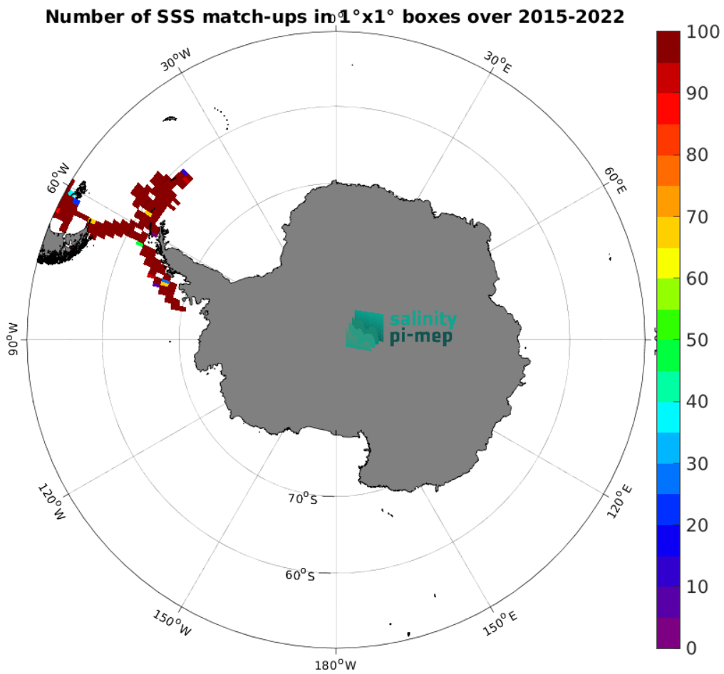
Figure 5: Number of SSS match-ups between TSG (CSIC-UTM) SSS and the SMAP SSS L2 v5.0 (JPL) SSS product for the Southern Ocean Pi-MEP region over 1^\circ \times 1^\circ boxes and for the full satellite product period.
