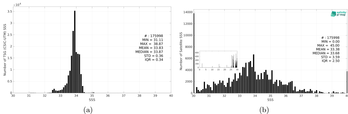
Figure 3: Histograms of SSS from TSG (CSIC-UTM) (a) and SMAP SSS L2 v5.0 (JPL) (b) considering all match-up pairs per bins of 0.1 over the Southern Ocean Pi-MEP region and for the full satellite product period.
