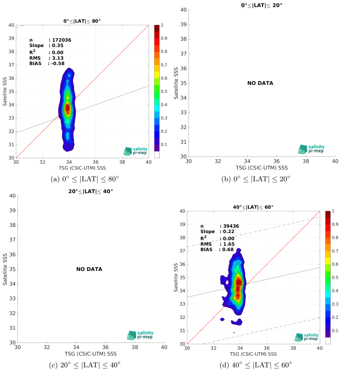
Figure 10: Contour maps of the concentration of SMAP SSS L2 v5.0 (JPL) SSS (y-axis) versus TSG (CSIC-UTM) SSS (x-axis) at match-up pairs for different latitude bands. For each plot, the red line shows x=y . The black thin and dashed lines indicate a linear fit through the data cloud and the \pm 95\% confidence levels, respectively. The number match-up pairs n , the slope and R^2 coefficient of the linear fit, the root mean square (RMS) and the mean bias between satellite and in situ data are indicated for each latitude band in each plot.
