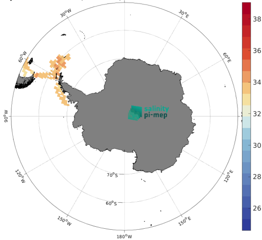
(c) MEAN(TSG (CSIC-UTM) SSS)
