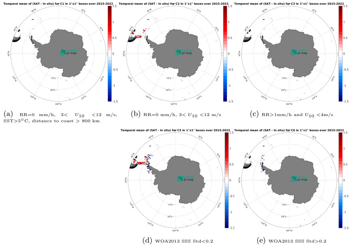
Figure 12: Temporal mean gridded over spatial boxes of size 1^{\circ}\times 1^{\circ} of \Delta\text{SSS} (SMAP SSS L2 v5.0 (JPL) - TSG (CSIC-UTM)) for 5 different subdatasets corresponding to: \text{RR}=0 mm/h, 3 < U_{10} < 12 m/s, \text{SST}>5^{\circ}\text{C} , distance to coast > 800 km (a), \text{RR}=0 mm/h, 3 < U_{10} < 12 m/s (b), \text{RR}>1\text{mm/h} and U_{10} < 4\text{m/s} (c), WOA2013 SSS Std < 0.2 (d), WOA2013 SSS Std > 0.2 (e).
