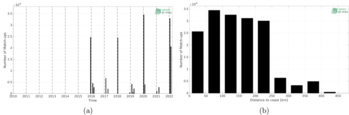
Figure 1: Number of match-ups between TSG (CSIC-UTM) and SMAP SSS L2 v5.0 (JPL) SSS as a function of time (a) and as function of the distance to coast (b) over the Southern Ocean Pi-MEP region and for the full satellite product period.
