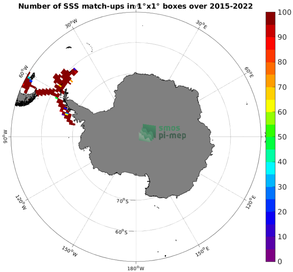
Figure 4: Number of SSS match-ups between TSG (CSIC-UTM) SSS and the SMAP SSS L2 v5.0 (JPL) SSS product for the Southern Ocean Pi-MEP region over 1^\circ \times 1^\circ boxes and for the full satellite product period.
