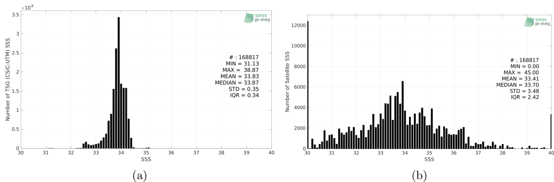
Figure 2: Histograms of SSS from TSG (CSIC-UTM) (a) and SMAP SSS L2 v5.0 (JPL) (b) considering all match-up pairs per bins of 0.1 over the Southern Ocean Pi-MEP region and for the full satellite product period.
