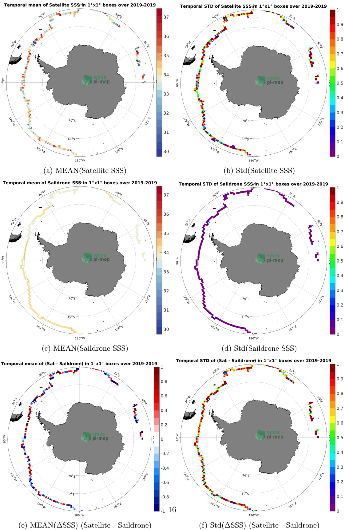
Figure 6: Temporal mean (left) and Std (right) of SSS from SMAP SSS L2 v5.0 (JPL) (top), Saildrone (middle), and of \Delta SSS (Satellite - Saildrone). Only match-up pairs are used to generate these maps.
