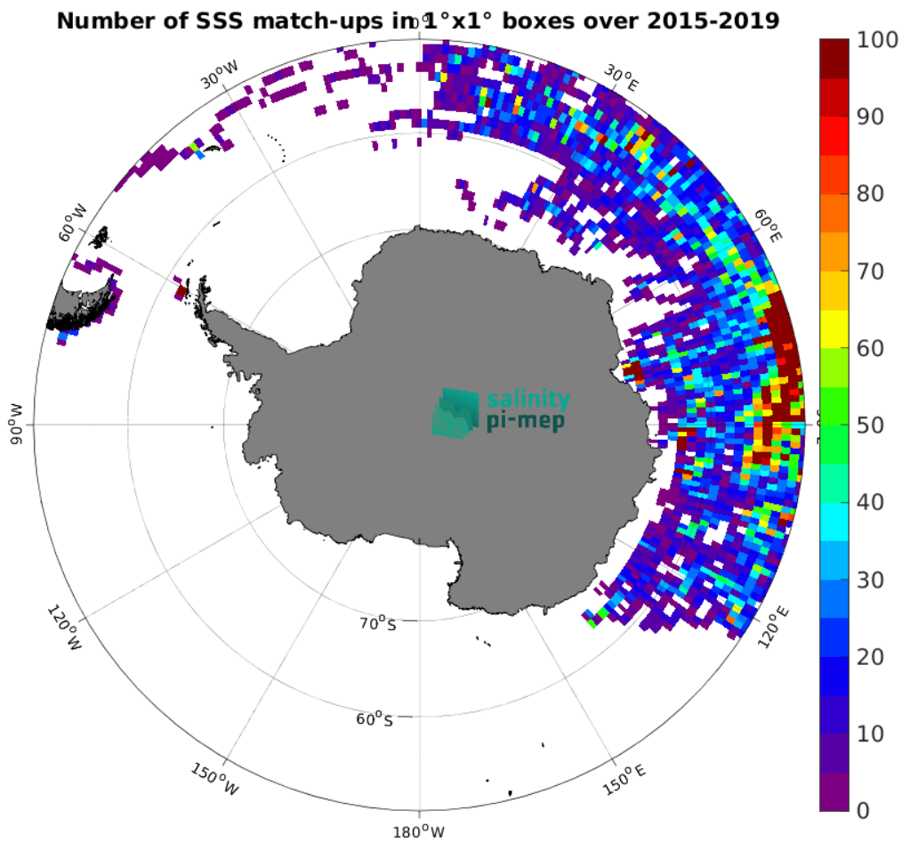
Figure 4: Number of SSS match-ups between Marine mammals SSS and the SMAP SSS L2 v5.0 (JPL) SSS product for the Southern Ocean Pi-MEP region over 1^{\circ} \times 1^{\circ} boxes and for the full satellite product period.
