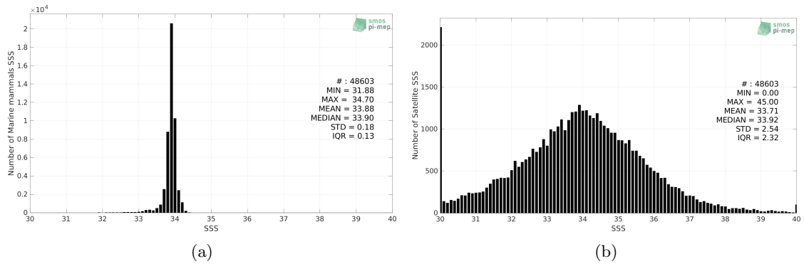
Figure 2: Histograms of SSS from Marine mammals (a) and SMAP SSS L2 v5.0 (JPL) (b) considering all match-up pairs per bins of 0.1 over the Southern Ocean Pi-MEP region and for the full satellite product period.
