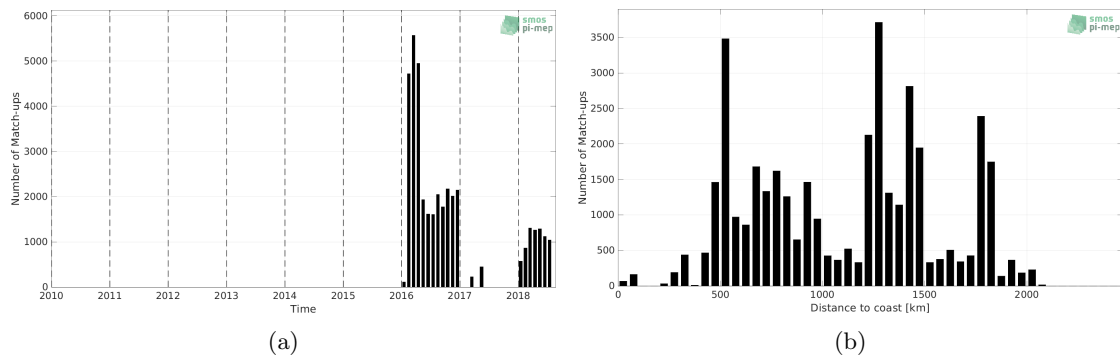
Figure 1: Number of match-ups between Surface drifters and SMAP SSS L2 v5.0 (JPL) SSS as a function of time (a) and as function of the distance to coast (b) over the Southern Ocean Pi-MEP region and for the full satellite product period.
