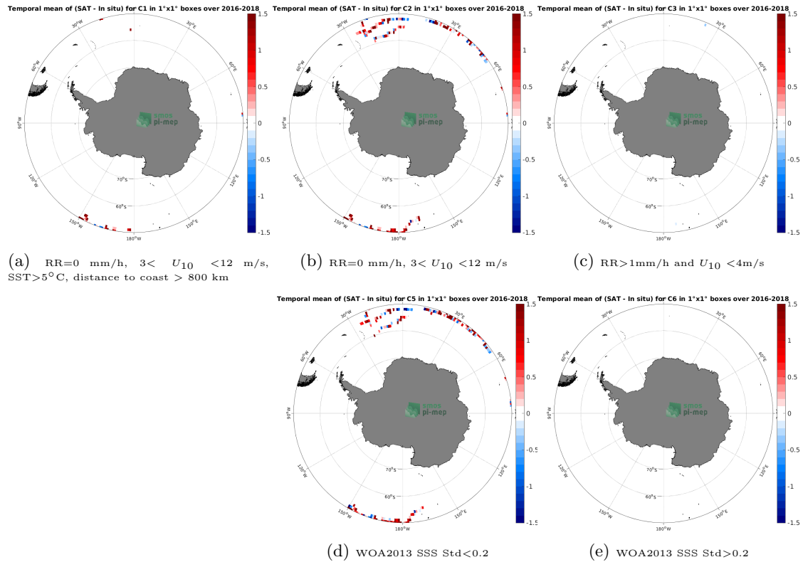
Figure 11: Temporal mean gridded over spatial boxes of size 1^{\circ}\times 1^{\circ} of \Delta\text{SSS} (SMAP SSS L2 v5.0 (JPL) - Surface drifters) for 5 different subdatasets corresponding to: \text{RR}=0 mm/h, 3 < U_{10} < 12 m/s, \text{SST}>5^{\circ}\text{C} , distance to coast > 800 km (a), \text{RR}=0 mm/h, 3 < U_{10} < 12 m/s (b), \text{RR}>1 mm/h and U_{10} < 4 m/s (c), WOA2013 SSS Std < 0.2 (d), WOA2013 SSS Std > 0.2 (e).
