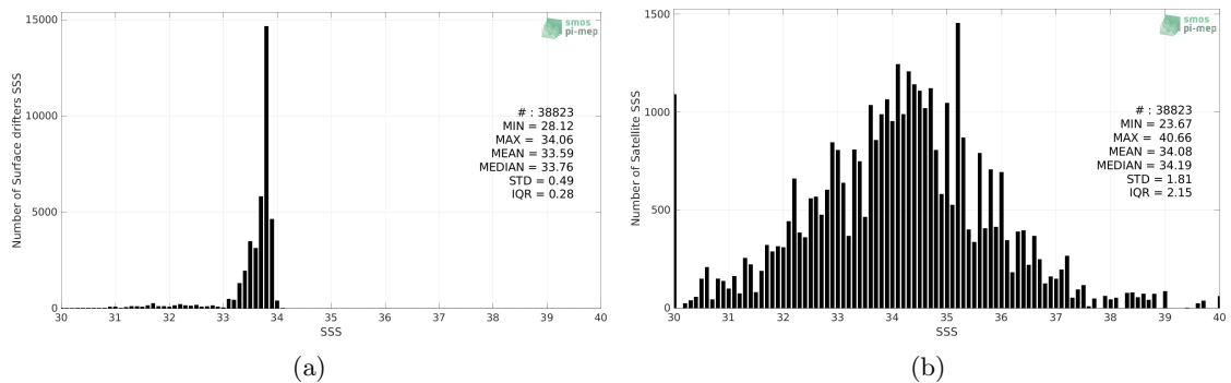
Figure 2: Histograms of SSS from Surface drifters (a) and SMAP SSS L2 v5.0 (JPL) (b) considering all match-up pairs per bins of 0.1 over the Southern Ocean Pi-MEP region and for the full satellite product period.
