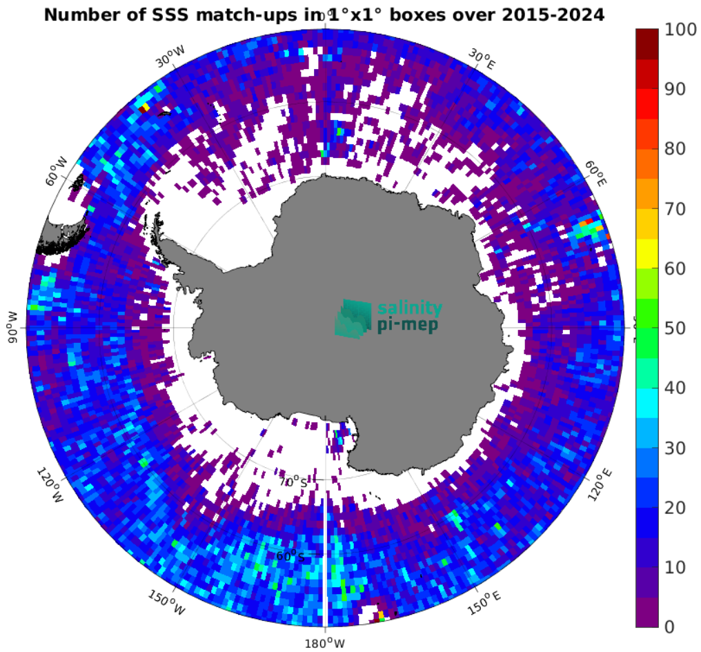
Figure 5: Number of SSS match-ups between Argo SSS and the SMAP SSS L2 v5.0 (JPL) SSS product for the Southern Ocean Pi-MEP region over 1^\circ \times 1^\circ boxes and for the full satellite product period.
