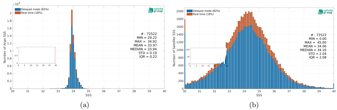
Figure 3: Histograms of SSS from Argo (a) and SMAP SSS L2 v5.0 (JPL) (b) considering all match-up pairs per bins of 0.1 over the Southern Ocean Pi-MEP region and for the full satellite product period.
