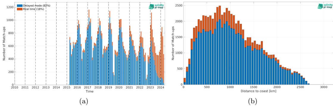
Figure 2: Number of match-ups between Argo and SMAP SSS L2 v5.0 (JPL) SSS as a function of time (a) and as function of the distance to coast (b) over the Southern Ocean Pi-MEP region and for the full satellite product period.
