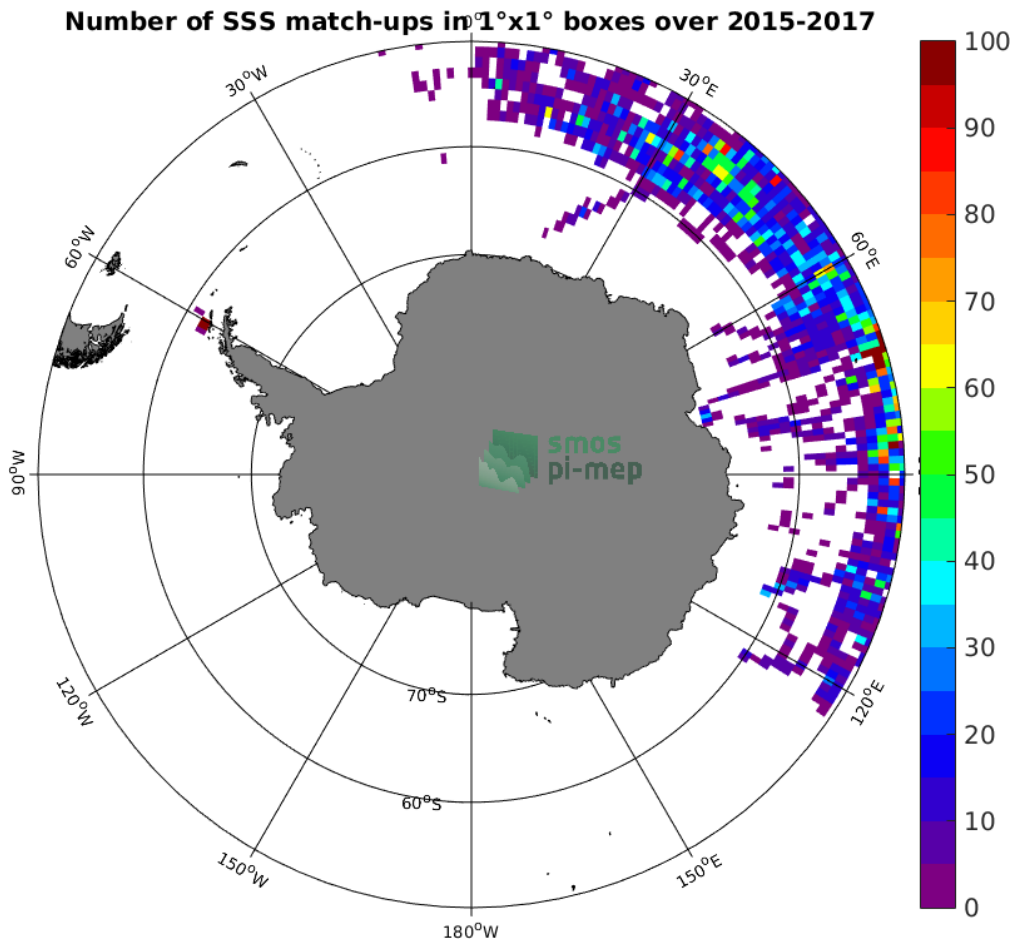
Figure 4: Number of SSS match-ups between Sea mammals SSS and the SMAP-L2-JPL-V4.3 SSS product for the Southern Ocean Pi-MEP region over 1^\circ \times 1^\circ boxes and for the full satellite product period.
