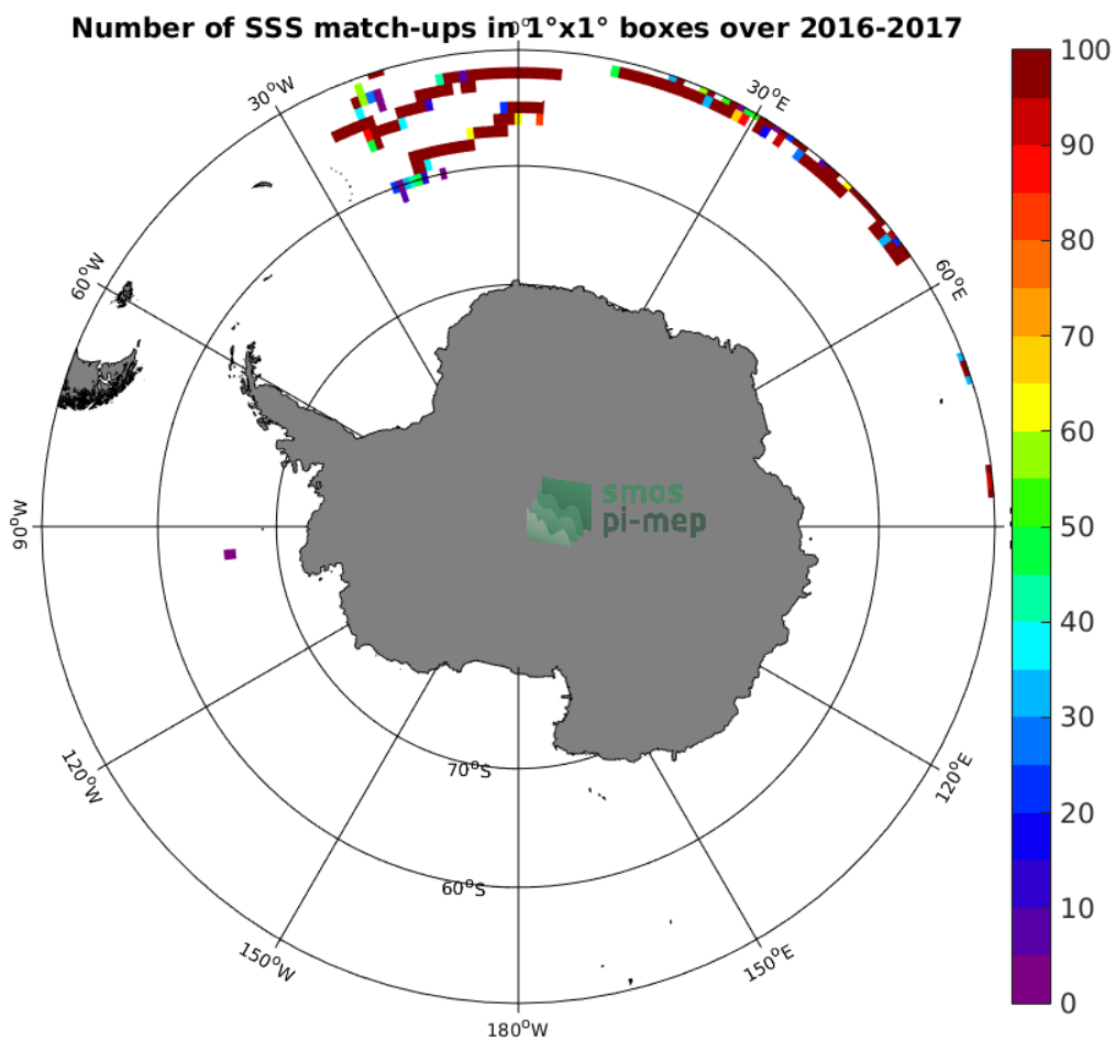
Figure 3: Number of SSS match-ups between Surface drifters SSS and the SMAP-L2-JPL-V4.3 SSS product for the Southern Ocean Pi-MEP region over 1^\circ \times 1^\circ boxes and for the full satellite product period.
