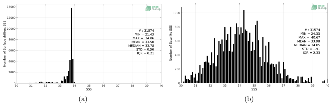
Figure 2: Histograms of SSS from Surface drifters (a) and SMAP-L2-JPL-V4.3 (b) considering all match-up pairs per bins of 0.1 over the Southern Ocean Pi-MEP region and for the full satellite product period.
