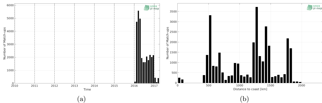
Figure 1: Number of match-ups between Surface drifters and SMAP-L2-JPL-V4.3 SSS as a function of time (a) and as function of the distance to coast (b) over the Southern Ocean Pi-MEP region and for the full satellite product period.
