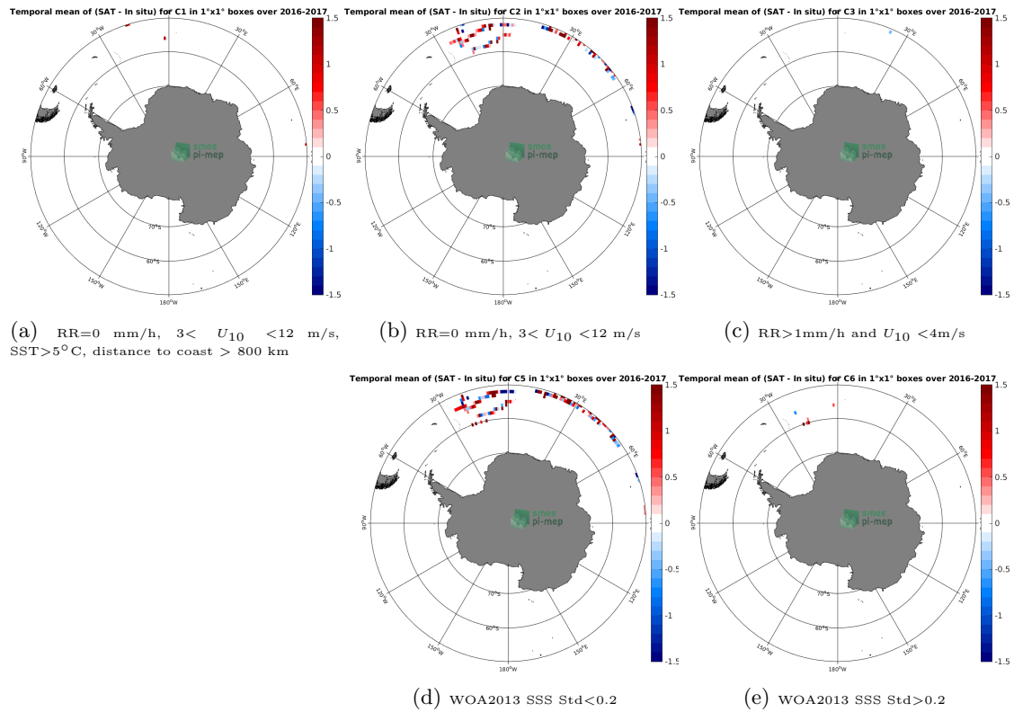
Figure 11: Temporal mean gridded over spatial boxes of size 1^\circ \times 1^\circ of \Delta SSS (SMAP-L2-JPL-V4.3 - Surface drifters) for 5 different subdatasets corresponding to:RR=0 mm/h, 3 < U_{10} < 12 m/s, SST >5^\circ C, distance to coast > 800 km (a), RR=0 mm/h, 3 < U_{10} < 12 m/s (b), RR >1 mm/h and U_{10} < 4 m/s (c), WOA2013 SSS Std <0.2 (d), WOA2013 SSS Std >0.2 (e).
