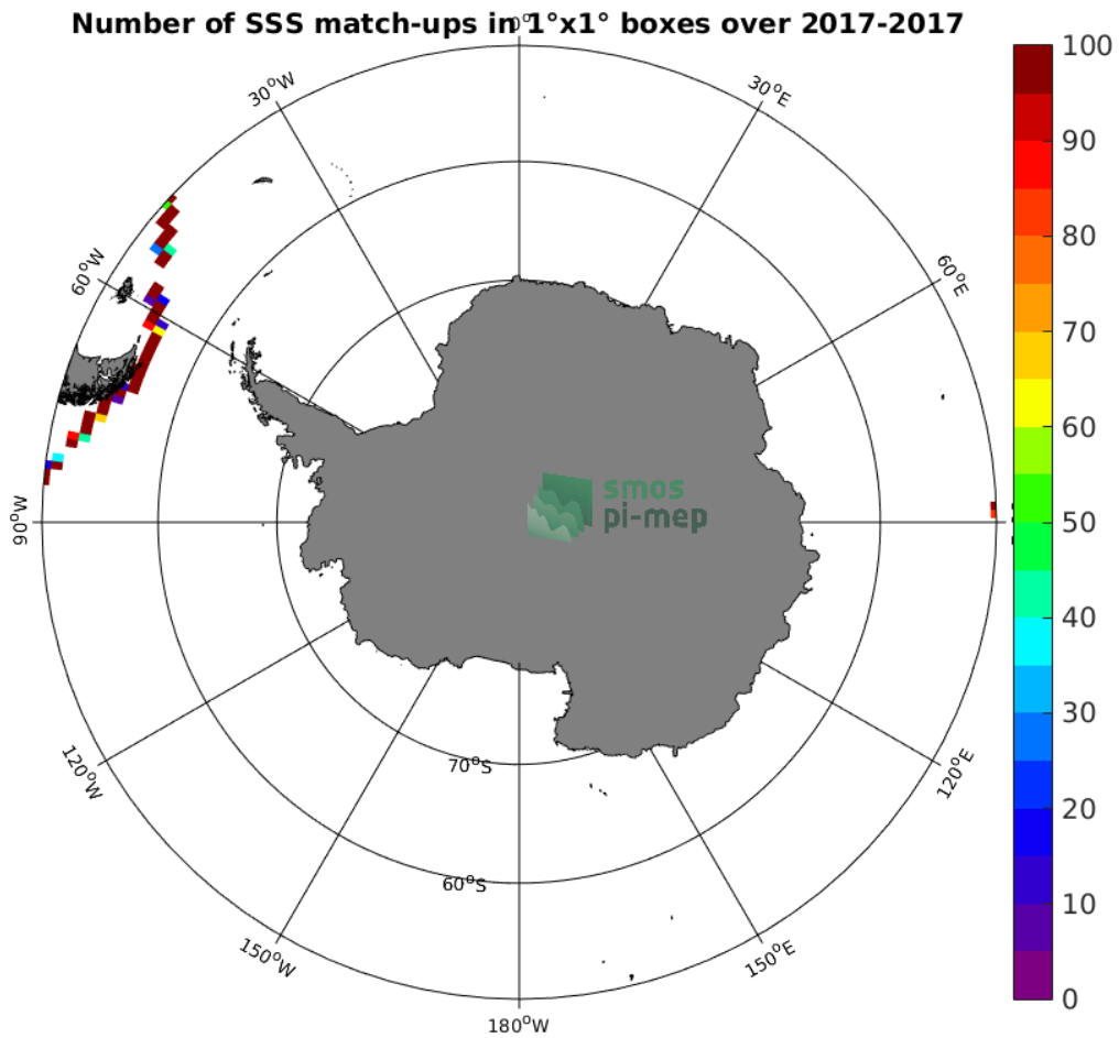
Figure 4: Number of SSS match-ups between TSG-GOSUD-Sailing-ship SSS and the SMAP-L2-JPL-V4.2 SSS product for the Southern Ocean Pi-MEP region over 1^\circ \times 1^\circ boxes and for the full satellite product period.
