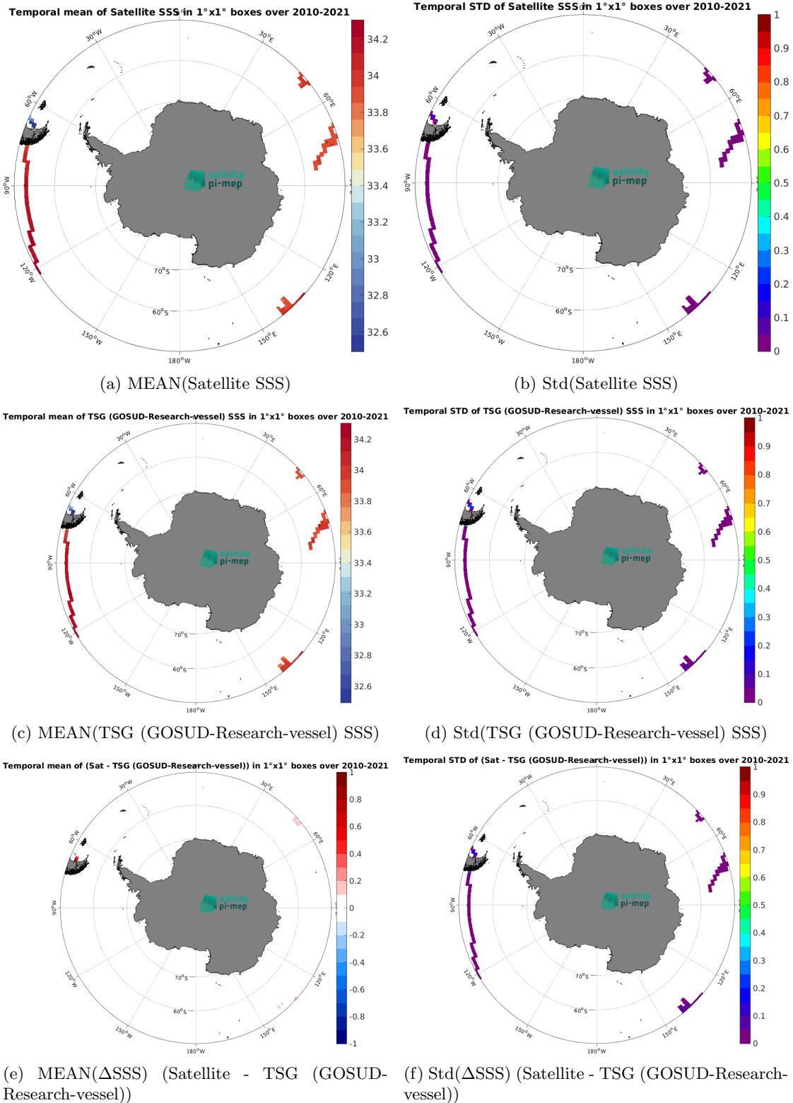
Figure 7: Temporal mean (left) and Std (right) of SSS from ISAS v7 - Monthly (Ifremer-LOPS-CMEMS) (top), TSG (GOSUD-Research-vessel) (middle), and of \Delta SSS (Satellite - TSG (GOSUD-Research-vessel)). Only match-up pairs are used to generate these maps.
