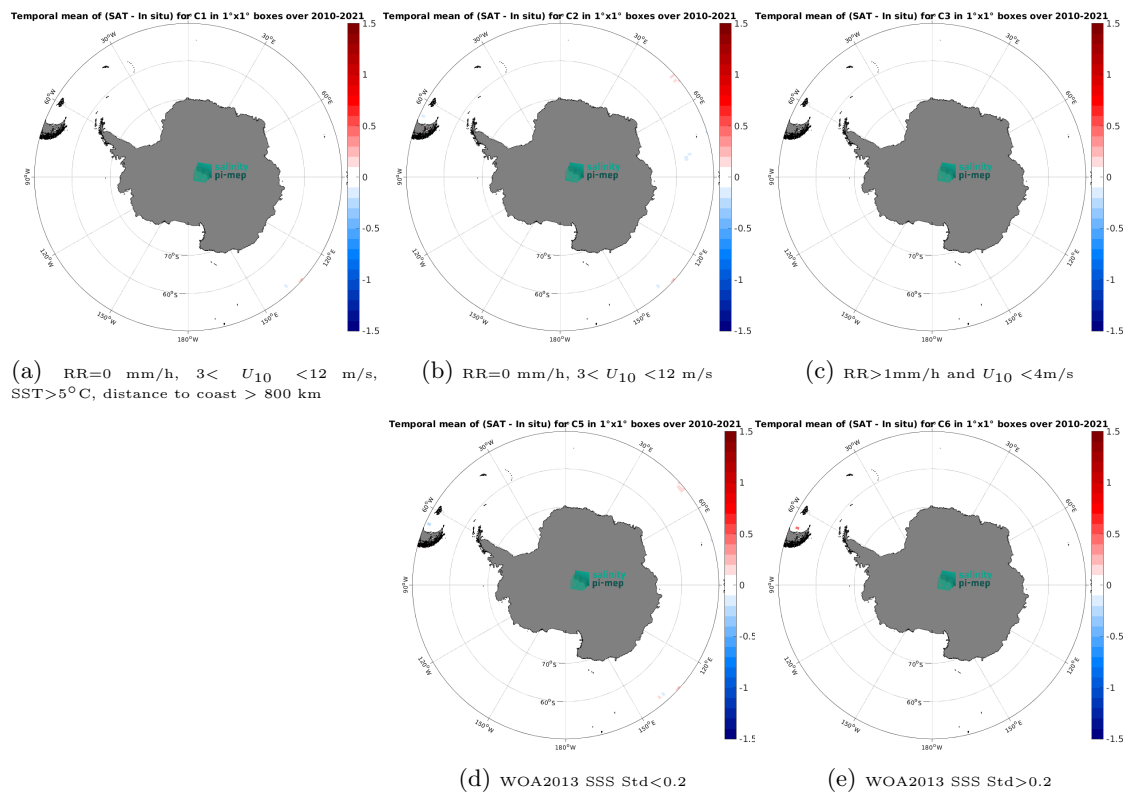
Figure 14: Temporal mean gridded over spatial boxes of size 1^\circ \times 1^\circ of \Delta SSS (ISAS v7 - Monthly (Ifremer-LOPS-CMEMS) - TSG (GOSUD-Research-vessel)) for 5 different subdatasets corresponding to: RR=0 mm/h, 3 < U_{10} < 12 m/s, SST > 5^\circ\text{C} , distance to coast > 800 km (a), RR=0 mm/h, 3 < U_{10} < 12 m/s (b), RR > 1 mm/h and U_{10} < 4 m/s (c), WOA2013 SSS Std < 0.2 (d), WOA2013 SSS Std > 0.2 (e).
