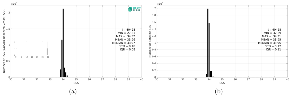
Figure 3: Histograms of SSS from TSG (GOSUD-Research-vessel) (a) and ISAS v7 - Monthly (Ifremer-LOPS-CMEMS) (b) considering all match-up pairs per bins of 0.1 over the Southern Ocean Pi-MEP region and for the full satellite product period.
