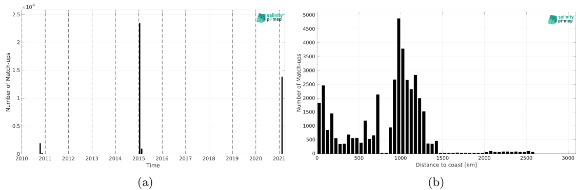
Figure 2: Number of match-ups between TSG (GOSUD-Research-vessel) and ISAS v7 - Monthly (Ifremer-LOPS-CMEMS) SSS as a function of time (a) and as function of the distance to coast (b) over the Southern Ocean Pi-MEP region and for the full satellite product period.
