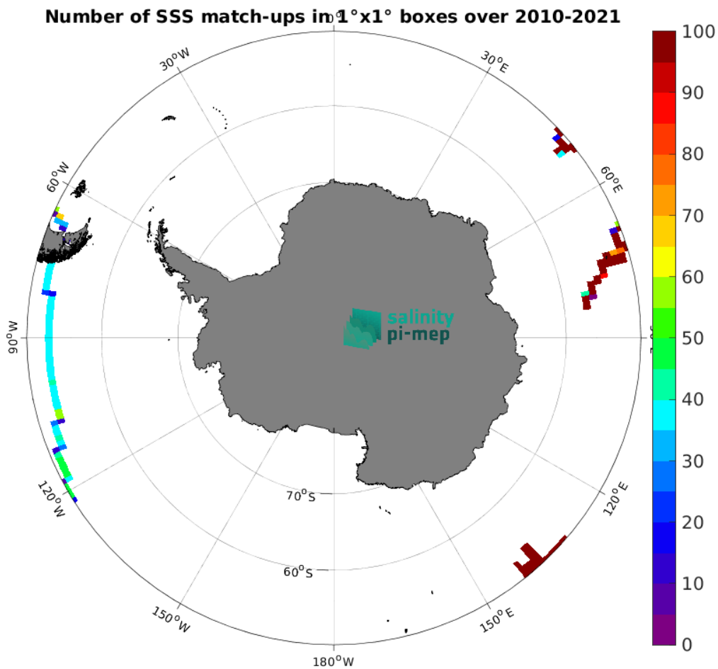
Figure 5: Number of SSS match-ups between TSG (GOSUD-Research-vessel) SSS and the ISAS v7 - Monthly (Ifremer-LOPS-CMEMS) SSS product for the Southern Ocean Pi-MEP region over 1^\circ \times 1^\circ boxes and for the full satellite product period.
