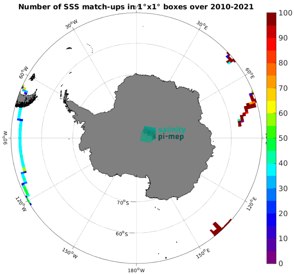
Figure 5: Number of SSS match-ups between TSG (GOSUD-Research-vessel) SSS and the ISAS SSS product for the Southern Ocean Pi-MEP region over 1^\circ \times 1^\circ boxes and for the full satellite product period.
