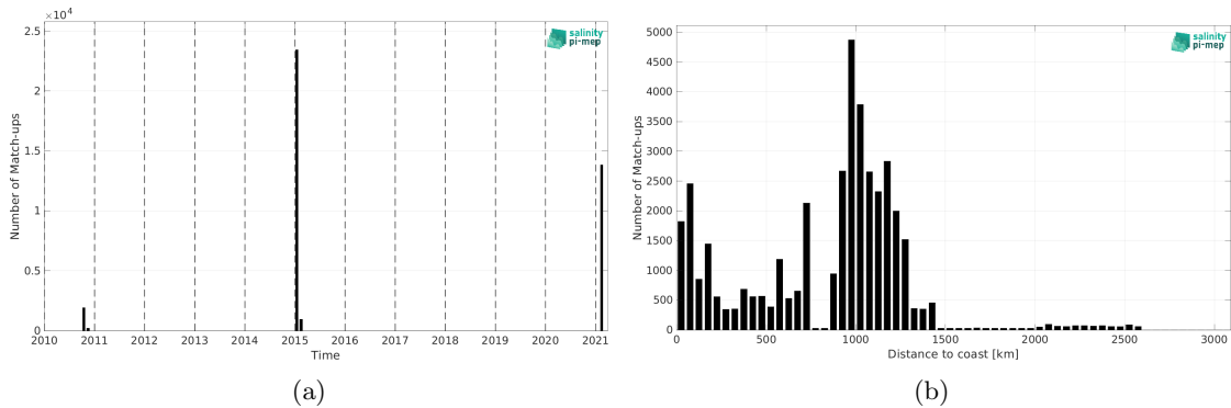
Figure 2: Number of match-ups between TSG (GOSUD-Research-vessel) and ISAS SSS as a function of time (a) and as function of the distance to coast (b) over the Southern Ocean Pi-MEP region and for the full satellite product period.
