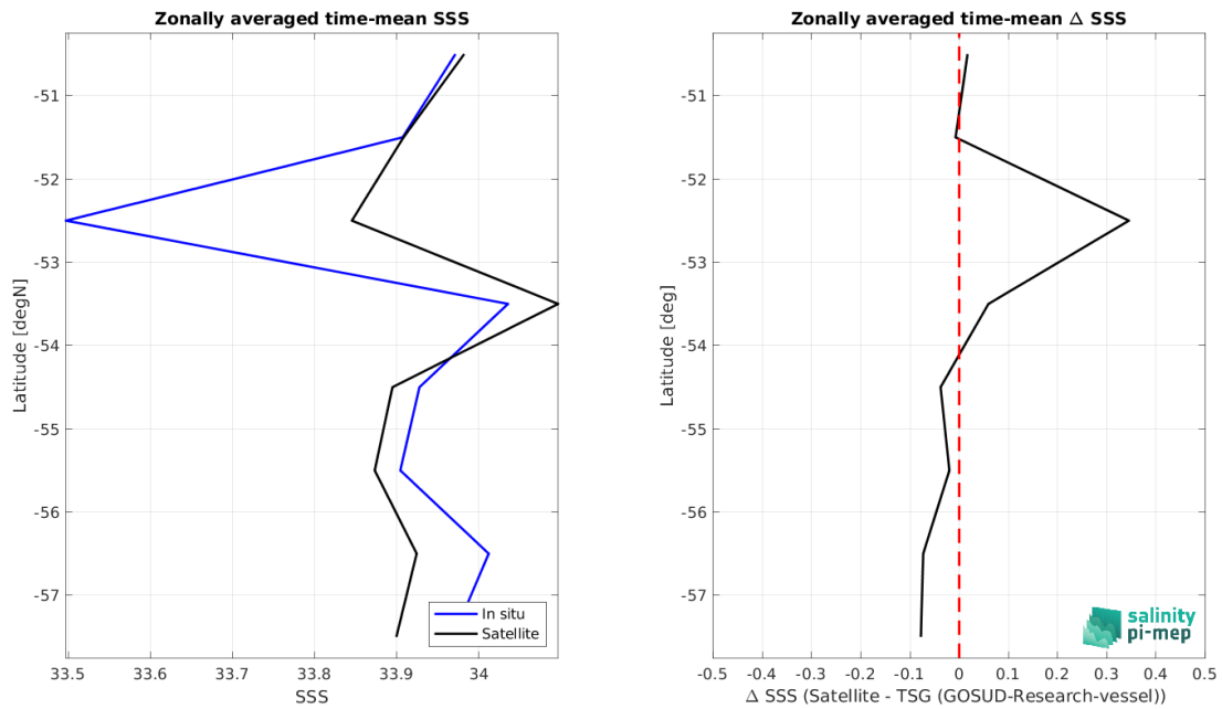
Figure 9: Left panel: Zonal mean SSS from ISAS satellite product (black) and from TSG (GOSUD-Research-vessel) (blue). Right panel: Zonal mean of \Delta SSS (Satellite - TSG (GOSUD-Research-vessel)) for all the collected Pi-MEP match-up pairs estimated over the full satellite product period.
