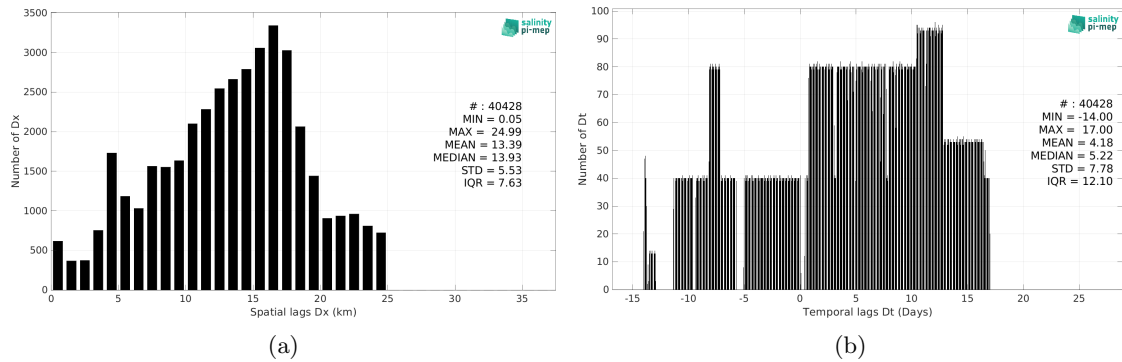
Figure 6: Histograms of the spatial (a) and temporal (b) lags between the location/time of the TSG (GOSUD-Research-vessel) measurement and the date of the corresponding ISAS SSS pixel.
