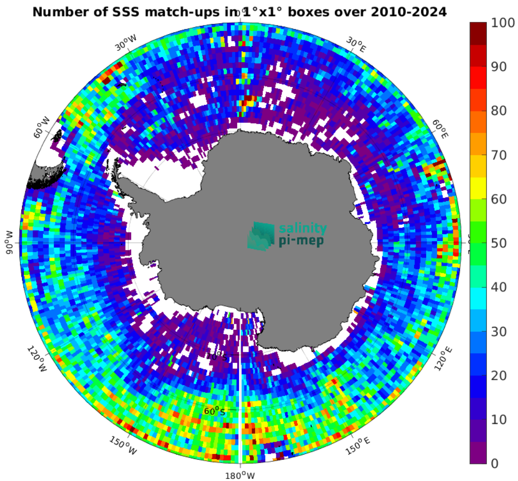
Figure 5: Number of SSS match-ups between Argo SSS and the ISAS v7 - Monthly (Ifremer-LOPS-CMEMS) SSS product for the Southern Ocean Pi-MEP region over 1^\circ \times 1^\circ boxes and for the full satellite product period.
