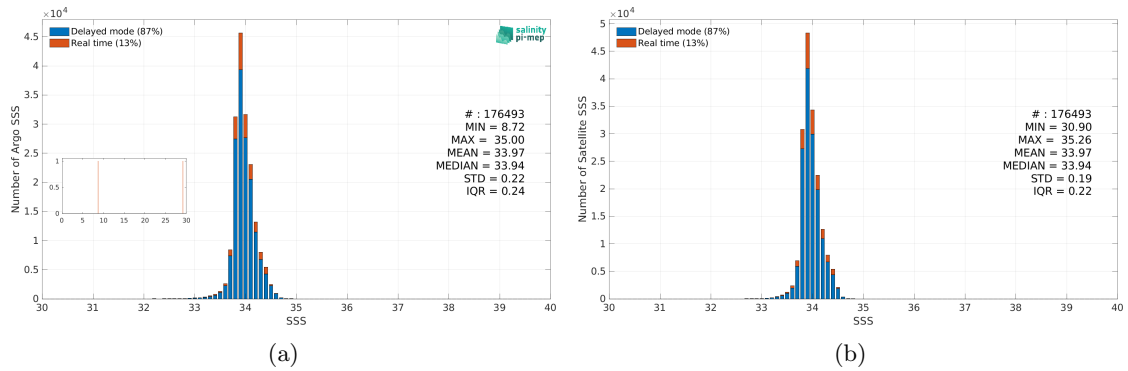
Figure 3: Histograms of SSS from Argo (a) and ISAS v7 - Monthly (Ifremer-LOPS-CMEMS) (b) considering all match-up pairs per bins of 0.1 over the Southern Ocean Pi-MEP region and for the full satellite product period.
