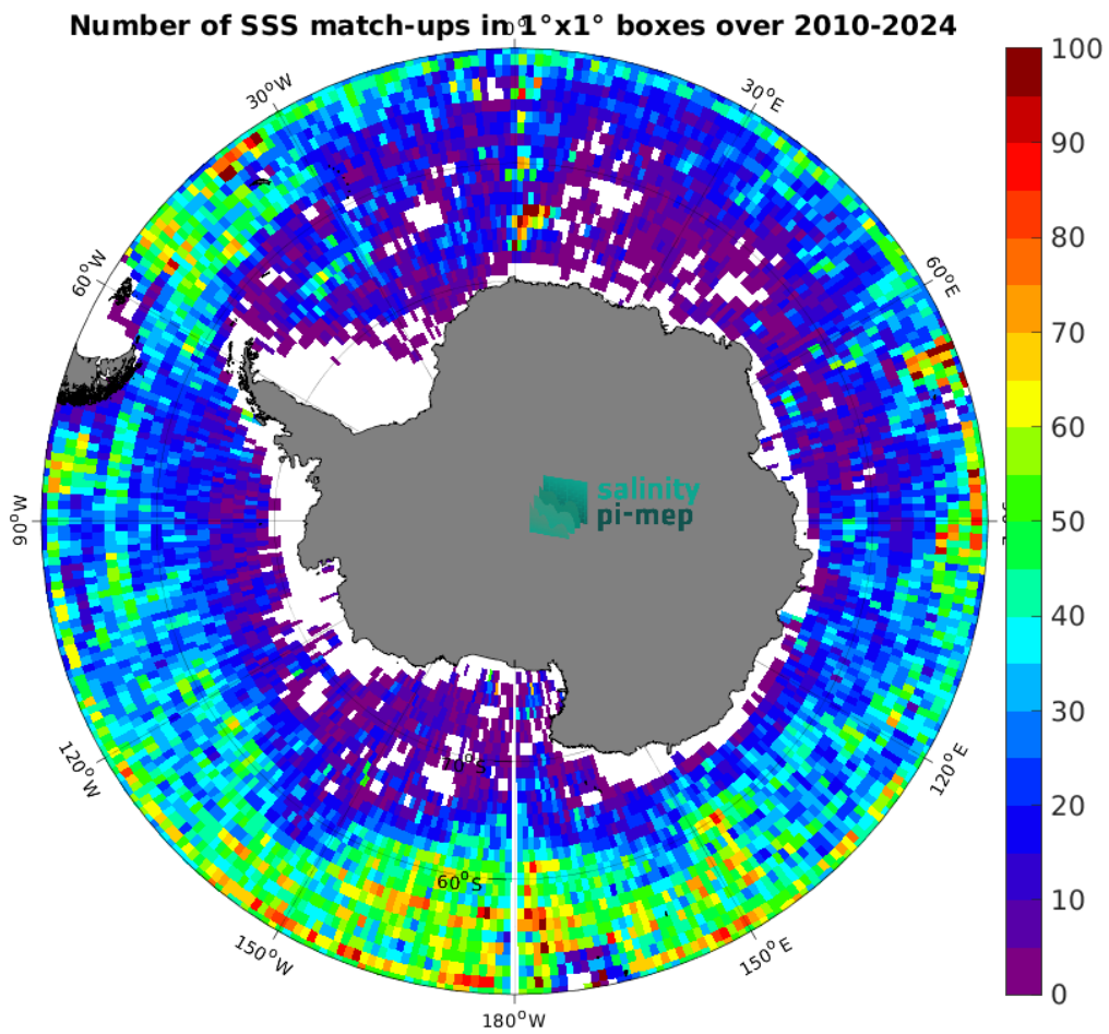
Figure 5: Number of SSS match-ups between Argo SSS and the ISAS SSS product for the Southern Ocean Pi-MEP region over 1^\circ \times 1^\circ boxes and for the full satellite product period.
