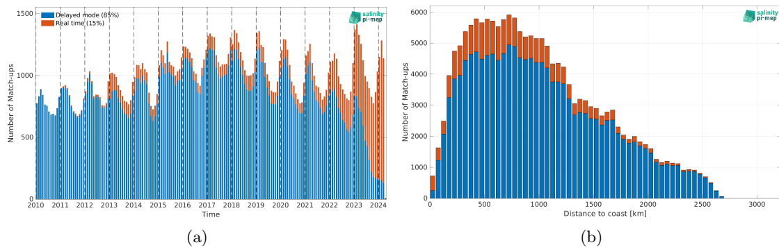
Figure 2: Number of match-ups between Argo and ISAS SSS as a function of time (a) and as function of the distance to coast (b) over the Southern Ocean Pi-MEP region and for the full satellite product period.
