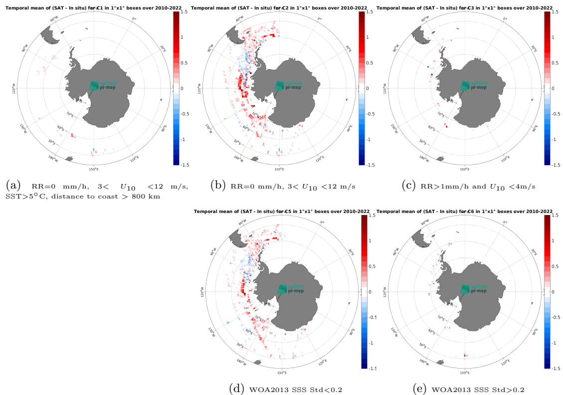
Figure 14: Temporal mean gridded over spatial boxes of size 1^\circ \times 1^\circ of \Delta\text{SSS} (CCI SSS L4 POLAR SH Merged-OI v4.41 - 7-day running (ESA) - TSG (SAMOS)) for 5 different subdatasets corresponding to:RR=0 mm/h, 3 < U_{10} < 12 m/s, SST>5°C, distance to coast > 800 km (a), RR=0 mm/h, 3 < U_{10} < 12 m/s (b), RR>1mm/h and U_{10} < 4 m/s (c), WOA2013 SSS Std<0.2 (d), WOA2013 SSS Std>0.2 (e).
