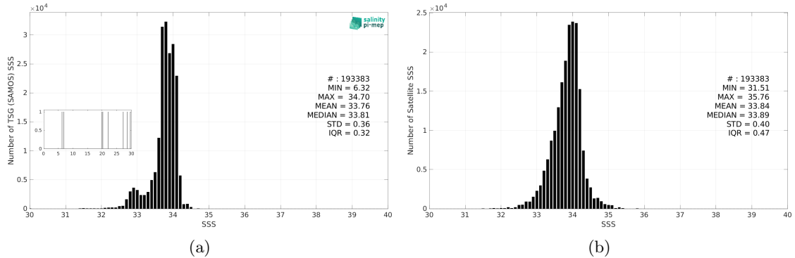
Figure 3: Histograms of SSS from TSG (SAMOS) (a) and CCI SSS L4 POLAR SH Merged-OI v4.41 - 7-day running (ESA) (b) considering all match-up pairs per bins of 0.1 over the Southern Ocean Pi-MEP region and for the full satellite product period.
