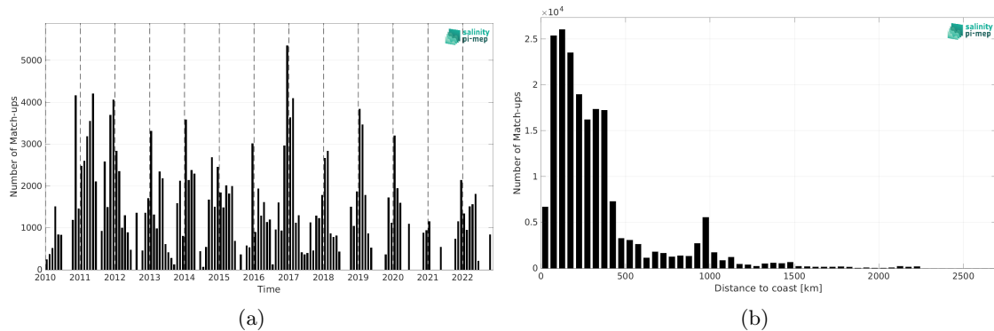
Figure 2: Number of match-ups between TSG (SAMOS) and CCI SSS L4 POLAR SH Merged-OI v4.41 - 7-day running (ESA) SSS as a function of time (a) and as function of the distance to coast (b) over the Southern Ocean Pi-MEP region and for the full satellite product period.
