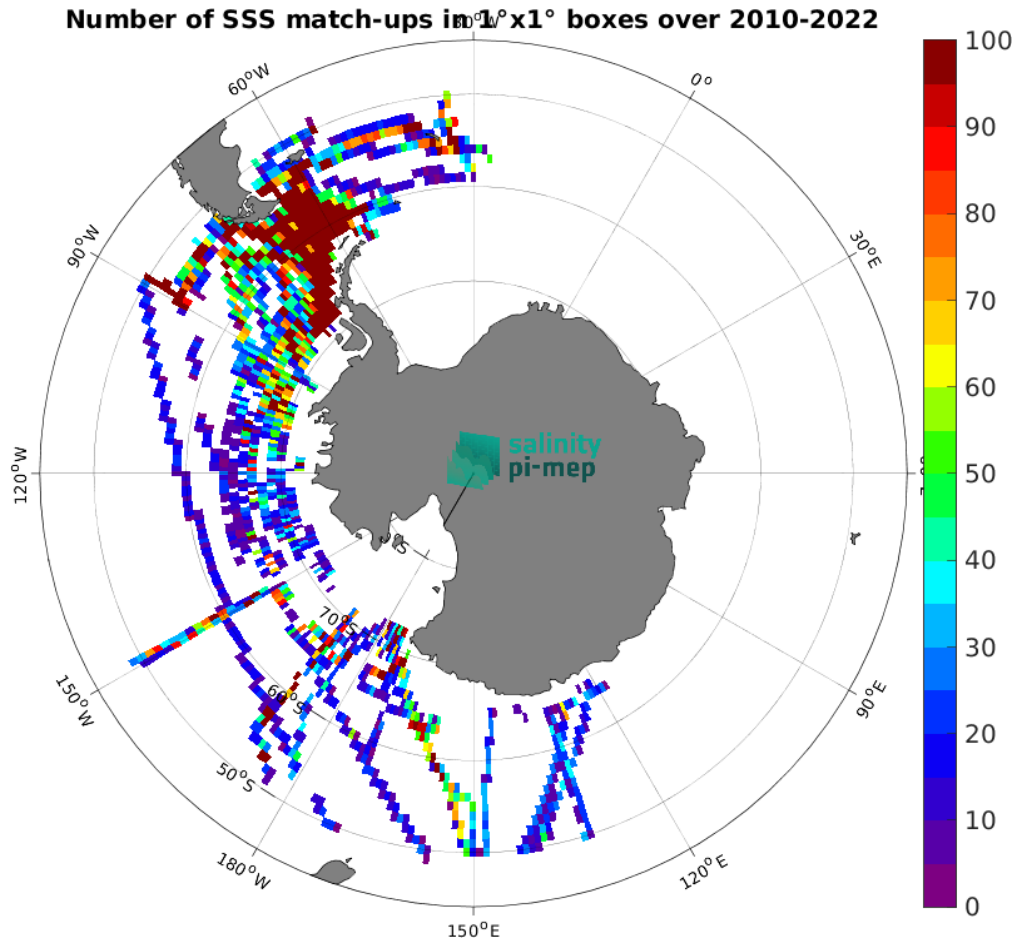
Figure 5: Number of SSS match-ups between TSG (SAMOS) SSS and the CCI SSS L4 POLAR SH Merged-OI v4.41 - 7-day running (ESA) SSS product for the Southern Ocean Pi-MEP region over 1^\circ \times 1^\circ boxes and for the full satellite product period.
