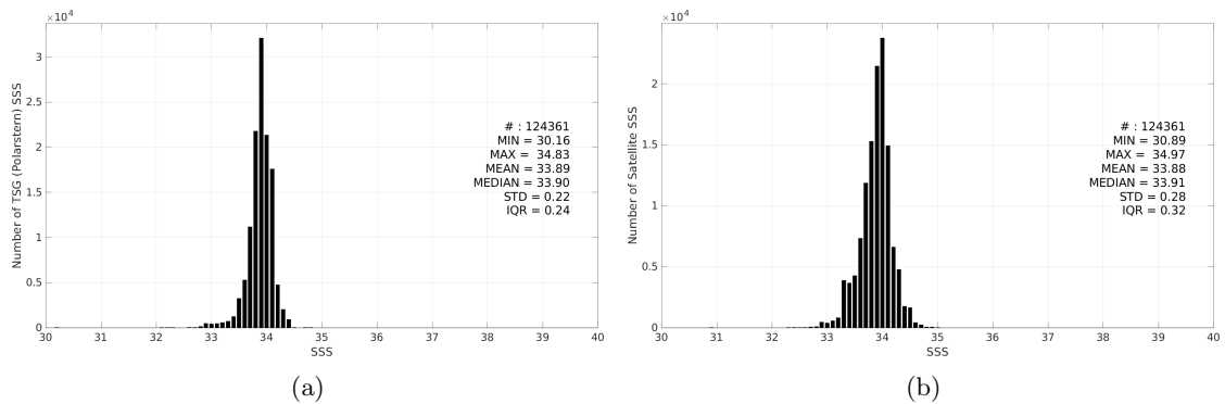
Figure 3: Histograms of SSS from TSG (Polarstern) (a) and CCI SSS L4 POLAR SH Merged-OI v4.41 - 7-day running (ESA) (b) considering all match-up pairs per bins of 0.1 over the Southern Ocean Pi-MEP region and for the full satellite product period.
