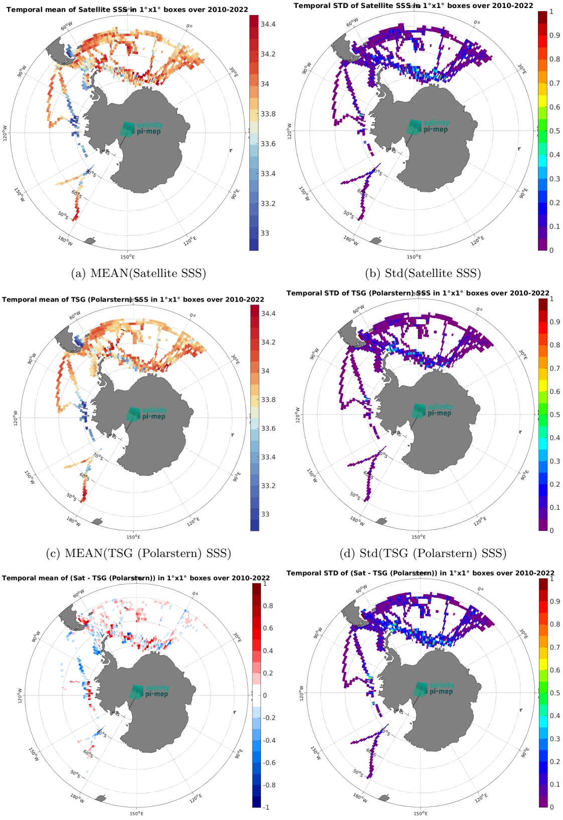
Figure 7: Temporal mean (left) and Std (right) of SSS from CCI SSS L4 POLAR SH Merged-OI v4.41 - 7-day running (ESA) (top), TSG (Polarstern) (middle), and of \Delta SSS (Satellite - TSG (Polarstern)). Only match-up pairs are used to generate these maps.
