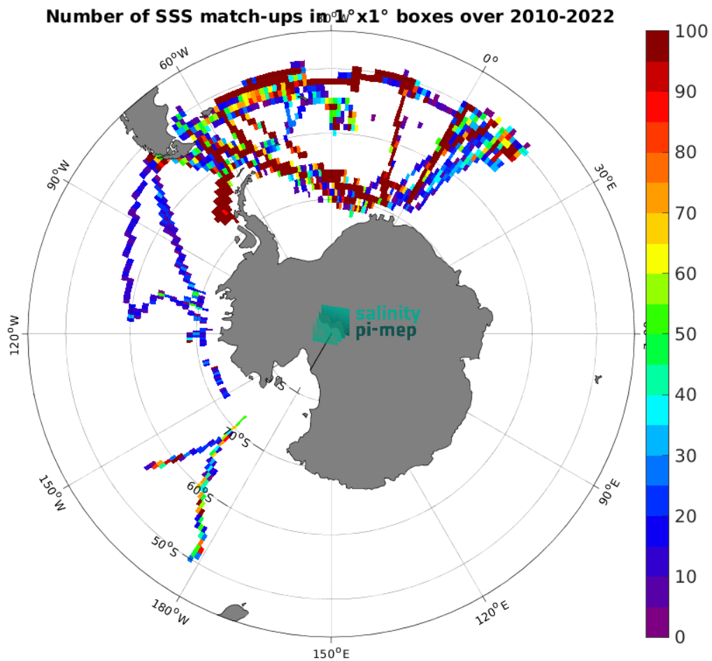
Figure 5: Number of SSS match-ups between TSG (Polarstern) SSS and the CCI SSS L4 POLAR SH Merged-OI v4.41 - 7-day running (ESA) SSS product for the Southern Ocean Pi-MEP region over 1^\circ \times 1^\circ boxes and for the full satellite product period.
