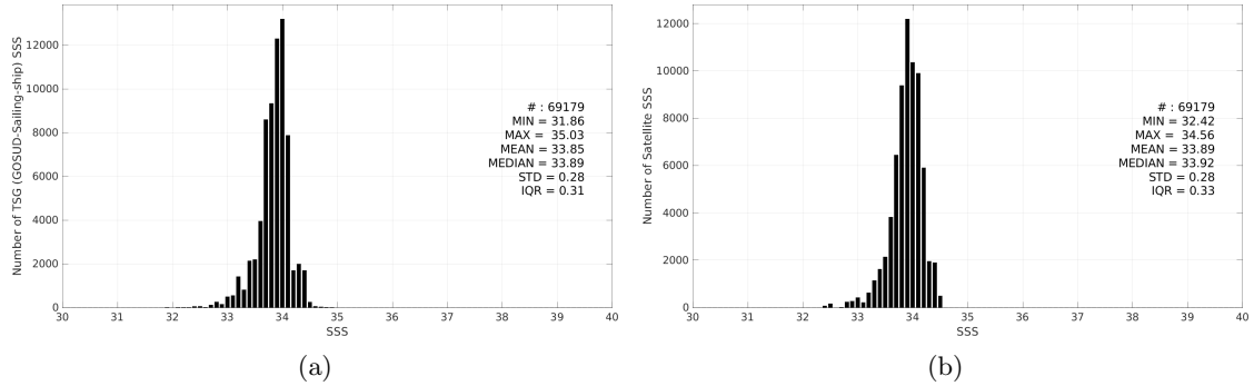
Figure 3: Histograms of SSS from TSG (GOSUD-Sailing-ship) (a) and CCI SSS L4 POLAR SH Merged-OI v4.41 - 7-day running (ESA) (b) considering all match-up pairs per bins of 0.1 over the Southern Ocean Pi-MEP region and for the full satellite product period.
