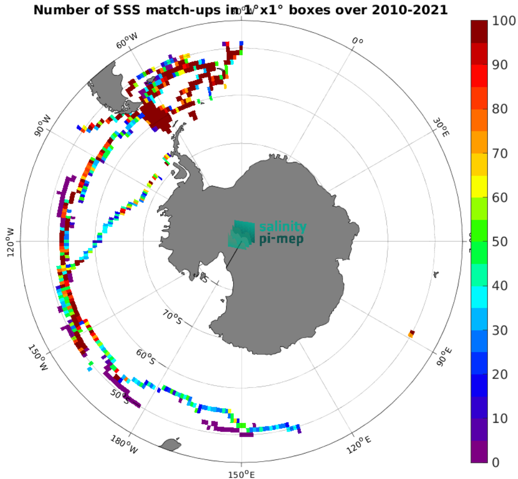
Figure 5: Number of SSS match-ups between TSG (GOSUD-Sailing-ship) SSS and the CCI SSS L4 POLAR SH Merged-OI v4.41 - 7-day running (ESA) SSS product for the Southern Ocean Pi-MEP region over 1^\circ \times 1^\circ boxes and for the full satellite product period.
