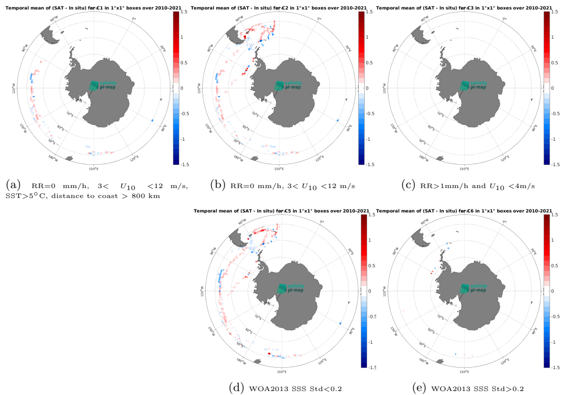
Figure 14: Temporal mean gridded over spatial boxes of size 1^\circ \times 1^\circ of \Delta\text{SSS} (CCI SSS L4 POLAR SH Merged-OI v4.41 - 7-day running (ESA) - TSG (GOSUD-Sailing-ship)) for 5 different subdatasets corresponding to:RR=0 mm/h, 3 < U_{10} < 12 m/s, SST>5°C, distance to coast > 800 km (a), RR=0 mm/h, 3 < U_{10} < 12 m/s (b), RR>1mm/h and U_{10} < 4 m/s (c), WOA2013 SSS Std<0.2 (d), WOA2013 SSS Std>0.2 (e).
