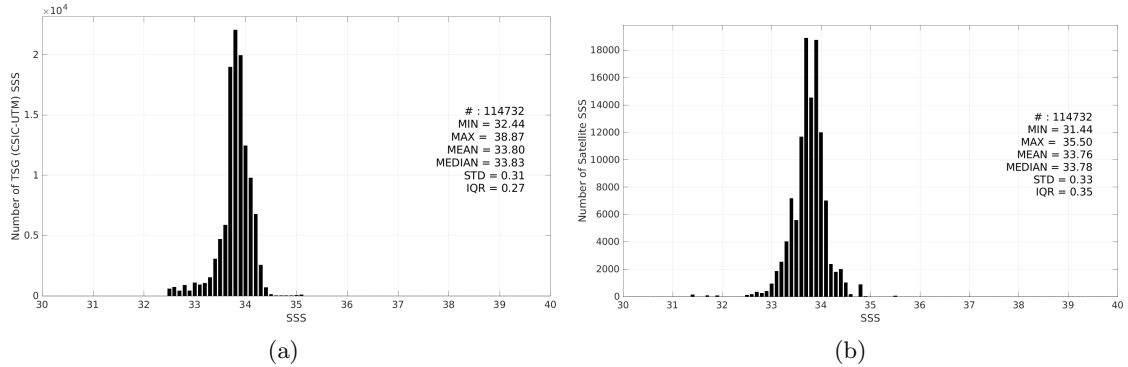
Figure 3: Histograms of SSS from TSG (CSIC-UTM) (a) and CCI SSS L4 POLAR SH Merged-OI v4.41 - 7-day running (ESA) (b) considering all match-up pairs per bins of 0.1 over the Southern Ocean Pi-MEP region and for the full satellite product period.
