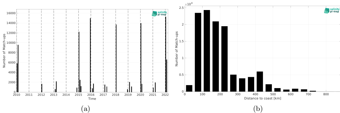
Figure 2: Number of match-ups between TSG (CSIC-UTM) and CCI SSS L4 POLAR SH Merged-OI v4.41 - 7-day running (ESA) SSS as a function of time (a) and as function of the distance to coast (b) over the Southern Ocean Pi-MEP region and for the full satellite product period.
