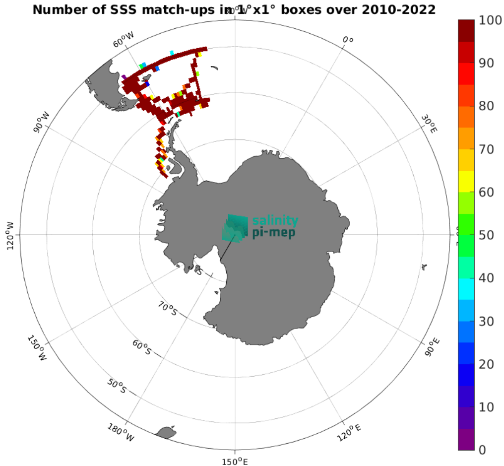
Figure 5: Number of SSS match-ups between TSG (CSIC-UTM) SSS and the CCI SSS L4 POLAR SH Merged-OI v4.41 - 7-day running (ESA) SSS product for the Southern Ocean Pi-MEP region over 1^\circ \times 1^\circ boxes and for the full satellite product period.
