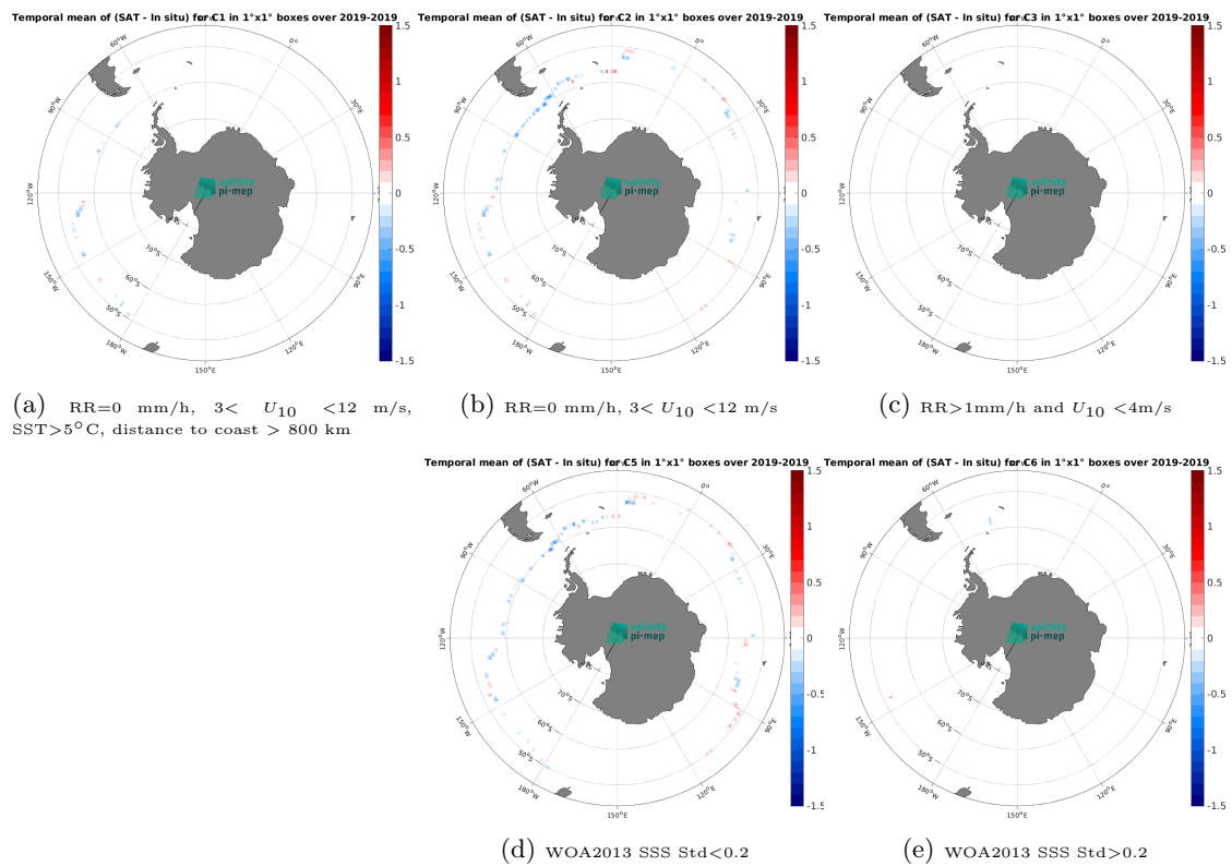
Figure 14: Temporal mean gridded over spatial boxes of size 1^\circ \times 1^\circ of \Delta\text{SSS} (CCI SSS L4 POLAR SH Merged-OI v4.41 - 7-day running (ESA) - Saildrone) for 5 different subdatasets corresponding to:RR=0 mm/h, 3 < U_{10} < 12 m/s, SST>5°C, distance to coast > 800 km (a), RR=0 mm/h, 3 < U_{10} < 12 m/s (b), RR>1mm/h and U_{10} < 4 m/s (c), WOA2013 SSS Std<0.2 (d), WOA2013 SSS Std>0.2 (e).
