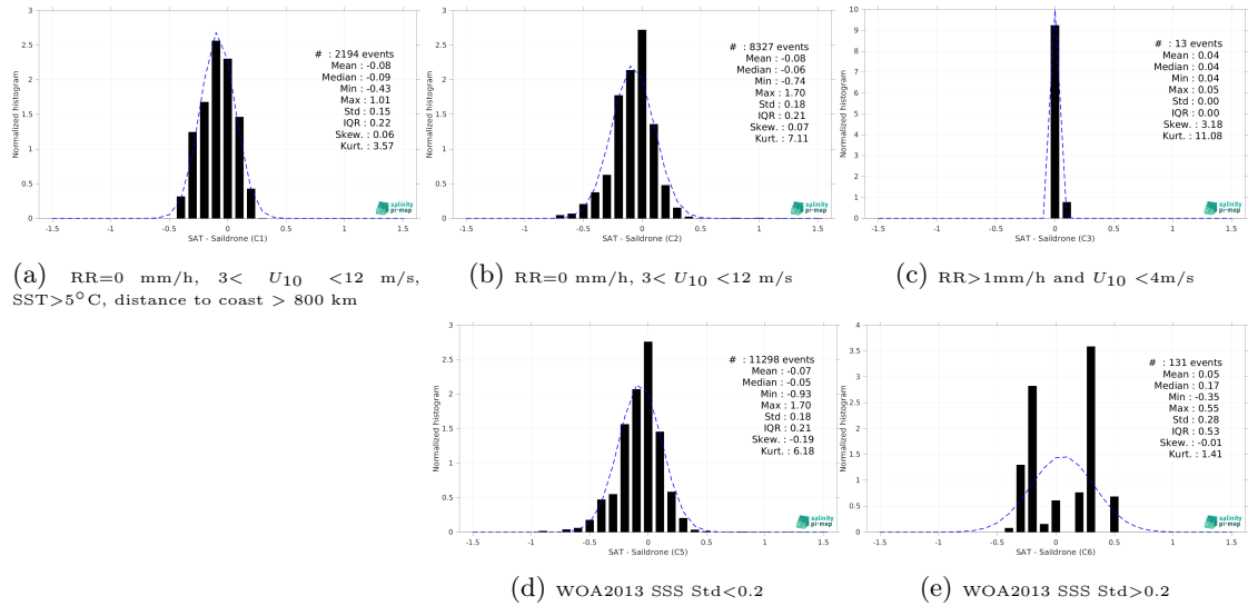
Figure 15: Normalized histogram of \Delta SSS (CCI SSS L4 POLAR SH Merged-OI v4.41 - 7-day running (ESA) - Saildrone) for 5 different subdatasets corresponding to: RR=0 mm/h, 3 < U_{10} < 12 m/s, SST > 5°C, distance to coast > 800 km (a), RR=0 mm/h, 3 < U_{10} < 12 m/s (b), RR > 1mm/h and U_{10} < 4 m/s (c), WOA2013 SSS Std < 0.2 (d), WOA2013 SSS Std > 0.2 (e).
