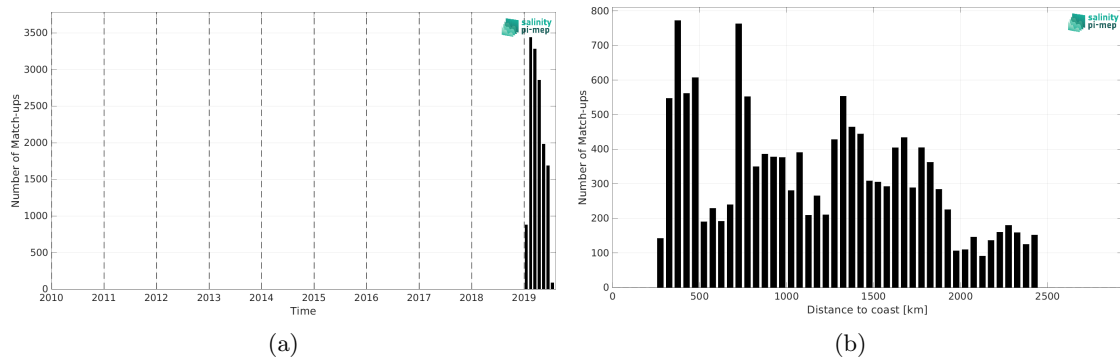
Figure 2: Number of match-ups between Saildrone and CCI SSS L4 POLAR SH Merged-OI v4.41 - 7-day running (ESA) SSS as a function of time (a) and as function of the distance to coast (b) over the Southern Ocean Pi-MEP region and for the full satellite product period.
