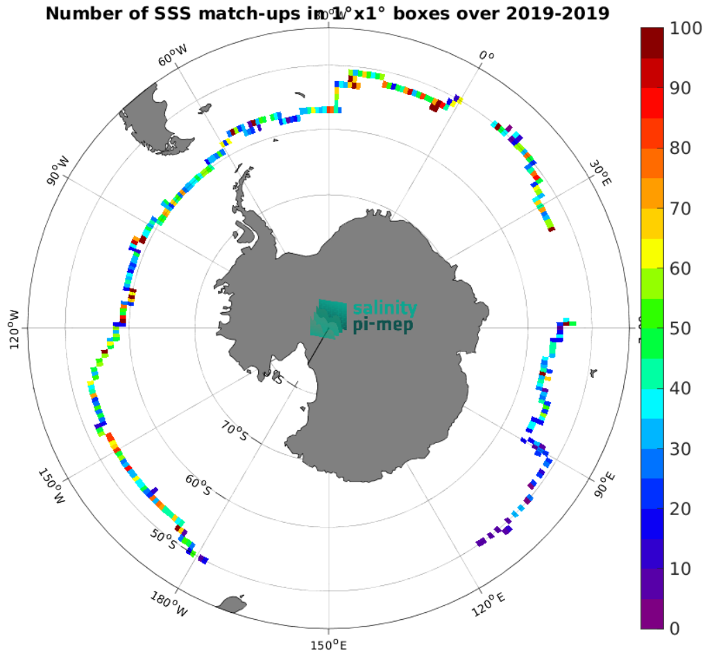
Figure 5: Number of SSS match-ups between Saildrone SSS and the CCI SSS L4 POLAR SH Merged-OI v4.41 - 7-day running (ESA) SSS product for the Southern Ocean Pi-MEP region over 1^\circ \times 1^\circ boxes and for the full satellite product period.
