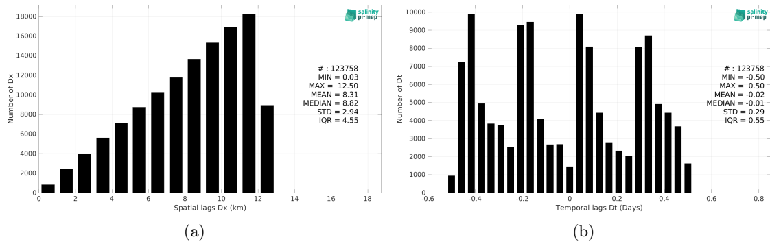
Figure 6: Histograms of the spatial (a) and temporal (b) lags between the location/time of the Marine mammals measurement and the date of the corresponding CCI SSS L4 POLAR SH Merged-OI v4.41 - 7-day running (ESA) SSS pixel.
