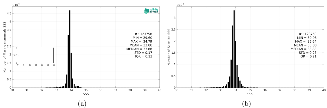
Figure 3: Histograms of SSS from Marine mammals (a) and CCI SSS L4 POLAR SH Merged-OI v4.41 - 7-day running (ESA) (b) considering all match-up pairs per bins of 0.1 over the Southern Ocean Pi-MEP region and for the full satellite product period.
