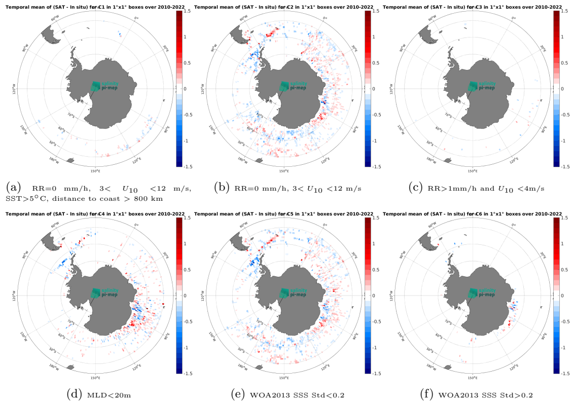
Figure 14: Temporal mean gridded over spatial boxes of size 1^\circ \times 1^\circ of \Delta\text{SSS} (CCI SSS L4 POLAR SH Merged-OI v4.41 - 7-day running (ESA) - Marine mammals) for 6 different subdatasets corresponding to:RR=0 mm/h, 3 < U_{10} < 12 m/s, SST>5°C, distance to coast > 800 km (a), RR=0 mm/h, 3 < U_{10} < 12 m/s (b), RR>1mm/h and U_{10} < 4 m/s (c),MLD<20m (d),WOA2013 SSS Std<0.2 (e),WOA2013 SSS Std>0.2 (f).
