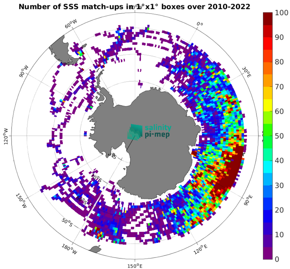
Figure 5: Number of SSS match-ups between Marine mammals SSS and the CCI SSS L4 POLAR SH Merged-OI v4.41 - 7-day running (ESA) SSS product for the Southern Ocean Pi-MEP region over 1^\circ \times 1^\circ boxes and for the full satellite product period.
