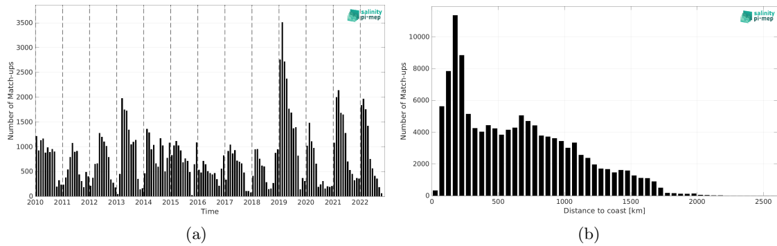
Figure 2: Number of match-ups between Marine mammals and CCI SSS L4 POLAR SH Merged-OI v4.41 - 7-day running (ESA) SSS as a function of time (a) and as function of the distance to coast (b) over the Southern Ocean Pi-MEP region and for the full satellite product period.
