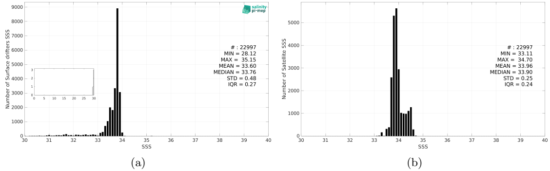
Figure 3: Histograms of SSS from Surface drifters (a) and CCI SSS L4 POLAR SH Merged-OI v4.41 - 7-day running (ESA) (b) considering all match-up pairs per bins of 0.1 over the Southern Ocean Pi-MEP region and for the full satellite product period.
