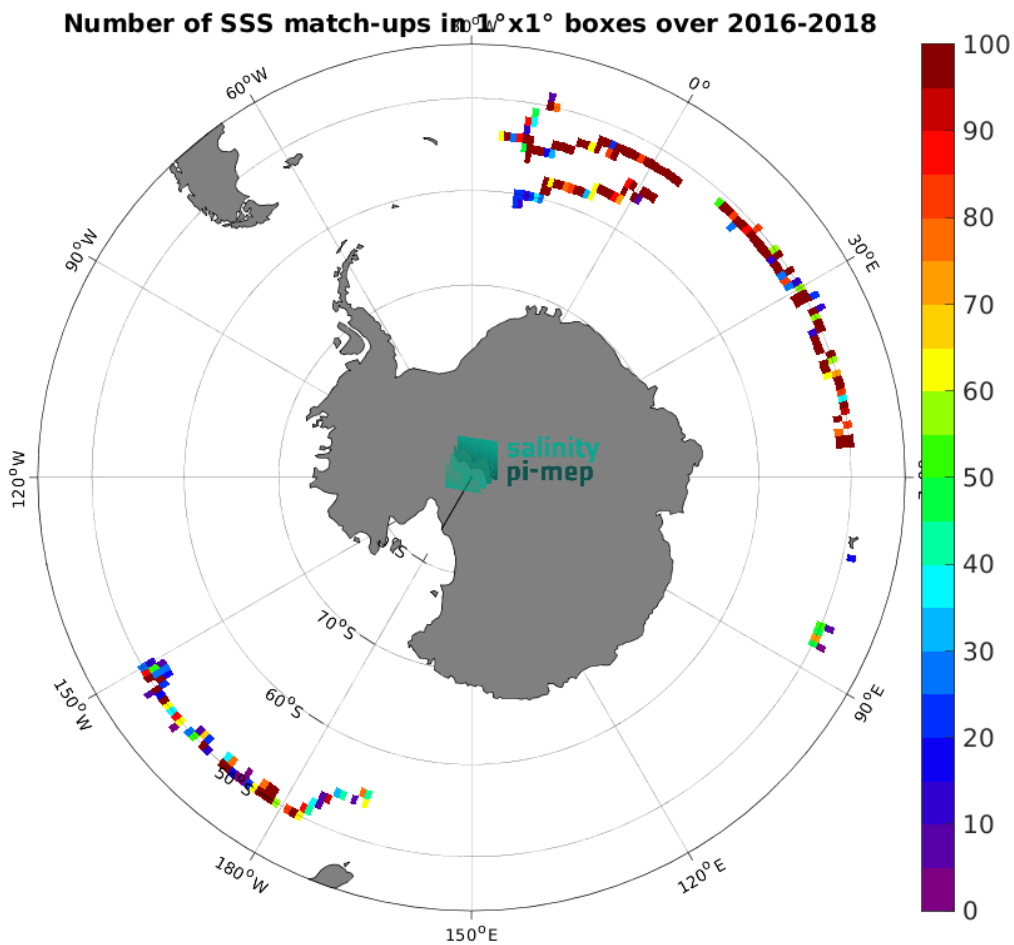
Figure 4: Number of SSS match-ups between Surface drifters SSS and the CCI SSS L4 POLAR SH Merged-OI v4.41 - 7-day running (ESA) SSS product for the Southern Ocean Pi-MEP region over 1^\circ \times 1^\circ boxes and for the full satellite product period.
