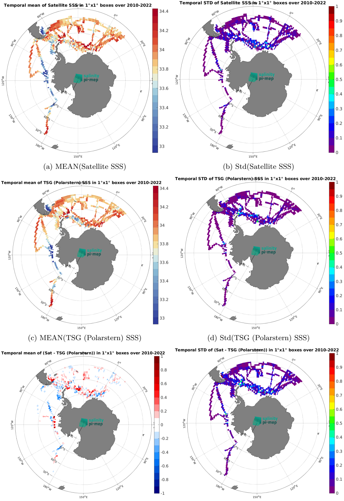
Figure 7: Temporal mean (left) and Std (right) of SSS from CCI SSS L4 POLAR SH Merged-OI v4.41 - 30-day running (ESA) (top), TSG (Polarstern) (middle), and of \Delta SSS (Satellite - TSG (Polarstern)). Only match-up pairs are used to generate these maps.
