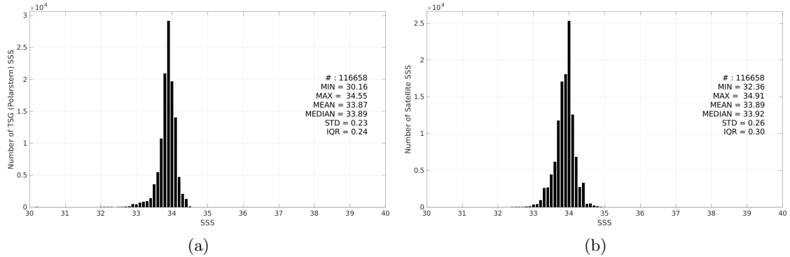
Figure 3: Histograms of SSS from TSG (Polarstern) (a) and CCI SSS L4 POLAR SH Merged-OI v4.41 - 30-day running (ESA) (b) considering all match-up pairs per bins of 0.1 over the Southern Ocean Pi-MEP region and for the full satellite product period.
