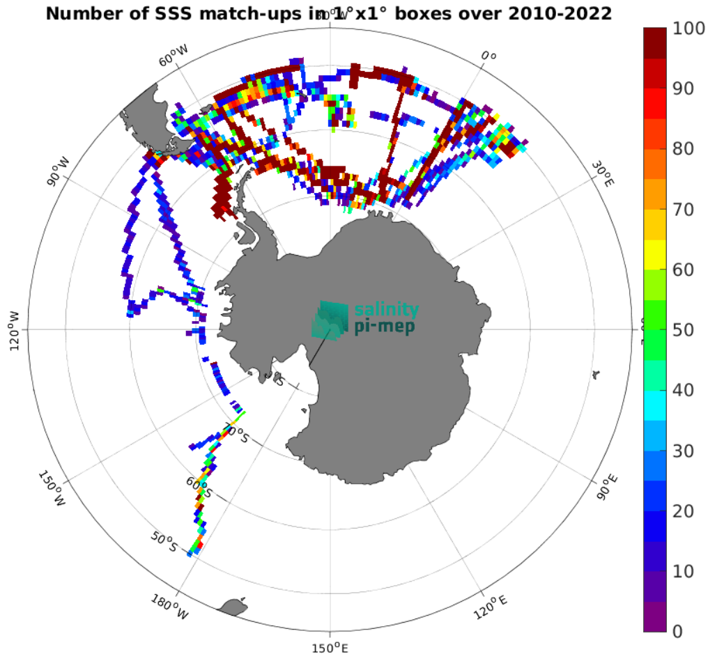
Figure 5: Number of SSS match-ups between TSG (Polarstern) SSS and the CCI SSS L4 POLAR SH Merged-OI v4.41 - 30-day running (ESA) SSS product for the Southern Ocean Pi-MEP region over 1^\circ \times 1^\circ boxes and for the full satellite product period.
