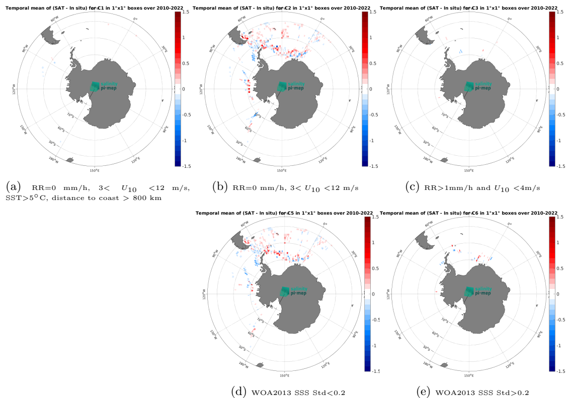
Figure 14: Temporal mean gridded over spatial boxes of size 1^\circ \times 1^\circ of \Delta\text{SSS} (CCI SSS L4 POLAR SH Merged-OI v4.41 - 30-day running (ESA) - TSG (Polarstern)) for 5 different subdatasets corresponding to:RR=0 mm/h, 3 < U_{10} < 12 m/s, SST>5°C, distance to coast > 800 km (a), RR=0 mm/h, 3 < U_{10} < 12 m/s (b), RR>1mm/h and U_{10} < 4 m/s (c), WOA2013 SSS Std<0.2 (d), WOA2013 SSS Std>0.2 (e).
