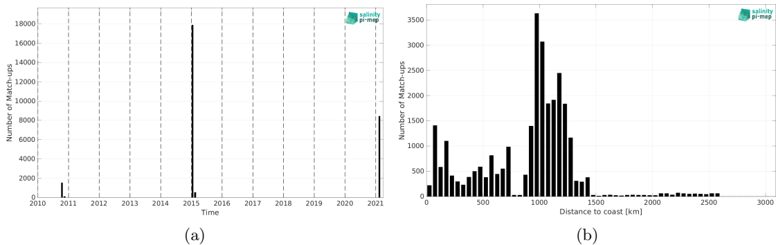
Figure 2: Number of match-ups between TSG (GOSUD-Research-vessel) and CCI SSS L4 POLAR SH Merged-OI v4.41 - 30-day running (ESA) SSS as a function of time (a) and as function of the distance to coast (b) over the Southern Ocean Pi-MEP region and for the full satellite product period.
