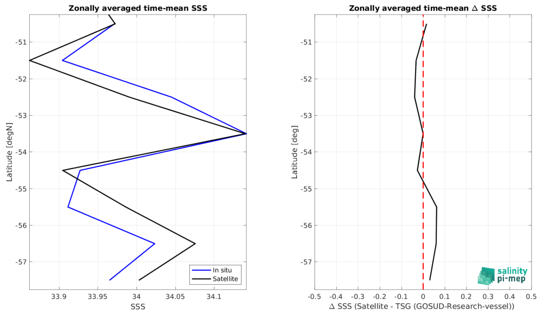
Figure 9: Left panel: Zonal mean SSS from CCI SSS L4 POLAR SH Merged-OI v4.41 - 30-day running (ESA) satellite product (black) and from TSG (GOSUD-Research-vessel) (blue). Right panel: Zonal mean of \Delta SSS (Satellite - TSG (GOSUD-Research-vessel)) for all the collected Pi-MEP match-up pairs estimated over the full satellite product period.
