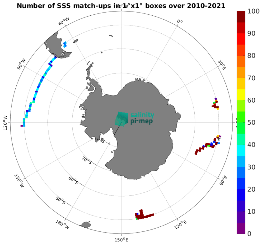
Figure 5: Number of SSS match-ups between TSG (GOSUD-Research-vessel) SSS and the CCI SSS L4 POLAR SH Merged-OI v4.41 - 30-day running (ESA) SSS product for the Southern Ocean Pi-MEP region over 1^\circ \times 1^\circ boxes and for the full satellite product period.
