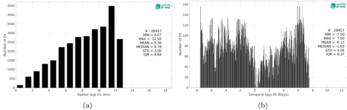
Figure 6: Histograms of the spatial (a) and temporal (b) lags between the location/time of the TSG (GOSUD-Research-vessel) measurement and the date of the corresponding CCI SSS L4 POLAR SH Merged-OI v4.41 - 30-day running (ESA) SSS pixel.
