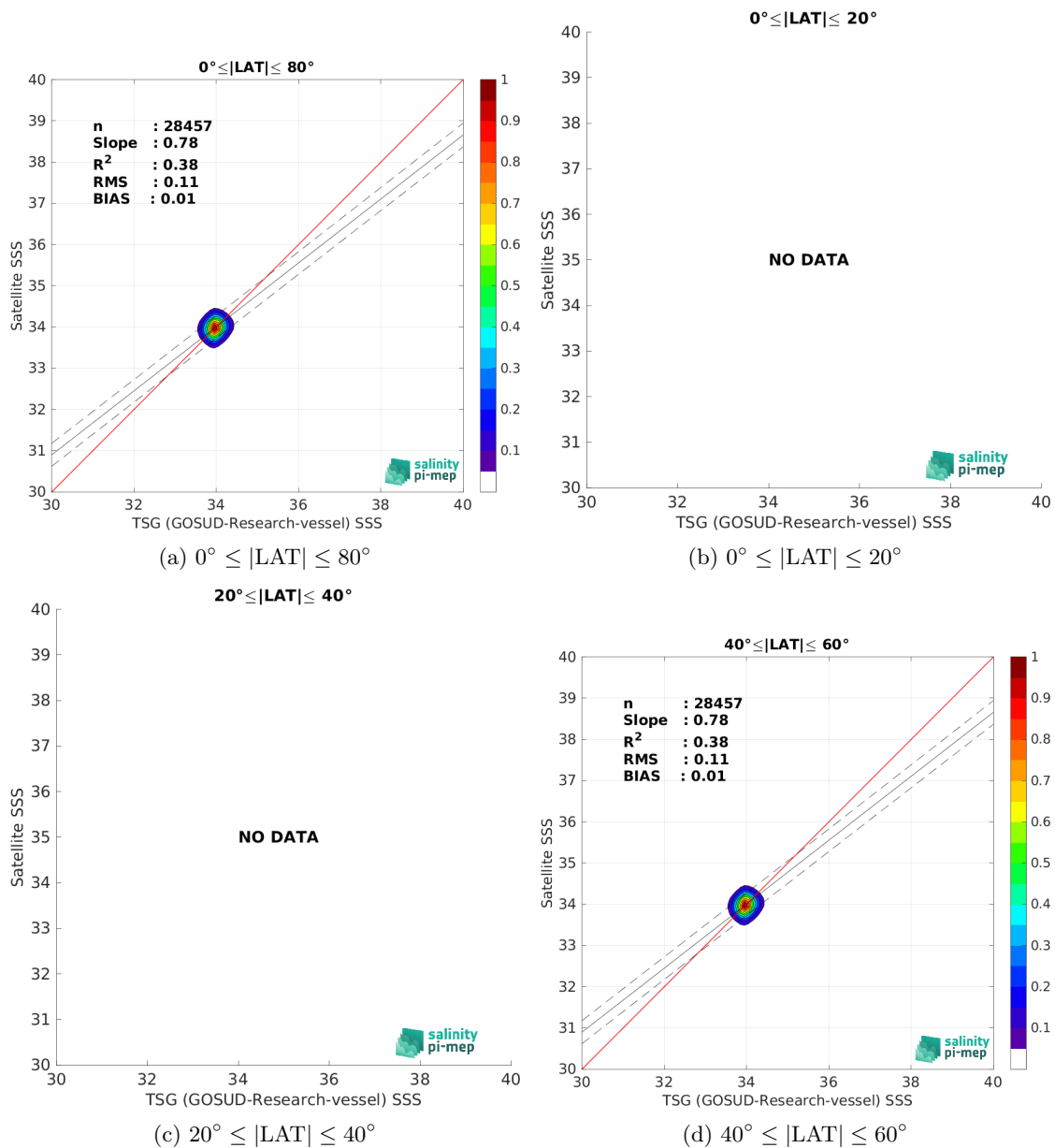
Figure 10: Contour maps of the concentration of CCI SSS L4 POLAR SH Merged-OI v4.41 - 30-day running (ESA) SSS (y-axis) versus TSG (GOSUD-Research-vessel) SSS (x-axis) at match-up pairs for different latitude bands. For each plot, the red line shows x=y . The black thin and dashed lines indicate a linear fit through the data cloud and the \pm 95\% confidence levels, respectively. The number match-up pairs n , the slope and R^2 coefficient of the linear fit, the root mean square (RMS) and the mean bias between satellite and in situ data are indicated for each latitude band in each plots.
