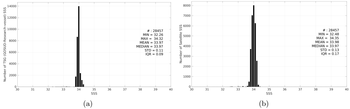
Figure 3: Histograms of SSS from TSG (GOSUD-Research-vessel) (a) and CCI SSS L4 POLAR SH Merged-OI v4.41 - 30-day running (ESA) (b) considering all match-up pairs per bins of 0.1 over the Southern Ocean Pi-MEP region and for the full satellite product period.
