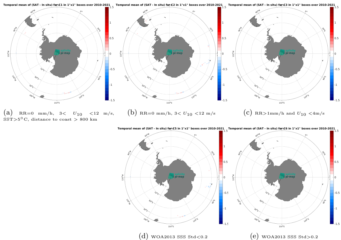
Figure 14: Temporal mean gridded over spatial boxes of size 1^\circ \times 1^\circ of \Delta SSS (CCI SSS L4 POLAR SH Merged-OI v4.41 - 30-day running (ESA) - TSG (GOSUD-Research-vessel)) for 5 different subdatasets corresponding to:RR=0 mm/h, 3 < U_{10} < 12 m/s, SST >5^\circ C, distance to coast > 800 km (a), RR=0 mm/h, 3 < U_{10} < 12 m/s (b), RR >1 mm/h and U_{10} < 4 m/s (c), WOA2013 SSS Std <0.2 (d), WOA2013 SSS Std >0.2 (e).
