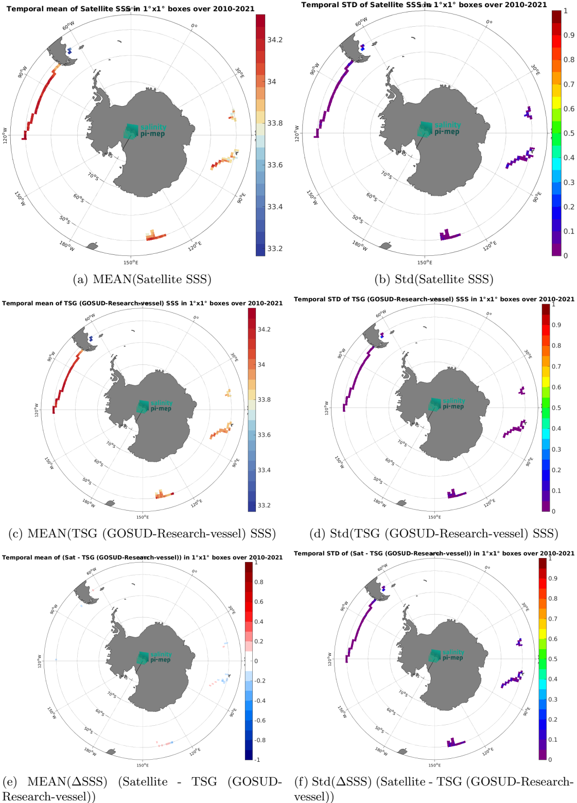
Figure 7: Temporal mean (left) and Std (right) of SSS from CCI SSS L4 POLAR SH Merged-OI v4.41 - 30-day running (ESA) (top), TSG (GOSUD-Research-vessel) (middle), and of \Delta SSS (Satellite - TSG (GOSUD-Research-vessel)). Only match-up pairs are used to generate these maps.
