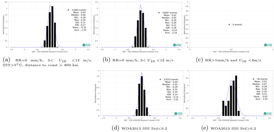
Figure 15: Normalized histogram of \Delta SSS (CCI SSS L4 POLAR SH Merged-OI v4.41 - 30-day running (ESA) - TSG (GOSUD-Research-vessel)) for 5 different subdatasets corresponding to: RR=0 mm/h, 3 < U_{10} < 12 m/s, SST>5°C, distance to coast > 800 km (a), RR=0 mm/h, 3 < U_{10} < 12 m/s (b), RR>1mm/h and U_{10} < 4 m/s (c), WOA2013 SSS Std<0.2 (d), WOA2013 SSS Std>0.2 (e).
