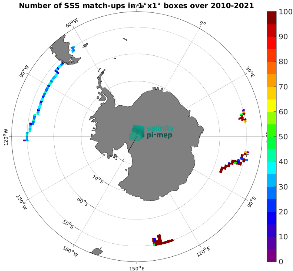
Figure 5: Number of SSS match-ups between TSG (GOSUD-Research-vessel) SSS and the CCI SSS L4 POLAR SH Merged-OI v4.41 - 30-day running (ESA) SSS product for the Southern Ocean Pi-MEP region over 1^\circ \times 1^\circ boxes and for the full satellite product period.
