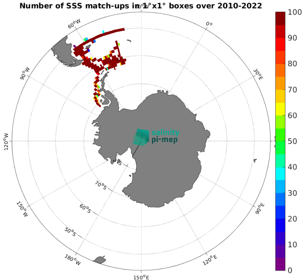
Figure 5: Number of SSS match-ups between TSG (CSIC-UTM) SSS and the CCI SSS L4 POLAR SH Merged-OI v4.41 - 30-day running (ESA) SSS product for the Southern Ocean Pi-MEP region over 1^\circ \times 1^\circ boxes and for the full satellite product period.
