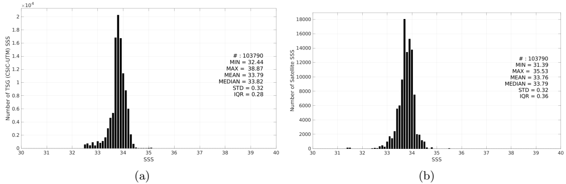
Figure 3: Histograms of SSS from TSG (CSIC-UTM) (a) and CCI SSS L4 POLAR SH Merged-OI v4.41 - 30-day running (ESA) (b) considering all match-up pairs per bins of 0.1 over the Southern Ocean Pi-MEP region and for the full satellite product period.
