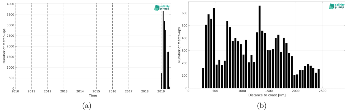
Figure 2: Number of match-ups between Saildrone and CCI SSS L4 POLAR SH Merged-OI v4.41 - 30-day running (ESA) SSS as a function of time (a) and as function of the distance to coast (b) over the Southern Ocean Pi-MEP region and for the full satellite product period.
