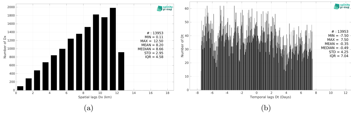
Figure 6: Histograms of the spatial (a) and temporal (b) lags between the location/time of the Saildrone measurement and the date of the corresponding CCI SSS L4 POLAR SH Merged-OI v4.41 - 30-day running (ESA) SSS pixel.
