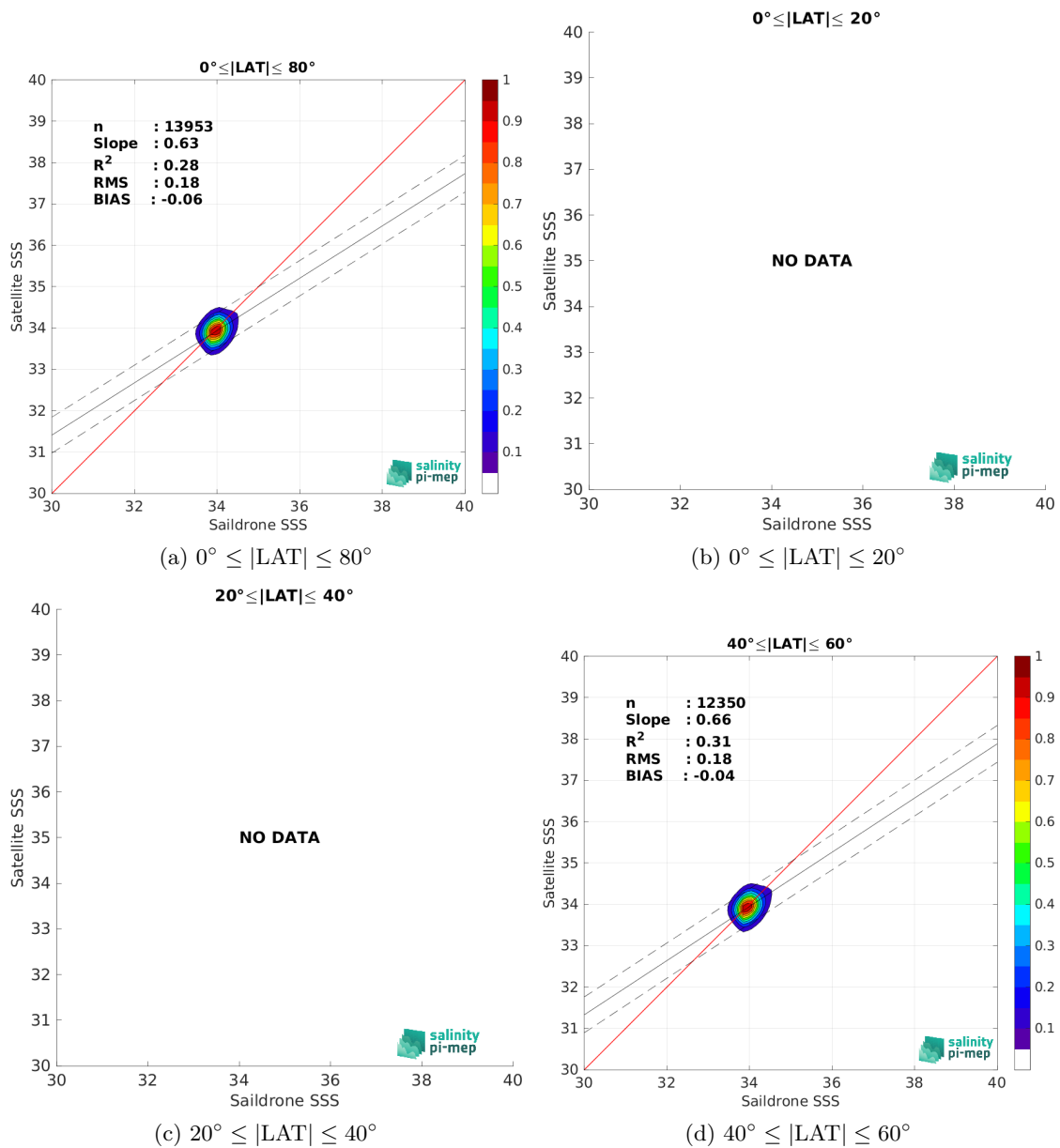
Figure 10: Contour maps of the concentration of CCI SSS L4 POLAR SH Merged-OI v4.41 - 30-day running (ESA) SSS (y-axis) versus Saildrone SSS (x-axis) at match-up pairs for different latitude bands. For each plot, the red line shows x=y . The black thin and dashed lines indicate a linear fit through the data cloud and the \pm 95\% confidence levels, respectively. The number match-up pairs n , the slope and R^2 coefficient of the linear fit, the root mean square (RMS) and the mean bias between satellite and in situ data are indicated for each latitude band in each plots.
