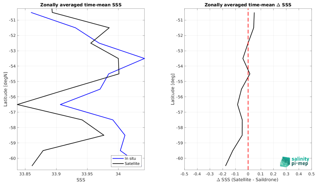
Figure 9: Left panel: Zonal mean SSS from CCI SSS L4 POLAR SH Merged-OI v4.41 - 30-day running (ESA) satellite product (black) and from Saildrone (blue). Right panel: Zonal mean of \Delta SSS (Satellite - Saildrone) for all the collected Pi-MEP match-up pairs estimated over the full satellite product period.
