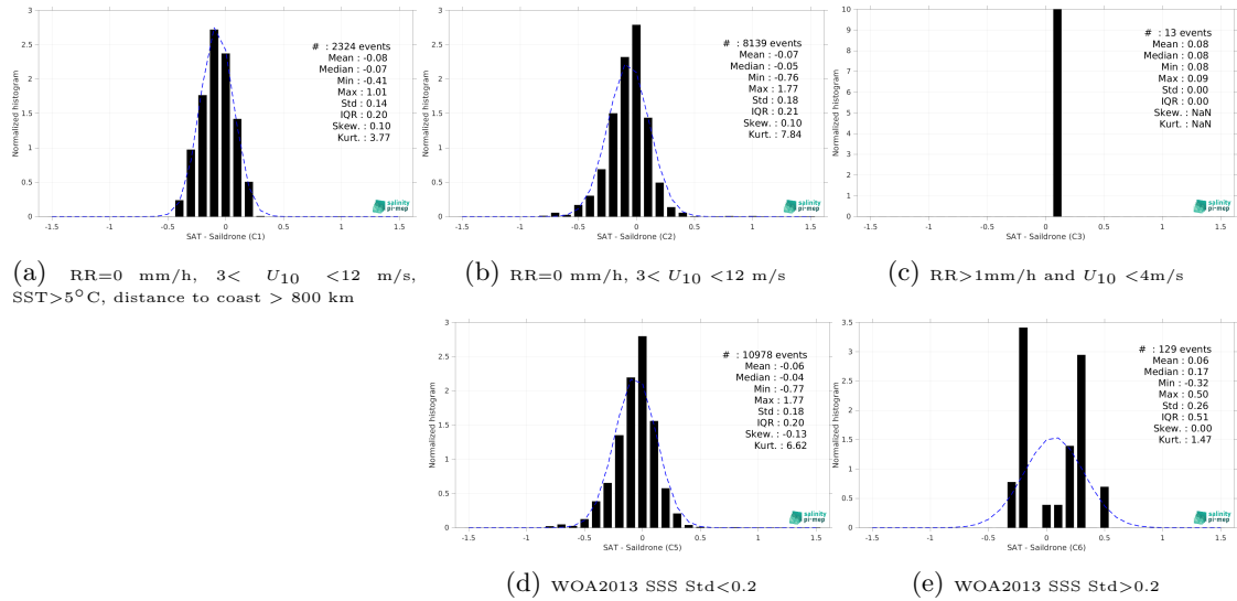
Figure 15: Normalized histogram of \Delta SSS (CCI SSS L4 POLAR SH Merged-OI v4.41 - 30-day running (ESA) - Saildrone) for 5 different subdatasets corresponding to: RR=0 mm/h, 3 < U_{10} < 12 m/s, SST > 5°C, distance to coast > 800 km (a), RR=0 mm/h, 3 < U_{10} < 12 m/s (b), RR > 1mm/h and U_{10} < 4 m/s (c), WOA2013 SSS Std < 0.2 (d), WOA2013 SSS Std > 0.2 (e).
