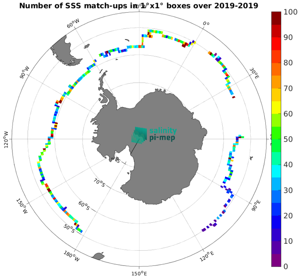
Figure 5: Number of SSS match-ups between Saildrone SSS and the CCI SSS L4 POLAR SH Merged-OI v4.41 - 30-day running (ESA) SSS product for the Southern Ocean Pi-MEP region over 1^\circ \times 1^\circ boxes and for the full satellite product period.
