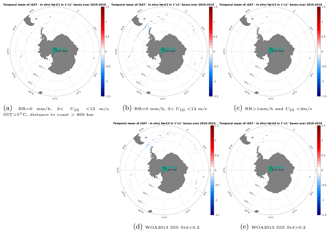
Figure 14: Temporal mean gridded over spatial boxes of size 1^\circ \times 1^\circ of \Delta SSS (CCI SSS L4 POLAR SH Merged-OI v4.41 - 30-day running (ESA) - Sailability) for 5 different subdatasets corresponding to:RR=0 mm/h, 3 < U_{10} < 12 m/s, SST >5^\circ C, distance to coast > 800 km (a), RR=0 mm/h, 3 < U_{10} < 12 m/s (b), RR >1 mm/h and U_{10} < 4 m/s (c), WOA2013 SSS Std <0.2 (d), WOA2013 SSS Std >0.2 (e).
