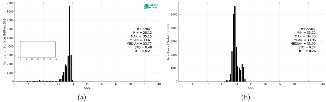
Figure 3: Histograms of SSS from Surface drifters (a) and CCI SSS L4 POLAR SH Merged-OI v4.41 - 30-day running (ESA) (b) considering all match-up pairs per bins of 0.1 over the Southern Ocean Pi-MEP region and for the full satellite product period.
