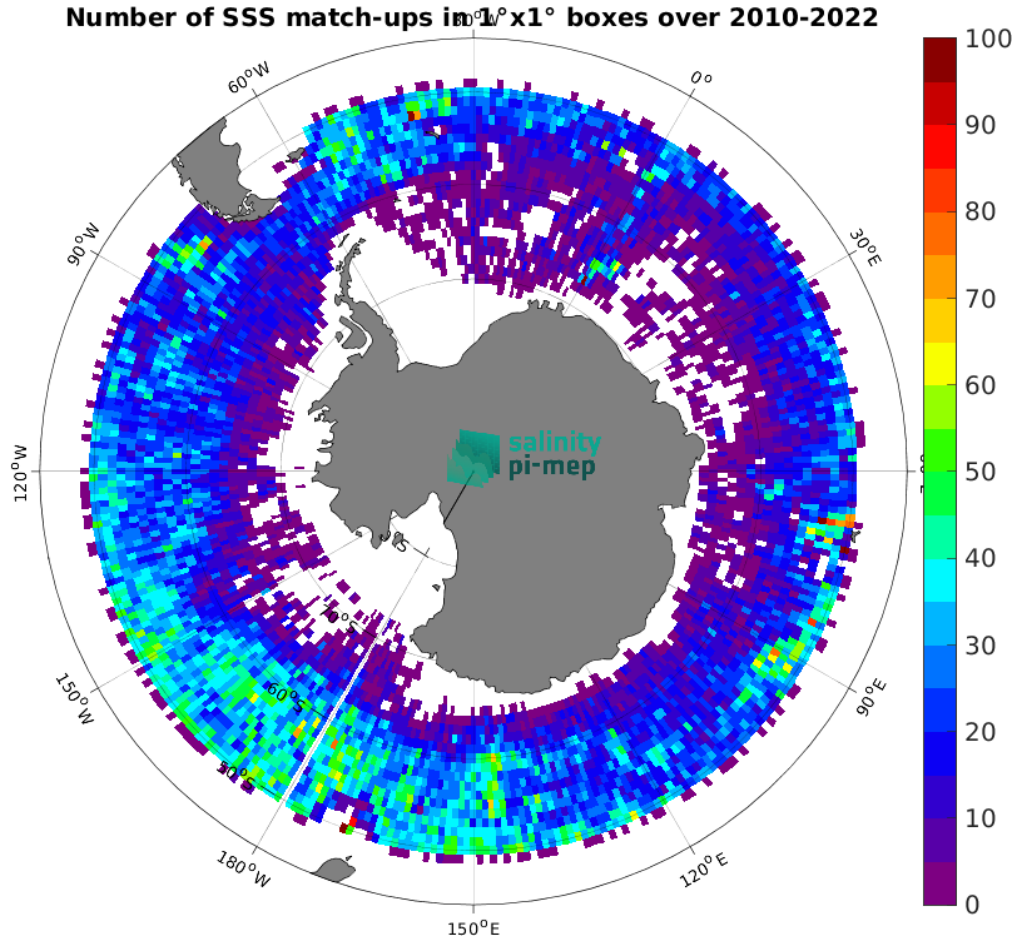
Figure 5: Number of SSS match-ups between Argo SSS and the CCI SSS L4 POLAR SH Merged-OI v4.41 - 30-day running (ESA) SSS product for the Southern Ocean Pi-MEP region over 1^\circ \times 1^\circ boxes and for the full satellite product period.
