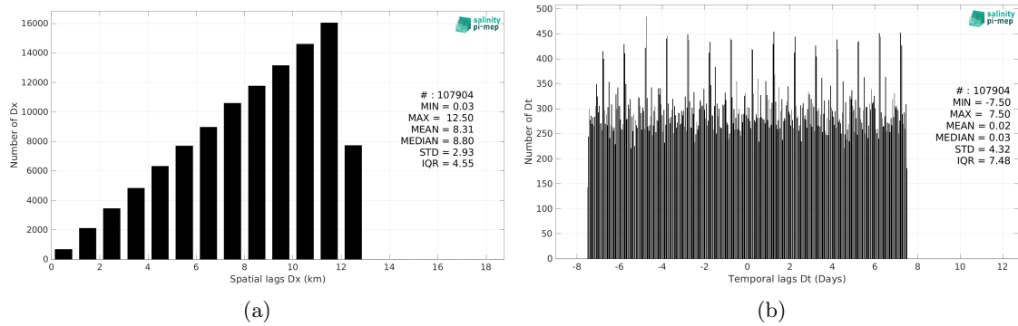
Figure 6: Histograms of the spatial (a) and temporal (b) lags between the location/time of the Argo measurement and the date of the corresponding CCI SSS L4 POLAR SH Merged-OI v4.41 - 30-day running (ESA) SSS pixel.
