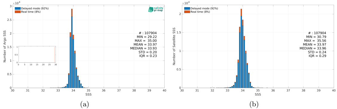
Figure 3: Histograms of SSS from Argo (a) and CCI SSS L4 POLAR SH Merged-OI v4.41 - 30-day running (ESA) (b) considering all match-up pairs per bins of 0.1 over the Southern Ocean Pi-MEP region and for the full satellite product period.
