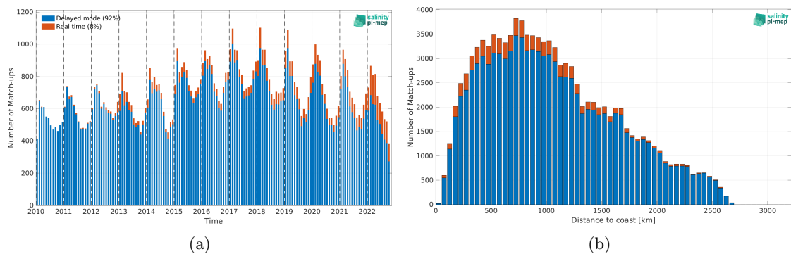
Figure 2: Number of match-ups between Argo and CCI SSS L4 POLAR SH Merged-OI v4.41 - 30-day running (ESA) SSS as a function of time (a) and as function of the distance to coast (b) over the Southern Ocean Pi-MEP region and for the full satellite product period.
