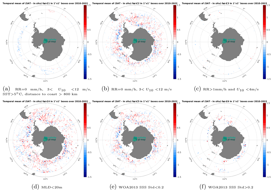
Figure 14: Temporal mean gridded over spatial boxes of size 1^\circ \times 1^\circ of \Delta SSS (CCI SSS L4 POLAR SH Merged-OI v4.41 - 30-day running (ESA) - Argo) for 6 different subdatasets corresponding to:RR=0 mm/h, 3 < U_{10} < 12 m/s, SST >5^\circ C, distance to coast > 800 km (a), RR=0 mm/h, 3 < U_{10} < 12 m/s (b), RR >1 mm/h and U_{10} < 4 m/s (c),MLD <20 m (d),WOA2013 SSS Std <0.2 (e),WOA2013 SSS Std >0.2 (f).
