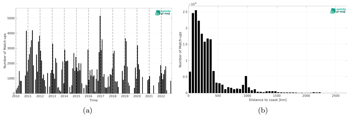
Figure 1: Number of match-ups between TSG (SAMOS) and CCI SSS L4 POLAR SH Merged-OI v4.4 - 7-day running (ESA) SSS as a function of time (a) and as function of the distance to coast (b) over the Southern Ocean Pi-MEP region and for the full satellite product period.
