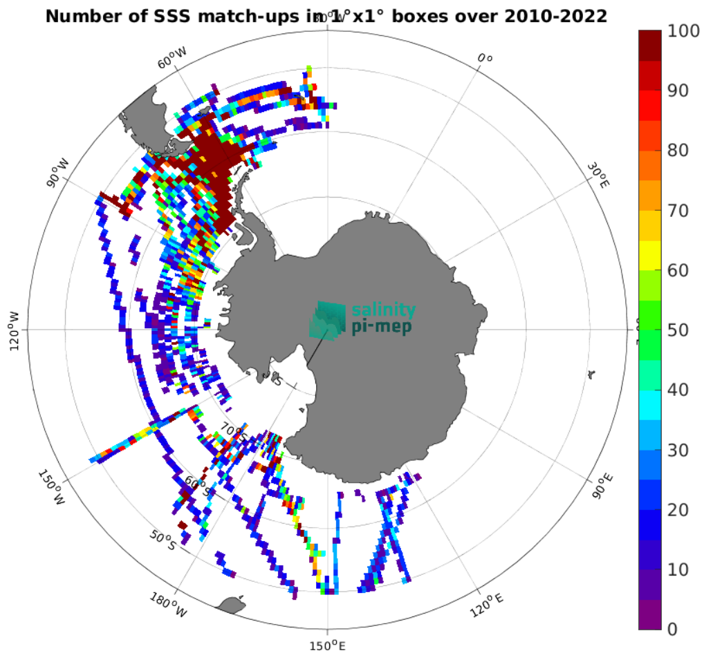
Figure 4: Number of SSS match-ups between TSG (SAMOS) SSS and the CCI SSS L4 POLAR SH Merged-OI v4.4 - 7-day running (ESA) SSS product for the Southern Ocean Pi-MEP region over 1^\circ \times 1^\circ boxes and for the full satellite product period.
