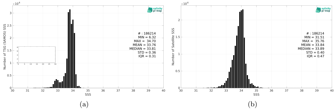
Figure 2: Histograms of SSS from TSG (SAMOS) (a) and CCI SSS L4 POLAR SH Merged-OI v4.4 - 7-day running (ESA) (b) considering all match-up pairs per bins of 0.1 over the Southern Ocean Pi-MEP region and for the full satellite product period.
