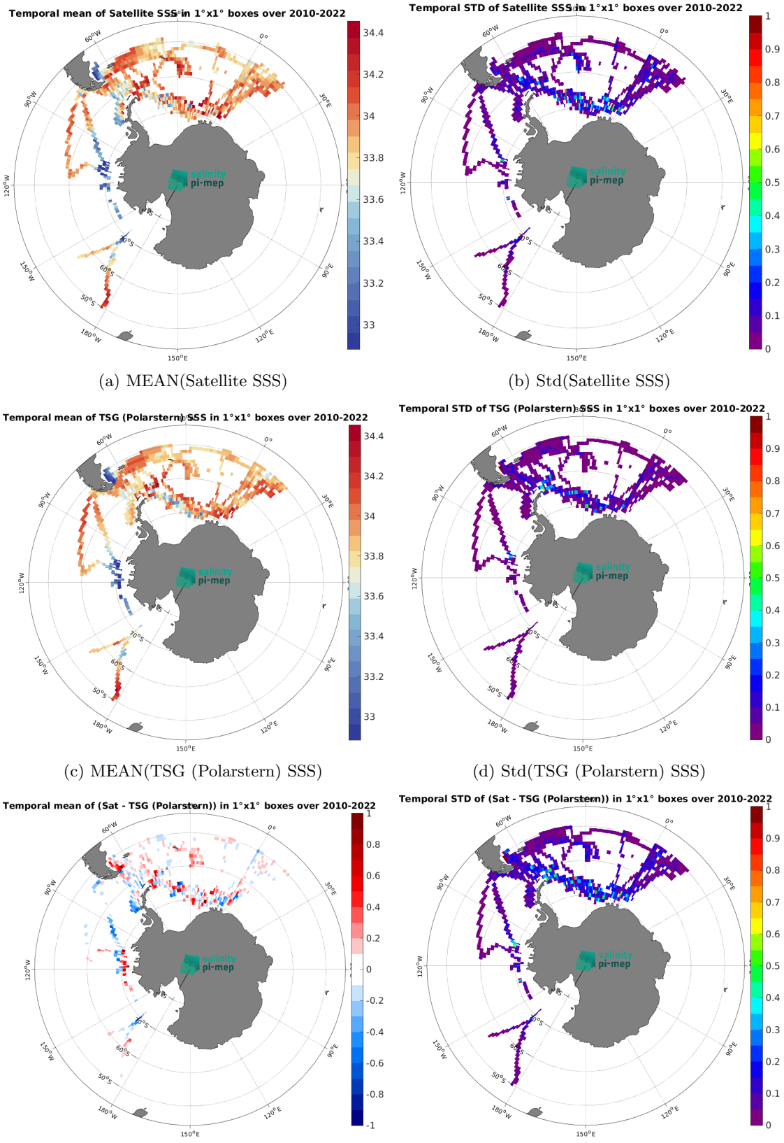
Figure 6: Temporal mean (left) and Std (right) of SSS from CCI SSS L4 POLAR SH Merged-OI v4.4 - 7-day running (ESA) (top), TSG (Polarstern) (middle), and of \Delta SSS (Satellite - TSG (Polarstern)). Only match-up pairs are used to generate these maps.
