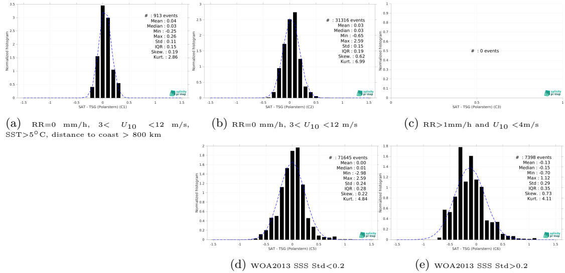
Figure 13: Normalized histogram of \Delta SSS (CCI SSS L4 POLAR SH Merged-OI v4.4 - 7-day running (ESA) - TSG (Polarstern)) for 5 different subdatasets corresponding to: RR=0 mm/h, 3 < U_{10} < 12 m/s, SST>5°C, distance to coast > 800 km (a), RR=0 mm/h, 3 < U_{10} < 12 m/s (b), RR>1mm/h and U_{10} < 4 m/s (c), WOA2013 SSS Std<0.2 (d), WOA2013 SSS Std>0.2 (e).
