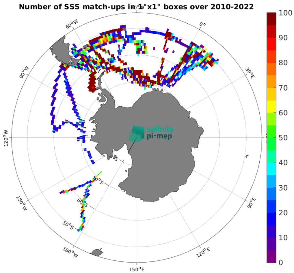
Figure 4: Number of SSS match-ups between TSG (Polarstern) SSS and the CCI SSS L4 POLAR SH Merged-OI v4.4 - 7-day running (ESA) SSS product for the Southern Ocean Pi-MEP region over 1^\circ \times 1^\circ boxes and for the full satellite product period.
