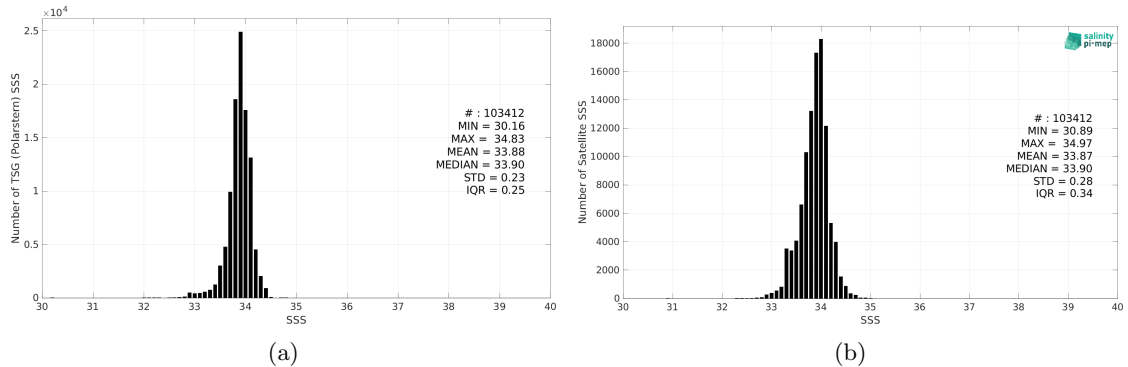
Figure 2: Histograms of SSS from TSG (Polarstern) (a) and CCI SSS L4 POLAR SH Merged-OI v4.4 - 7-day running (ESA) (b) considering all match-up pairs per bins of 0.1 over the Southern Ocean Pi-MEP region and for the full satellite product period.
