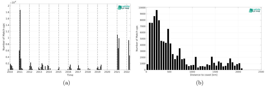
Figure 1: Number of match-ups between TSG (Polarstern) and CCI SSS L4 POLAR SH Merged-OI v4.4 - 7-day running (ESA) SSS as a function of time (a) and as function of the distance to coast (b) over the Southern Ocean Pi-MEP region and for the full satellite product period.
