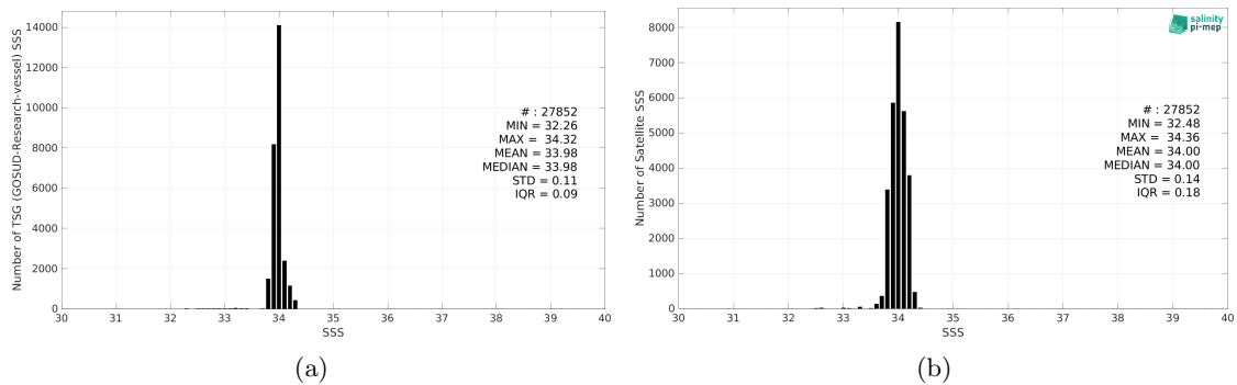
Figure 2: Histograms of SSS from TSG (GOSUD-Research-vessel) (a) and CCI SSS L4 POLAR SH Merged-OI v4.4 - 7-day running (ESA) (b) considering all match-up pairs per bins of 0.1 over the Southern Ocean Pi-MEP region and for the full satellite product period.
