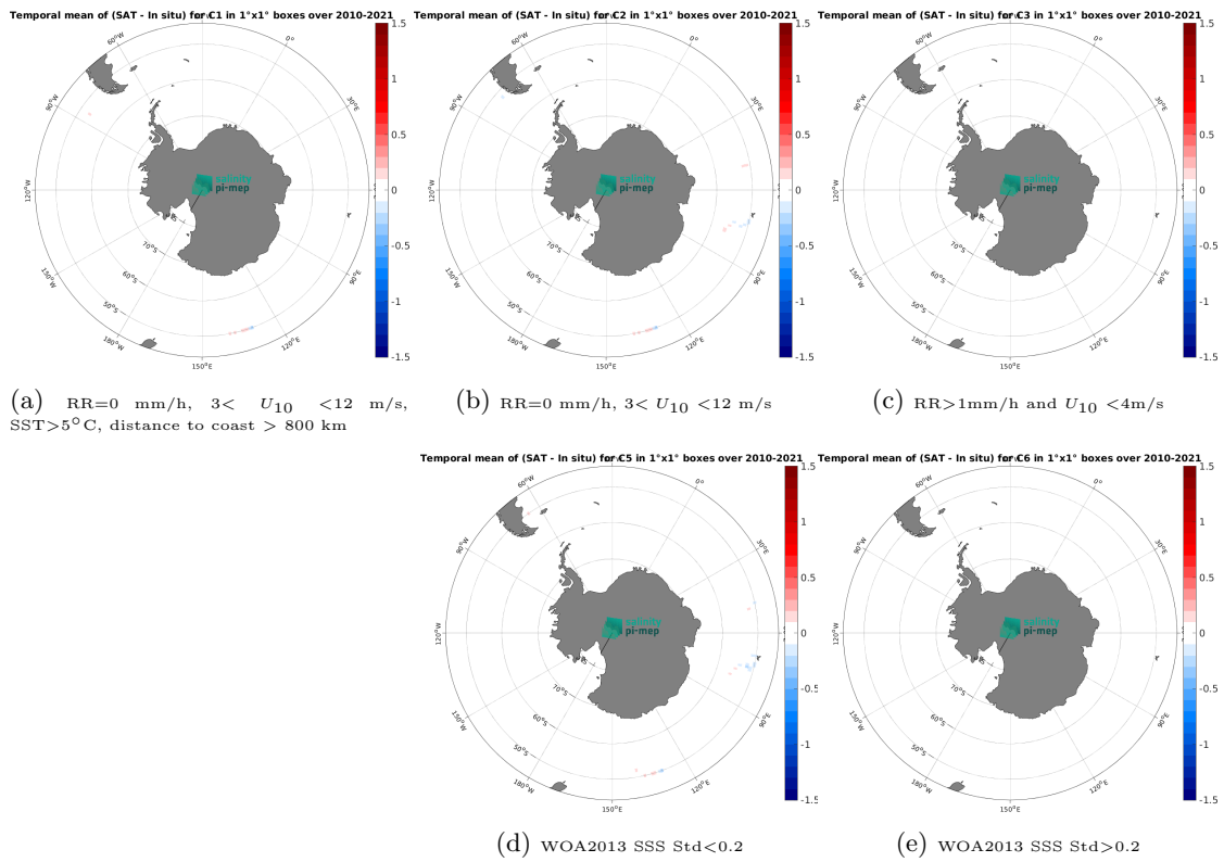
Figure 12: Temporal mean gridded over spatial boxes of size 1°×1° of \Delta SSS (CCI SSS L4 POLAR SH Merged-OI v4.4 - 7-day running (ESA) - TSG (GOSUD-Research-vessel)) for 5 different subdatasets corresponding to:RR=0 mm/h, 3 < U_{10} < 12 m/s, SST>5°C, distance to coast > 800 km (a), RR=0 mm/h, 3 < U_{10} < 12 m/s (b), RR>1mm/h and U_{10} < 4 m/s (c), WOA2013 SSS Std<0.2 (d), WOA2013 SSS Std>0.2 (e).
