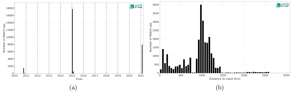
Figure 1: Number of match-ups between TSG (GOSUD-Research-vessel) and CCI SSS L4 POLAR SH Merged-OI v4.4 - 7-day running (ESA) SSS as a function of time (a) and as function of the distance to coast (b) over the Southern Ocean Pi-MEP region and for the full satellite product period.
