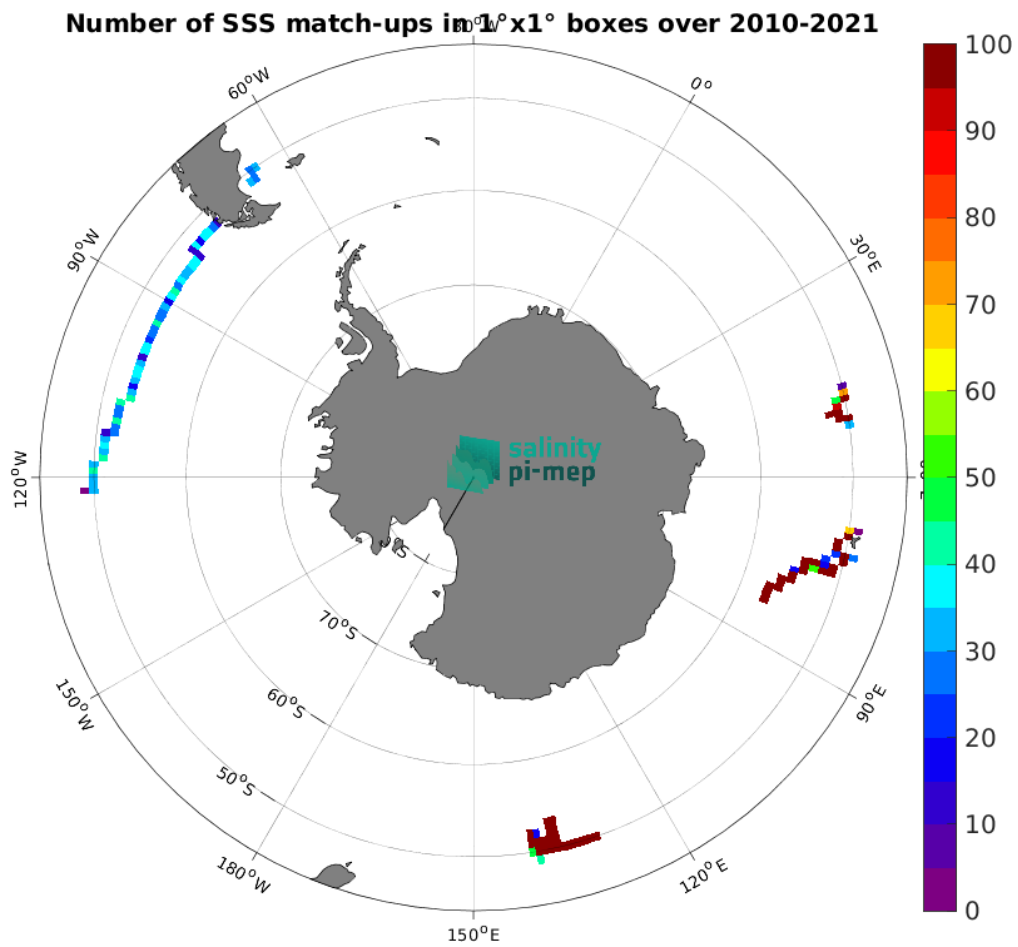
Figure 4: Number of SSS match-ups between TSG (GOSUD-Research-vessel) SSS and the CCI SSS L4 POLAR SH Merged-OI v4.4 - 7-day running (ESA) SSS product for the Southern Ocean Pi-MEP region over 1^{\circ} \times 1^{\circ} boxes and for the full satellite product period.
