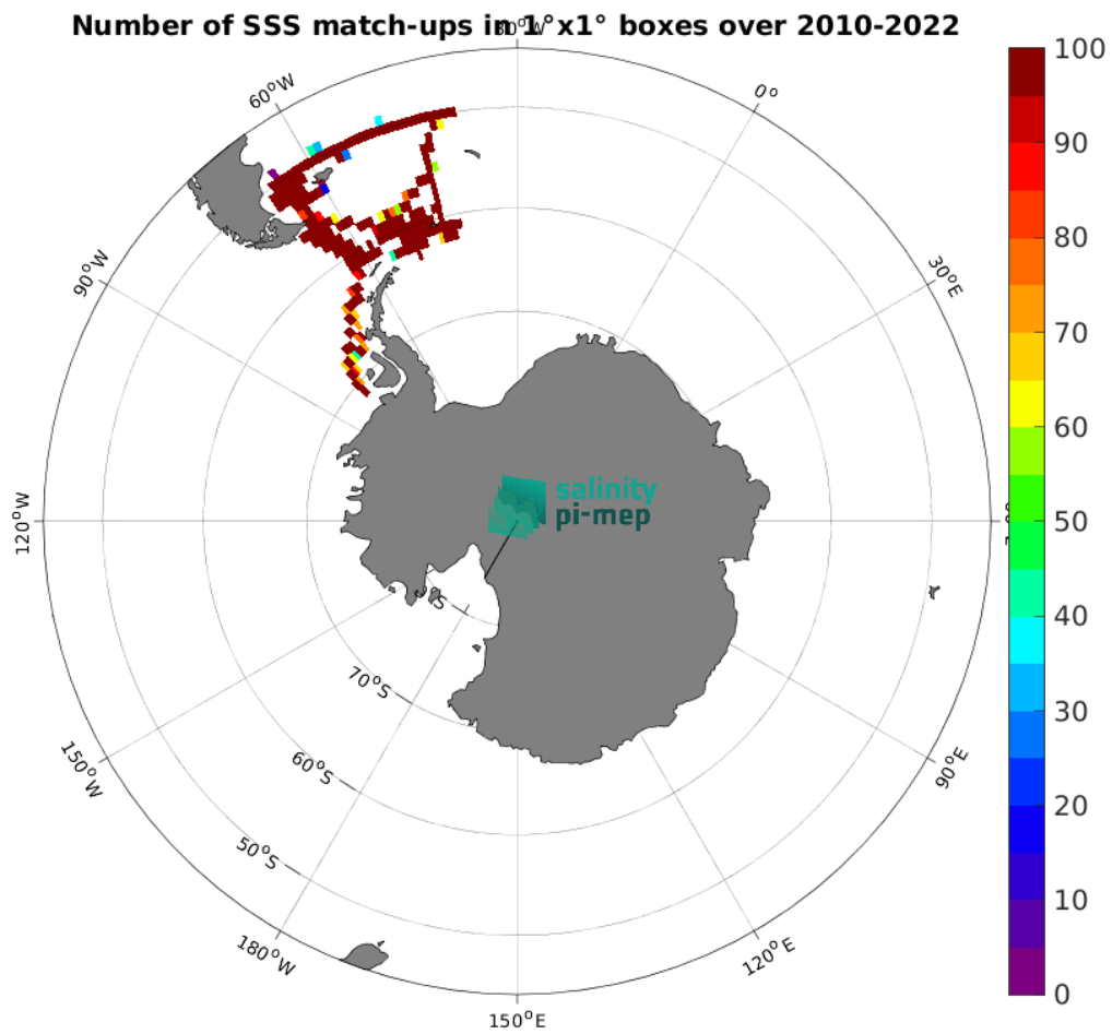
Figure 4: Number of SSS match-ups between TSG (CSIC-UTM) SSS and the CCI SSS L4 POLAR SH Merged-OI v4.4 - 7-day running (ESA) SSS product for the Southern Ocean Pi-MEP region over 1^\circ \times 1^\circ boxes and for the full satellite product period.
