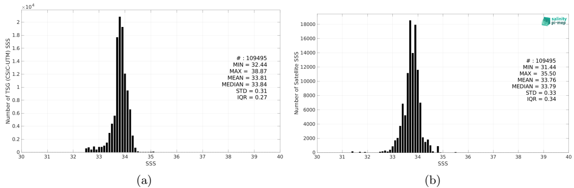
Figure 2: Histograms of SSS from TSG (CSIC-UTM) (a) and CCI SSS L4 POLAR SH Merged-OI v4.4 - 7-day running (ESA) (b) considering all match-up pairs per bins of 0.1 over the Southern Ocean Pi-MEP region and for the full satellite product period.
