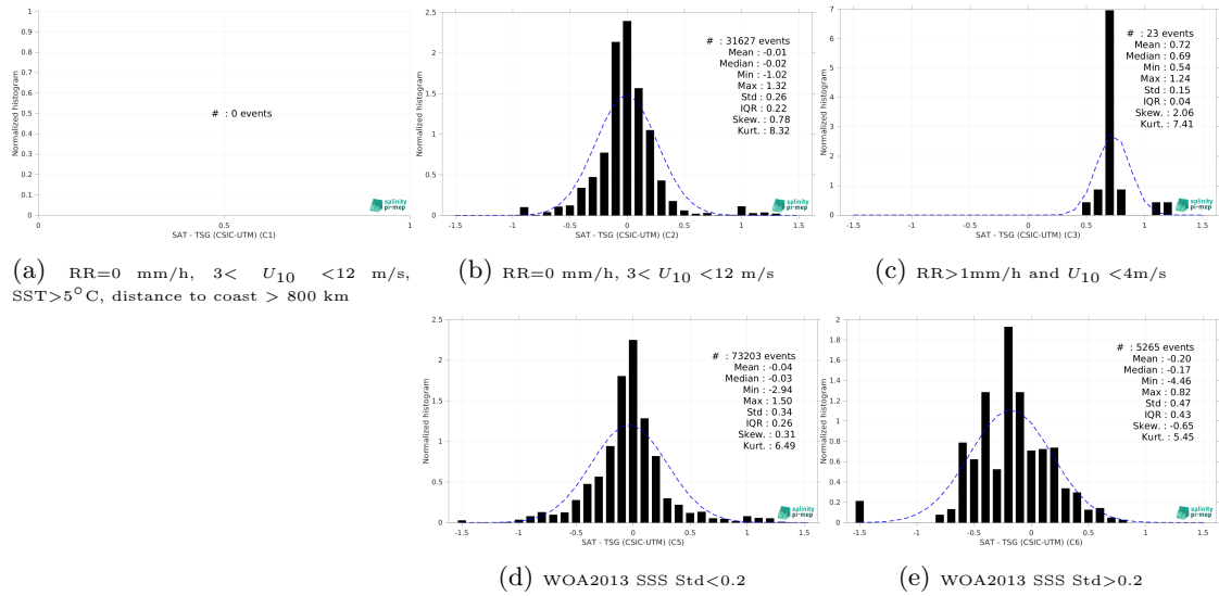
Figure 13: Normalized histogram of \Delta\text{SSS} (CCI SSS L4 POLAR SH Merged-OI v4.4 - 7-day running (ESA) - TSG (CSIC-UTM)) for 5 different subdatasets corresponding to: RR=0 mm/h, 3 < U_{10} < 12 m/s, SST > 5^{\circ}\text{C} , distance to coast > 800 km (a), RR=0 mm/h, 3 < U_{10} < 12 m/s (b), RR > 1\text{mm/h} and U_{10} < 4\text{m/s} (c), WOA2013 SSS Std < 0.2 (d), WOA2013 SSS Std > 0.2 (e).
