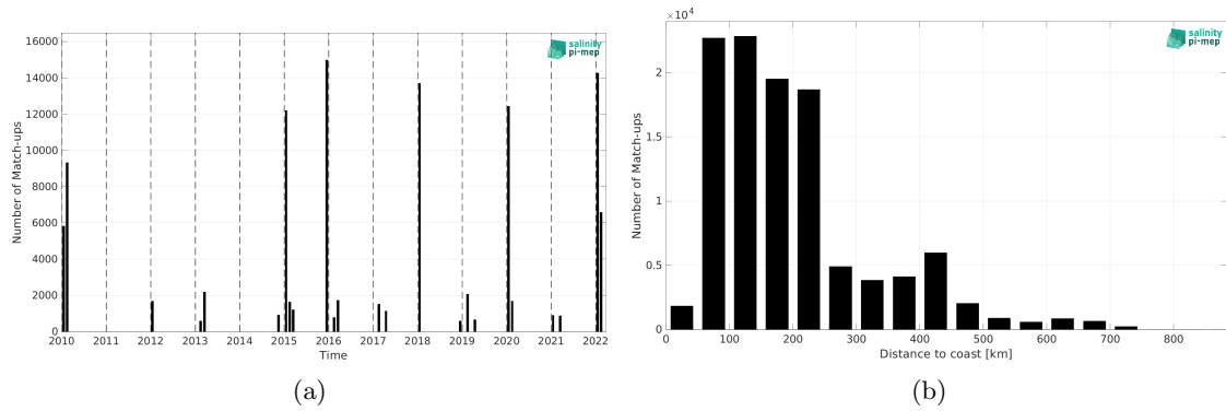
Figure 1: Number of match-ups between TSG (CSIC-UTM) and CCI SSS L4 POLAR SH Merged-OI v4.4 - 7-day running (ESA) SSS as a function of time (a) and as function of the distance to coast (b) over the Southern Ocean Pi-MEP region and for the full satellite product period.
