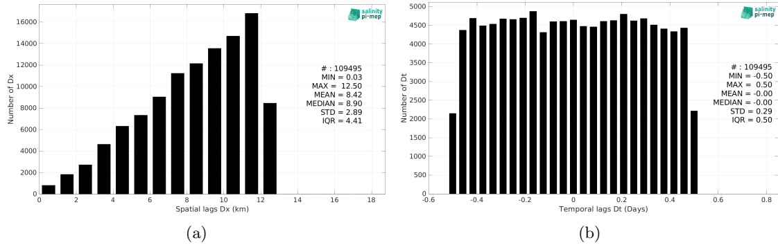
Figure 5: Histograms of the spatial (a) and temporal (b) lags between the location/time of the TSG (CSIC-UTM) measurement and the date of the corresponding CCI SSS L4 POLAR SH Merged-OI v4.4 - 7-day running (ESA) SSS pixel.
