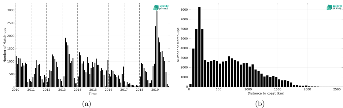
Figure 1: Number of match-ups between Marine mammals and CCI SSS L4 POLAR SH Merged-OI v4.4 - 7-day running (ESA) SSS as a function of time (a) and as function of the distance to coast (b) over the Southern Ocean Pi-MEP region and for the full satellite product period.
