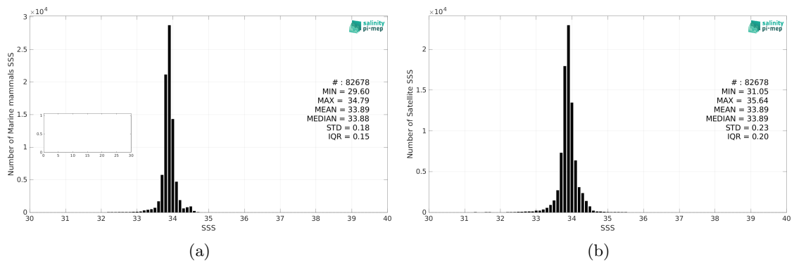
Figure 2: Histograms of SSS from Marine mammals (a) and CCI SSS L4 POLAR SH Merged-OI v4.4 - 7-day running (ESA) (b) considering all match-up pairs per bins of 0.1 over the Southern Ocean Pi-MEP region and for the full satellite product period.
