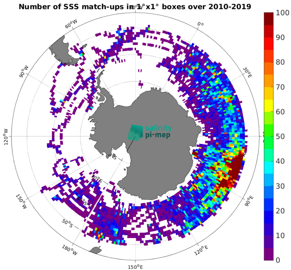
Figure 4: Number of SSS match-ups between Marine mammals SSS and the CCI SSS L4 POLAR SH Merged-OI v4.4 - 7-day running (ESA) SSS product for the Southern Ocean Pi-MEP region over 1^{\circ} \times 1^{\circ} boxes and for the full satellite product period.
