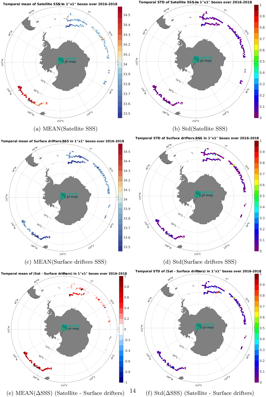
Figure 5: Temporal mean (left) and Std (right) of SSS from CCI SSS L4 POLAR SH Merged-OI v4.4 - 7-day running (ESA) (top), Surface drifters (middle), and of \Delta SSS (Satellite - Surface drifters). Only match-up pairs are used to generate these maps.
