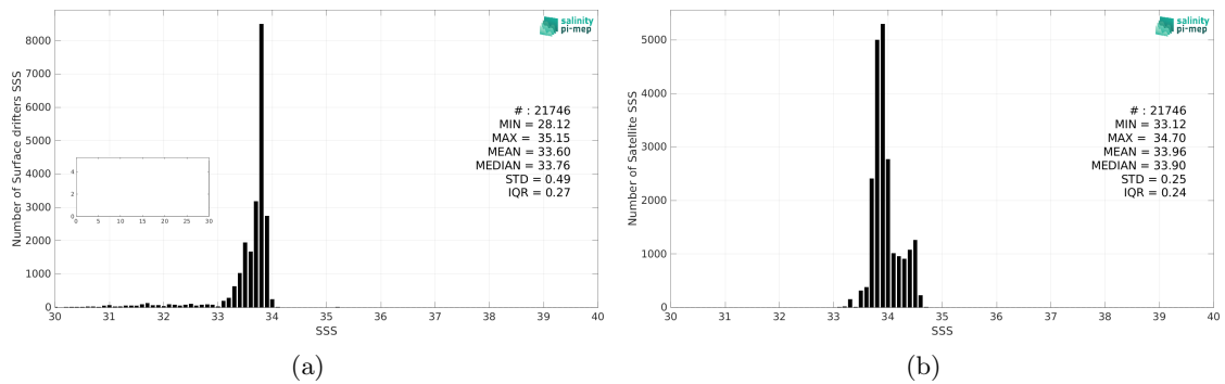
Figure 2: Histograms of SSS from Surface drifters (a) and CCI SSS L4 POLAR SH Merged-OI v4.4 - 7-day running (ESA) (b) considering all match-up pairs per bins of 0.1 over the Southern Ocean Pi-MEP region and for the full satellite product period.
