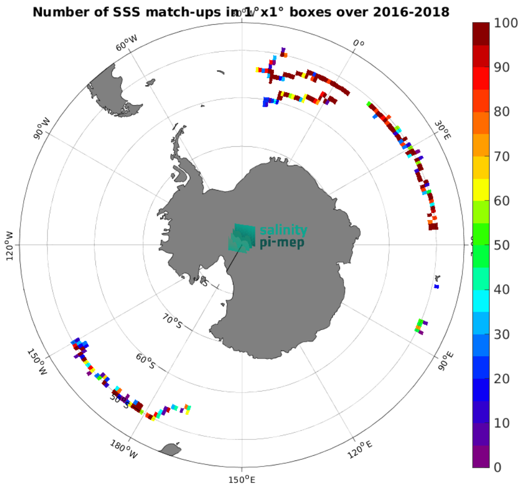
Figure 3: Number of SSS match-ups between Surface drifters SSS and the CCI SSS L4 POLAR SH Merged-OI v4.4 - 7-day running (ESA) SSS product for the Southern Ocean Pi-MEP region over 1°x1° boxes and for the full satellite product period.
