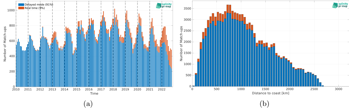
Figure 1: Number of match-ups between Argo and CCI SSS L4 POLAR SH Merged-OI v4.4 - 7-day running (ESA) SSS as a function of time (a) and as function of the distance to coast (b) over the Southern Ocean Pi-MEP region and for the full satellite product period.
