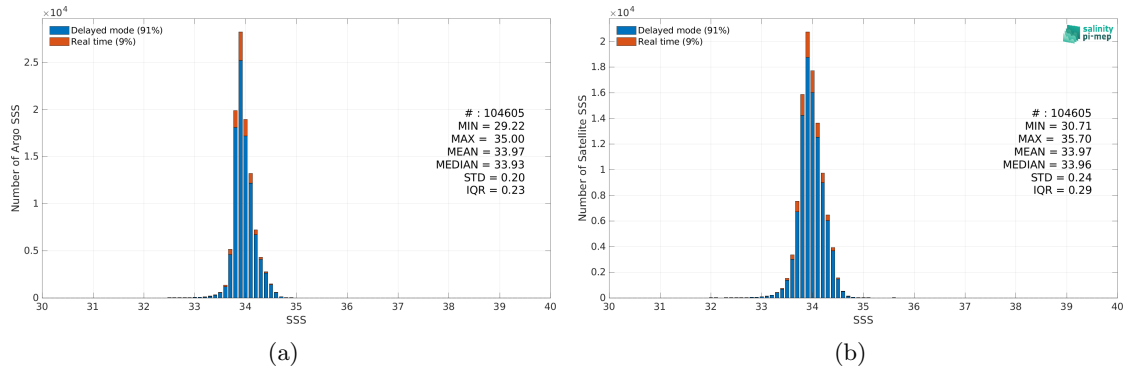
Figure 2: Histograms of SSS from Argo (a) and CCI SSS L4 POLAR SH Merged-OI v4.4 - 7-day running (ESA) (b) considering all match-up pairs per bins of 0.1 over the Southern Ocean Pi-MEP region and for the full satellite product period.
