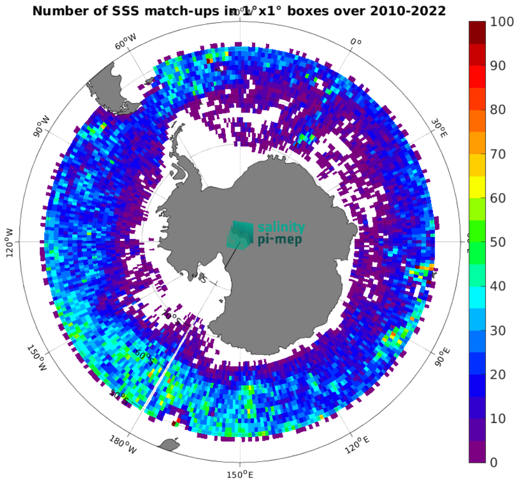
Figure 4: Number of SSS match-ups between Argo SSS and the CCI SSS L4 POLAR SH Merged-OI v4.4 - 7-day running (ESA) SSS product for the Southern Ocean Pi-MEP region over 1^\circ \times 1^\circ boxes and for the full satellite product period.
