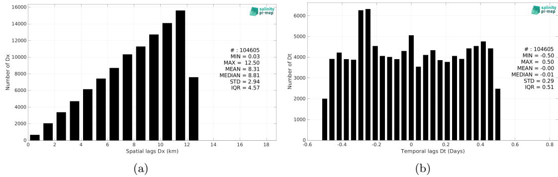
Figure 5: Histograms of the spatial (a) and temporal (b) lags between the location/time of the Argo measurement and the date of the corresponding CCI SSS L4 POLAR SH Merged-OI v4.4 - 7-day running (ESA) SSS pixel.
