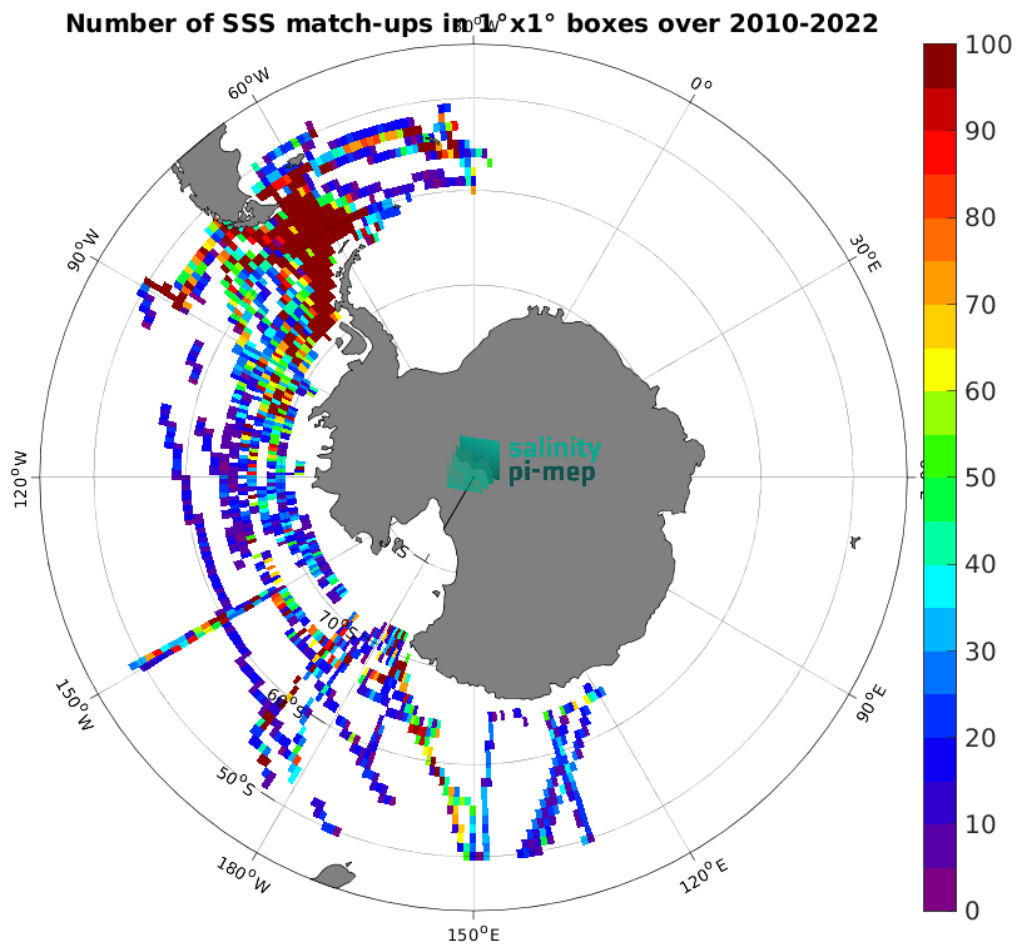
Figure 4: Number of SSS match-ups between TSG (SAMOS) SSS and the CCI SSS L4 POLAR SH Merged-OI v4.4 - 30-day running (ESA) SSS product for the Southern Ocean Pi-MEP region over 1^\circ \times 1^\circ boxes and for the full satellite product period.
