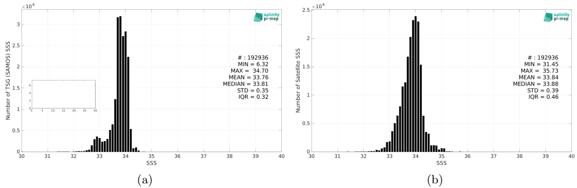
Figure 2: Histograms of SSS from TSG (SAMOS) (a) and CCI SSS L4 POLAR SH Merged-OI v4.4 - 30-day running (ESA) (b) considering all match-up pairs per bins of 0.1 over the Southern Ocean Pi-MEP region and for the full satellite product period.
