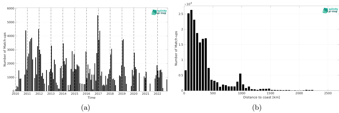
Figure 1: Number of match-ups between TSG (SAMOS) and CCI SSS L4 POLAR SH Merged-OI v4.4 - 30-day running (ESA) SSS as a function of time (a) and as function of the distance to coast (b) over the Southern Ocean Pi-MEP region and for the full satellite product period.
