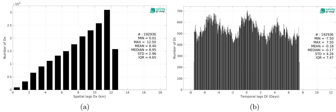
Figure 5: Histograms of the spatial (a) and temporal (b) lags between the location/time of the TSG (SAMOS) measurement and the date of the corresponding CCI SSS L4 POLAR SH Merged-OI v4.4 - 30-day running (ESA) SSS pixel.
