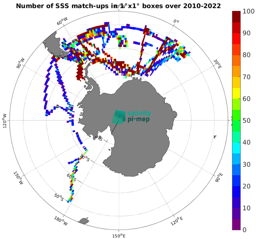
Figure 4: Number of SSS match-ups between TSG (Polarstern) SSS and the CCI SSS L4 POLAR SH Merged-OI v4.4 - 30-day running (ESA) SSS product for the Southern Ocean Pi-MEP region over 1^\circ \times 1^\circ boxes and for the full satellite product period.
