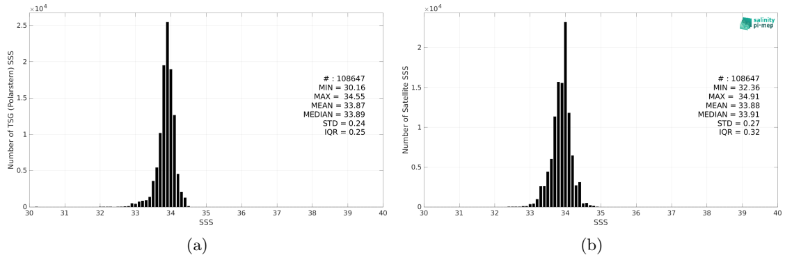
Figure 2: Histograms of SSS from TSG (Polarstern) (a) and CCI SSS L4 POLAR SH Merged-OI v4.4 - 30-day running (ESA) (b) considering all match-up pairs per bins of 0.1 over the Southern Ocean Pi-MEP region and for the full satellite product period.
