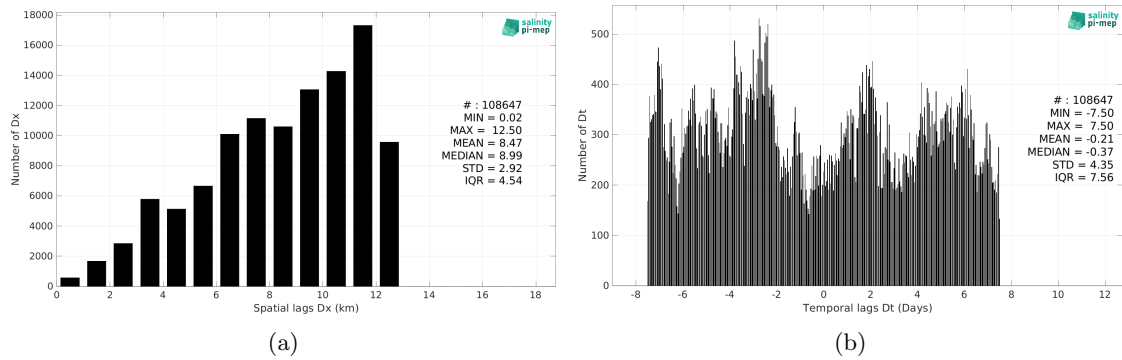
Figure 5: Histograms of the spatial (a) and temporal (b) lags between the location/time of the TSG (Polarstern) measurement and the date of the corresponding CCI SSS L4 POLAR SH Merged-OI v4.4 - 30-day running (ESA) SSS pixel.
