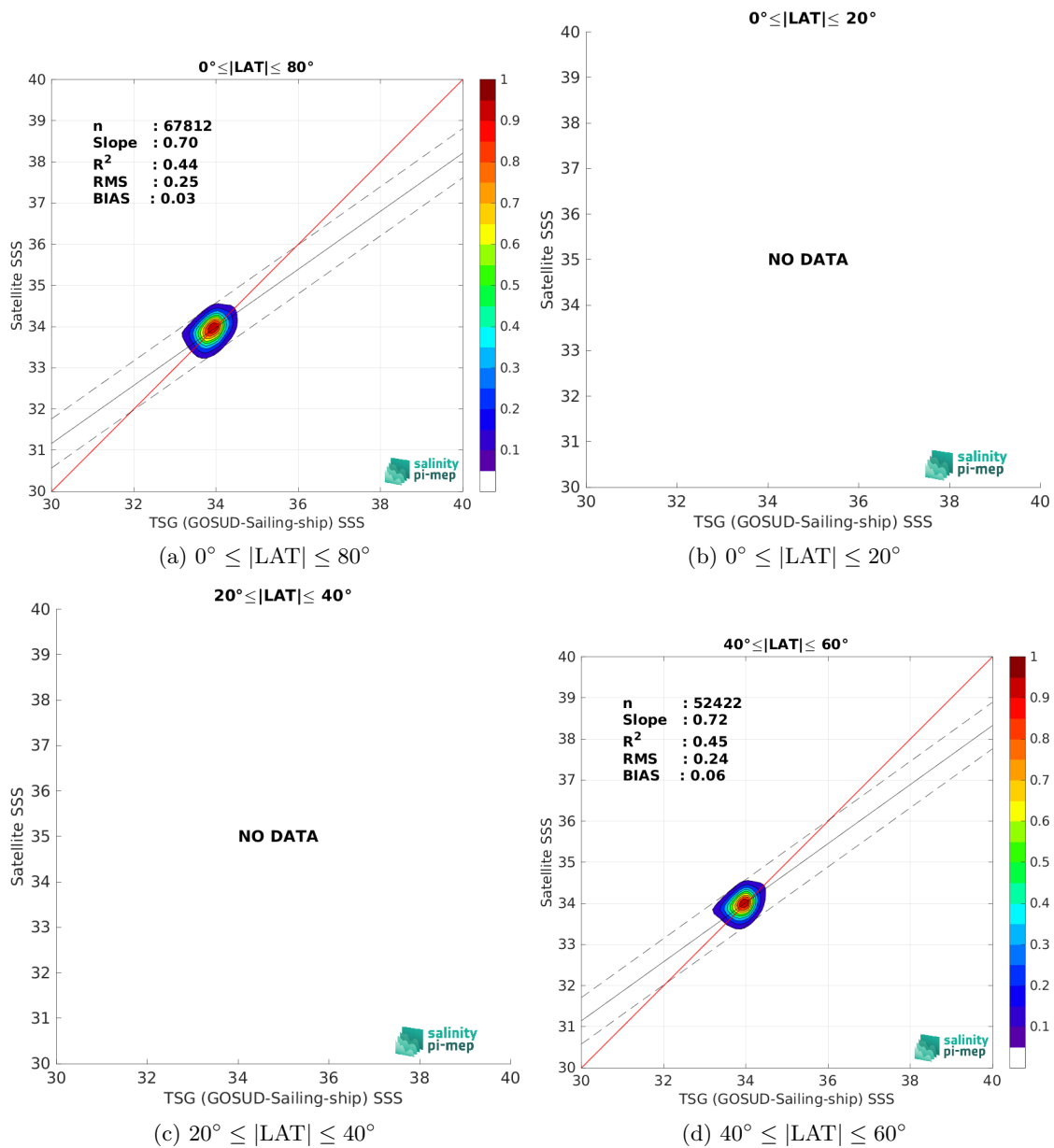
Figure 9: Contour maps of the concentration of CCI SSS L4 POLAR SH Merged-OI v4.4 - 30-day running (ESA) SSS (y-axis) versus TSG (GOSUD-Sailing-ship) SSS (x-axis) at match-up pairs for different latitude bands. For each plot, the red line shows x=y . The black thin and dashed lines indicate a linear fit through the data cloud and the \pm 95\% confidence levels, respectively. The number match-up pairs n , the slope and R^2 coefficient of the linear fit, the root mean square (RMS) and the mean bias between satellite and in situ data are indicated for each latitude band in each plots.
