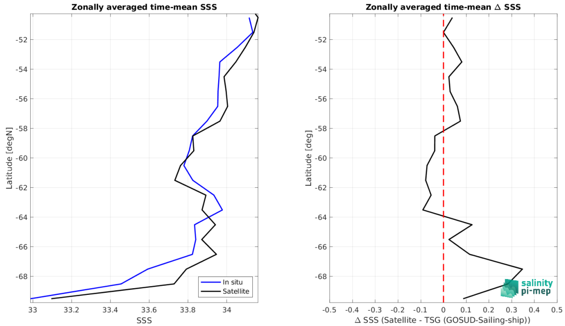
Figure 8: Left panel: Zonal mean SSS from CCI SSS L4 POLAR SH Merged-OI v4.4 - 30-day running (ESA) satellite product (black) and from TSG (GOSUD-Sailing-ship) (blue). Right panel: Zonal mean of \Delta SSS (Satellite - TSG (GOSUD-Sailing-ship)) for all the collected Pi-MEP match-up pairs estimated over the full satellite product period.
