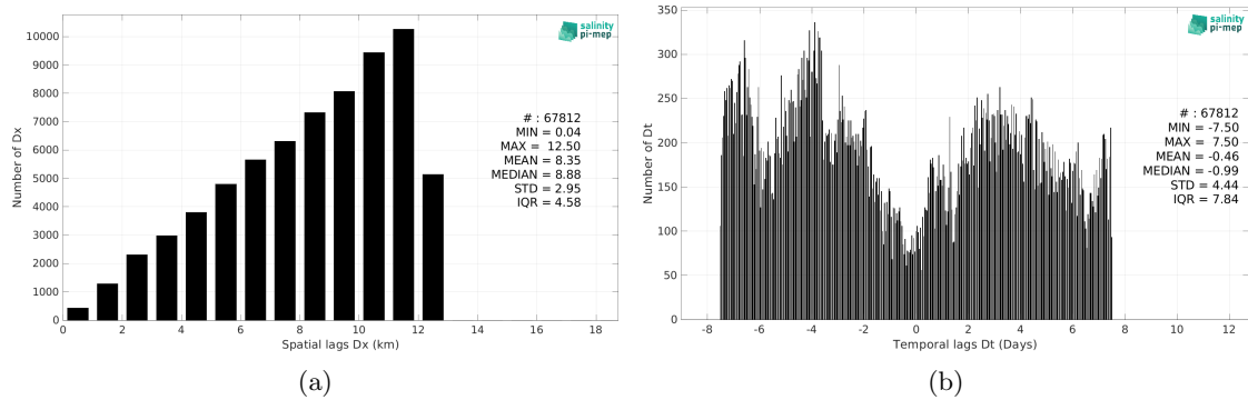
Figure 5: Histograms of the spatial (a) and temporal (b) lags between the location/time of the TSG (GOSUD-Sailing-ship) measurement and the date of the corresponding CCI SSS L4 POLAR SH Merged-OI v4.4 - 30-day running (ESA) SSS pixel.
