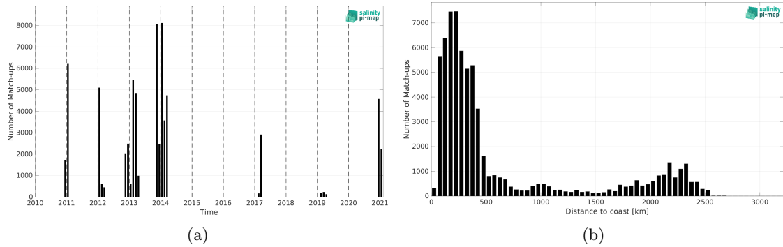
Figure 1: Number of match-ups between TSG (GOSUD-Sailing-ship) and CCI SSS L4 POLAR SH Merged-OI v4.4 - 30-day running (ESA) SSS as a function of time (a) and as function of the distance to coast (b) over the Southern Ocean Pi-MEP region and for the full satellite product period.
