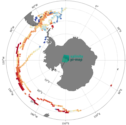
(c) MEAN(TSG (GOSUD-Sailing-ship) SSS)
