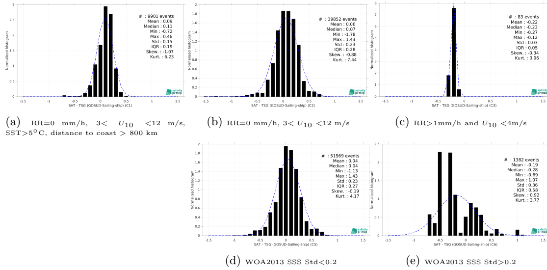
Figure 13: Normalized histogram of \Delta SSS (CCI SSS L4 POLAR SH Merged-OI v4.4 - 30-day running (ESA) - TSG (GOSUD-Sailing-ship)) for 5 different subdatasets corresponding to: RR=0 mm/h, 3 < U_{10} < 12 m/s, SST>5°C, distance to coast > 800 km (a), RR=0 mm/h, 3 < U_{10} < 12 m/s (b), RR>1mm/h and U_{10} < 4 m/s (c), WOA2013 SSS Std<0.2 (d), WOA2013 SSS Std>0.2 (e).
