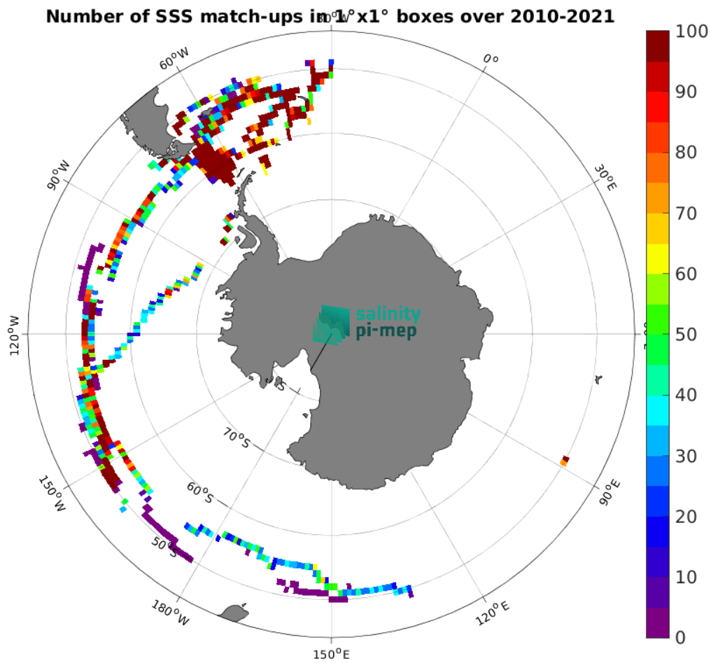
Figure 4: Number of SSS match-ups between TSG (GOSUD-Sailing-ship) SSS and the CCI SSS L4 POLAR SH Merged-OI v4.4 - 30-day running (ESA) SSS product for the Southern Ocean Pi-MEP region over 1^\circ \times 1^\circ boxes and for the full satellite product period.
