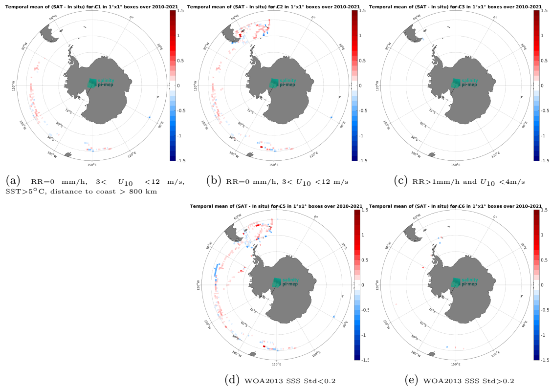
Figure 12: Temporal mean gridded over spatial boxes of size 1°×1° of ΔSSS (CCI SSS L4 POLAR SH Merged-OI v4.4 - 30-day running (ESA) - TSG (GOSUD-Sailing-ship)) for 5 different subdatasets corresponding to:RR=0 mm/h, 3 < U_{10} < 12 m/s, SST>5°C, distance to coast > 800 km (a), RR=0 mm/h, 3 < U_{10} < 12 m/s (b), RR>1mm/h and U_{10} < 4 m/s (c), WOA2013 SSS Std<0.2 (d), WOA2013 SSS Std>0.2 (e).
