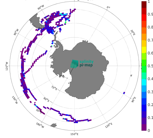
(f) Std( \Delta SSS) (Satellite - TSG (GOSUD-Sailing-ship))
