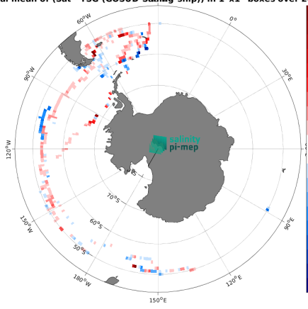
(e) MEAN( \Delta SSS) (Satellite - TSG (GOSUD-Sailing-ship))
