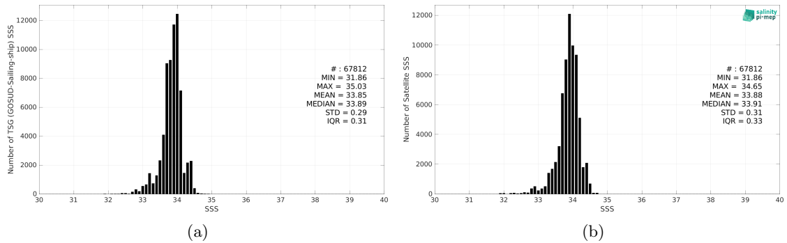
Figure 2: Histograms of SSS from TSG (GOSUD-Sailing-ship) (a) and CCI SSS L4 POLAR SH Merged-OI v4.4 - 30-day running (ESA) (b) considering all match-up pairs per bins of 0.1 over the Southern Ocean Pi-MEP region and for the full satellite product period.
