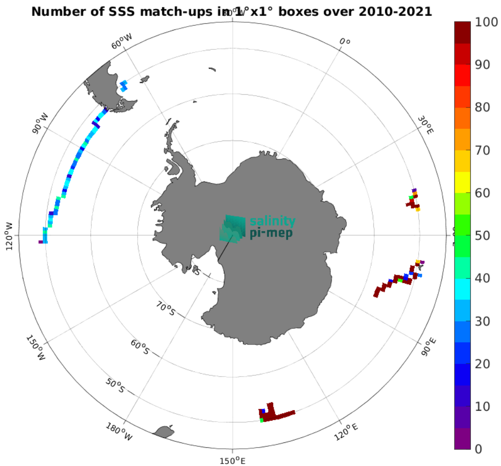
Figure 4: Number of SSS match-ups between TSG (GOSUD-Research-vessel) SSS and the CCI SSS L4 POLAR SH Merged-OI v4.4 - 30-day running (ESA) SSS product for the Southern Ocean Pi-MEP region over 1^\circ \times 1^\circ boxes and for the full satellite product period.
