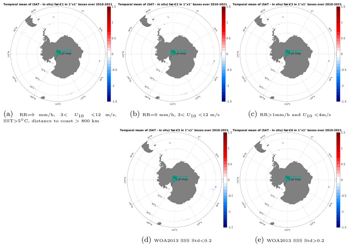
Figure 12: Temporal mean gridded over spatial boxes of size 1°×1° of ΔSSS (CCI SSS L4 POLAR SH Merged-OI v4.4 - 30-day running (ESA) - TSG (GOSUD-Research-vessel)) for 5 different subdatasets corresponding to:RR=0 mm/h, 3 < U_{10} < 12 m/s, SST>5°C, distance to coast > 800 km (a), RR=0 mm/h, 3 < U_{10} < 12 m/s (b), RR>1mm/h and U_{10} < 4 m/s (c), WOA2013 SSS Std<0.2 (d), WOA2013 SSS Std>0.2 (e).
