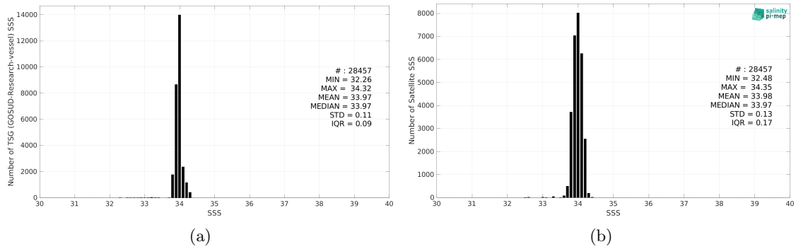
Figure 2: Histograms of SSS from TSG (GOSUD-Research-vessel) (a) and CCI SSS L4 POLAR SH Merged-OI v4.4 - 30-day running (ESA) (b) considering all match-up pairs per bins of 0.1 over the Southern Ocean Pi-MEP region and for the full satellite product period.
