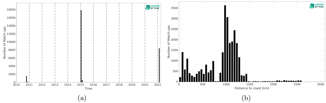
Figure 1: Number of match-ups between TSG (GOSUD-Research-vessel) and CCI SSS L4 POLAR SH Merged-OI v4.4 - 30-day running (ESA) SSS as a function of time (a) and as function of the distance to coast (b) over the Southern Ocean Pi-MEP region and for the full satellite product period.
