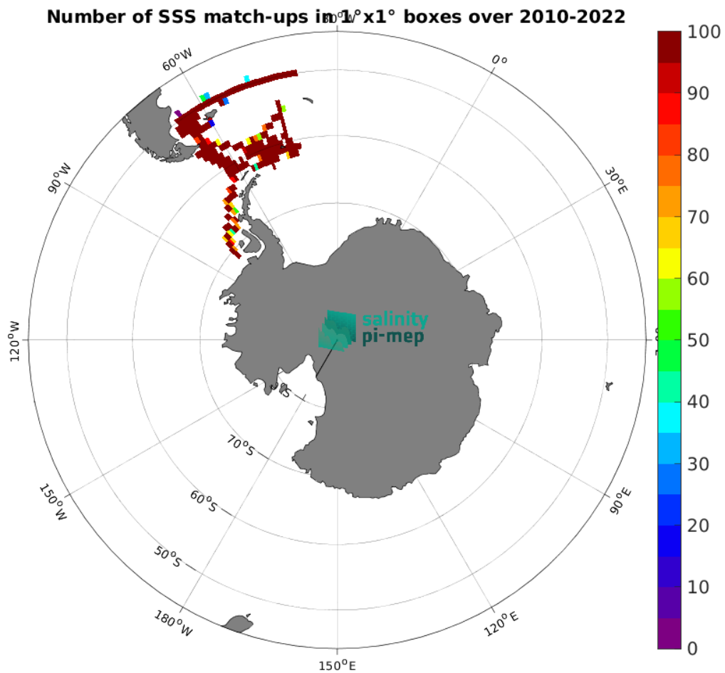
Figure 4: Number of SSS match-ups between TSG (CSIC-UTM) SSS and the CCI SSS L4 POLAR SH Merged-OI v4.4 - 30-day running (ESA) SSS product for the Southern Ocean Pi-MEP region over 1^\circ \times 1^\circ boxes and for the full satellite product period.
