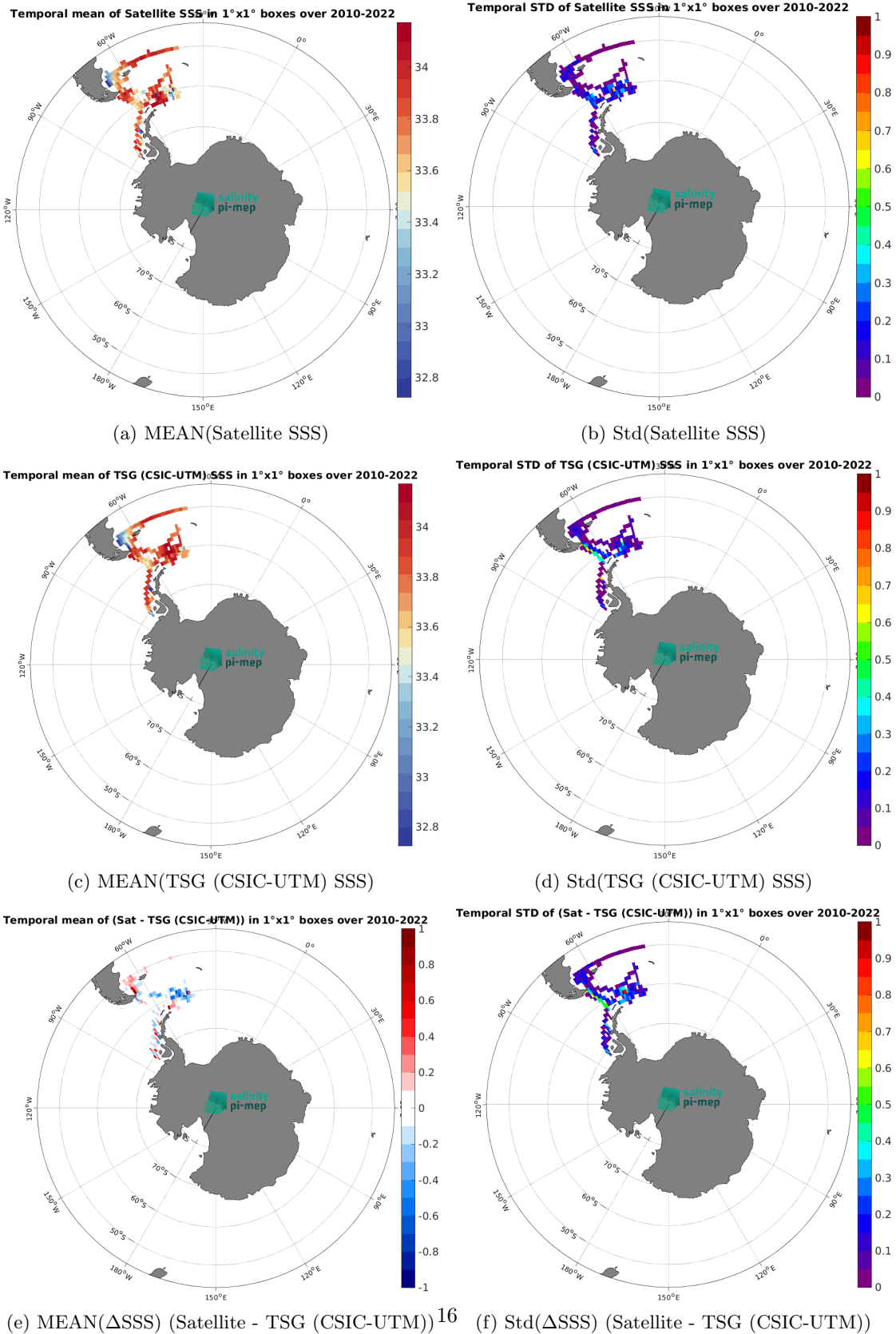
Figure 6: Temporal mean (left) and Std (right) of SSS from CCI SSS L4 POLAR SH Merged-OI v4.4 - 30-day running (ESA) (top), TSG (CSIC-UTM) (middle), and of \Delta SSS (Satellite - TSG (CSIC-UTM)). Only match-up pairs are used to generate these maps.
