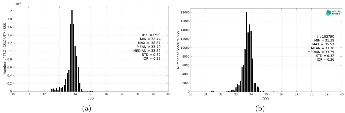
Figure 2: Histograms of SSS from TSG (CSIC-UTM) (a) and CCI SSS L4 POLAR SH Merged-OI v4.4 - 30-day running (ESA) (b) considering all match-up pairs per bins of 0.1 over the Southern Ocean Pi-MEP region and for the full satellite product period.
