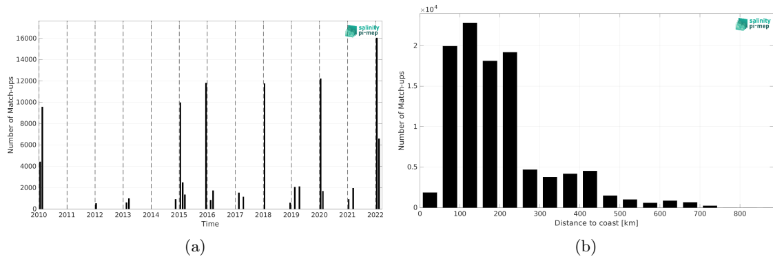
Figure 1: Number of match-ups between TSG (CSIC-UTM) and CCI SSS L4 POLAR SH Merged-OI v4.4 - 30-day running (ESA) SSS as a function of time (a) and as function of the distance to coast (b) over the Southern Ocean Pi-MEP region and for the full satellite product period.
