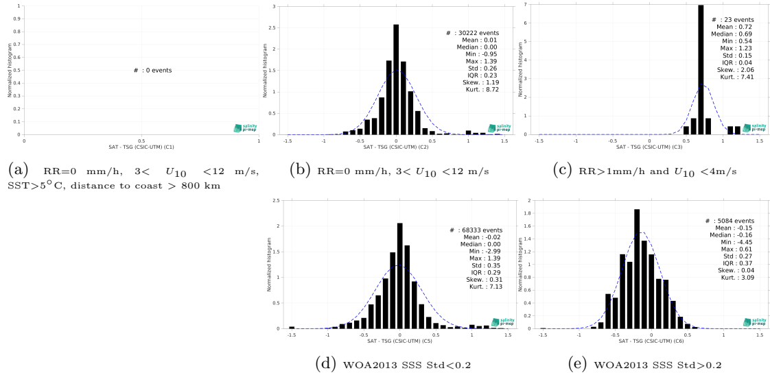
Figure 13: Normalized histogram of \Delta\text{SSS} (CCI SSS L4 POLAR SH Merged-OI v4.4 - 30-day running (ESA) - TSG (CSIC-UTM)) for 5 different subdatasets corresponding to: RR=0 mm/h, 3 < U_{10} < 12 m/s, SST >5^{\circ}\text{C} , distance to coast > 800 km (a), RR=0 mm/h, 3 < U_{10} < 12 m/s (b), RR>1\text{mm/h} and U_{10} < 4\text{m/s} (c), WOA2013 SSS Std <0.2 (d), WOA2013 SSS Std >0.2 (e).
