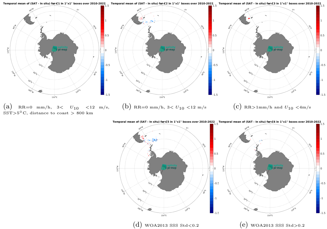
Figure 12: Temporal mean gridded over spatial boxes of size 1^{\circ}\times 1^{\circ} of \Delta\text{SSS} (CCI SSS L4 POLAR SH Merged-OI v4.4 - 30-day running (ESA) - TSG (CSIC-UTM)) for 5 different subdatasets corresponding to:RR=0 mm/h, 3 < U_{10} < 12 m/s, SST >5^{\circ}\text{C} , distance to coast > 800 km (a), RR=0 mm/h, 3 < U_{10} < 12 m/s (b), RR >1 mm/h and U_{10} < 4 m/s (c), WOA2013 SSS Std <0.2 (d), WOA2013 SSS Std >0.2 (e).
