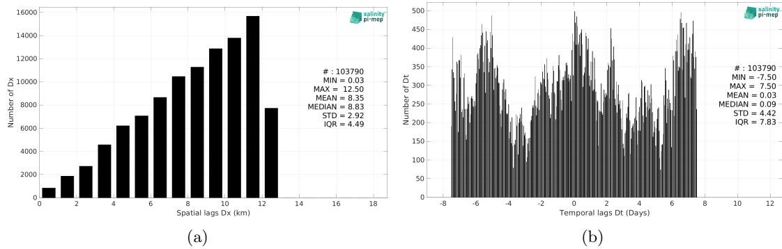
Figure 5: Histograms of the spatial (a) and temporal (b) lags between the location/time of the TSG (CSIC-UTM) measurement and the date of the corresponding CCI SSS L4 POLAR SH Merged-OI v4.4 - 30-day running (ESA) SSS pixel.
