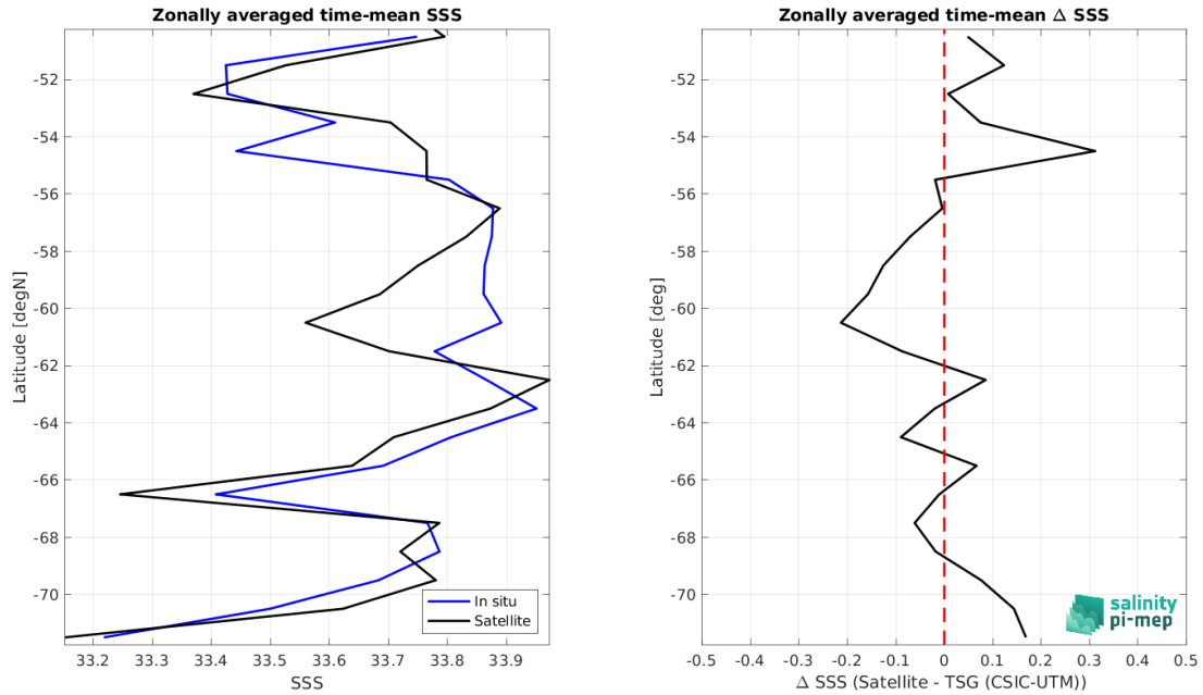
Figure 8: Left panel: Zonal mean SSS from CCI SSS L4 POLAR SH Merged-OI v4.4 - 30-day running (ESA) satellite product (black) and from TSG (CSIC-UTM) (blue). Right panel: Zonal mean of \Delta SSS (Satellite - TSG (CSIC-UTM)) for all the collected Pi-MEP match-up pairs estimated over the full satellite product period.
