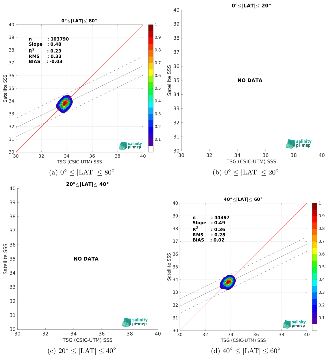
Figure 9: Contour maps of the concentration of CCI SSS L4 POLAR SH Merged-OI v4.4 - 30-day running (ESA) SSS (y-axis) versus TSG (CSIC-UTM) SSS (x-axis) at match-up pairs for different latitude bands. For each plot, the red line shows x=y . The black thin and dashed lines indicate a linear fit through the data cloud and the \pm 95\% confidence levels, respectively. The number match-up pairs n , the slope and R^2 coefficient of the linear fit, the root mean square (RMS) and the mean bias between satellite and in situ data are indicated for each latitude band in each plots.
