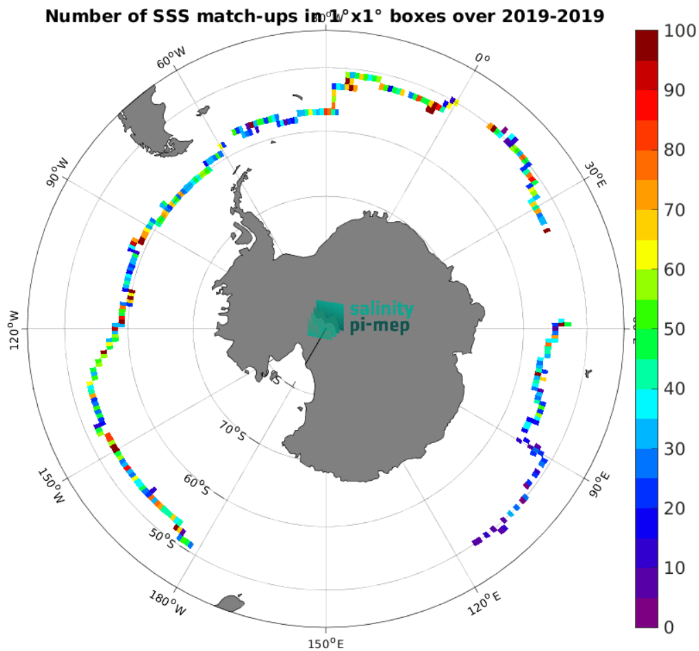
Figure 4: Number of SSS match-ups between Saildrone SSS and the CCI SSS L4 POLAR SH Merged-OI v4.4 - 30-day running (ESA) SSS product for the Southern Ocean Pi-MEP region over 1^{\circ} \times 1^{\circ} boxes and for the full satellite product period.
