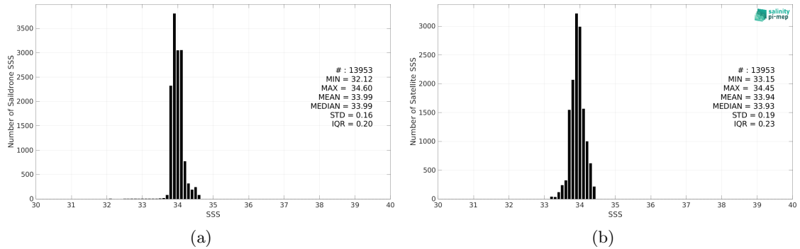
Figure 2: Histograms of SSS from Saildrone (a) and CCI SSS L4 POLAR SH Merged-OI v4.4 - 30-day running (ESA) (b) considering all match-up pairs per bins of 0.1 over the Southern Ocean Pi-MEP region and for the full satellite product period.
