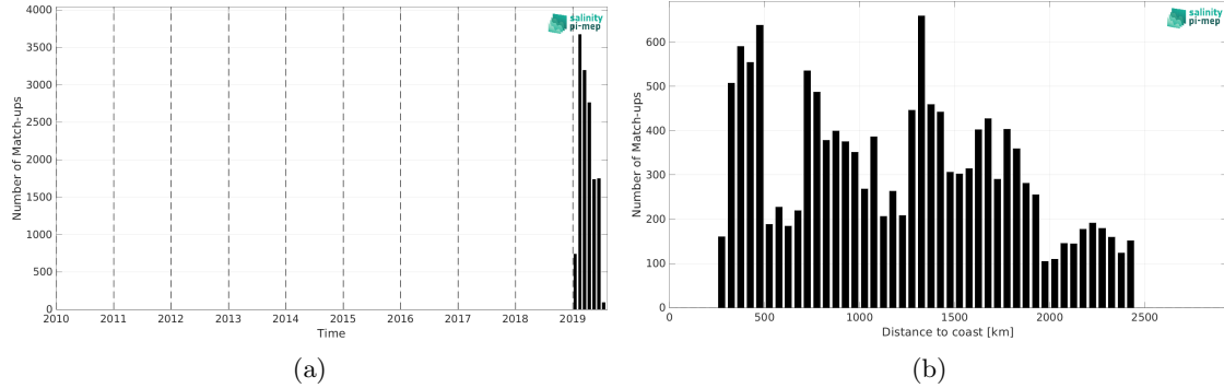
Figure 1: Number of match-ups between Saildrone and CCI SSS L4 POLAR SH Merged-OI v4.4 - 30-day running (ESA) SSS as a function of time (a) and as function of the distance to coast (b) over the Southern Ocean Pi-MEP region and for the full satellite product period.
