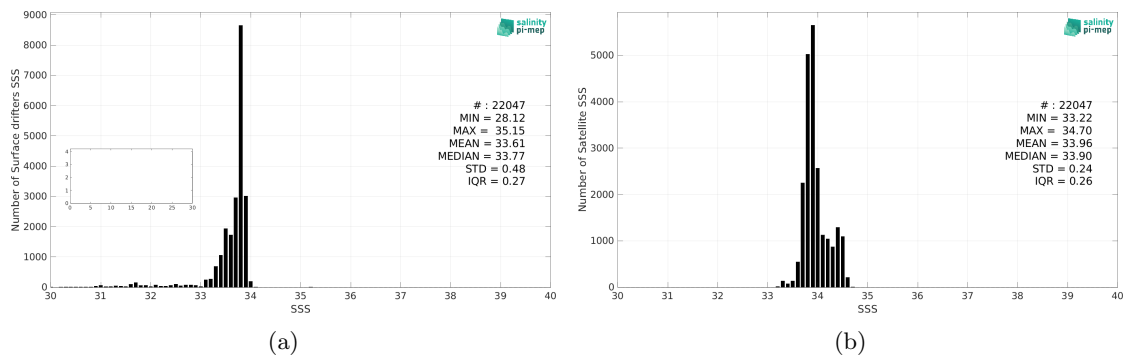
Figure 2: Histograms of SSS from Surface drifters (a) and CCI SSS L4 POLAR SH Merged-OI v4.4 - 30-day running (ESA) (b) considering all match-up pairs per bins of 0.1 over the Southern Ocean Pi-MEP region and for the full satellite product period.
