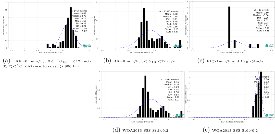
Figure 12: Normalized histogram of \Delta\text{SSS} (CCI SSS L4 POLAR SH Merged-OI v4.4 - 30-day running (ESA) - Surface drifters) for 5 different subdatasets corresponding to: RR=0 mm/h, 3 < U_{10} < 12 m/s, SST > 5^{\circ}\text{C} , distance to coast > 800 km (a), RR=0 mm/h, 3 < U_{10} < 12 m/s (b), RR > 1\text{mm/h} and U_{10} < 4\text{m/s} (c), WOA2013 SSS Std < 0.2 (d), WOA2013 SSS Std > 0.2 (e).
