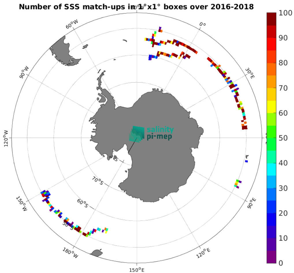
Figure 3: Number of SSS match-ups between Surface drifters SSS and the CCI SSS L4 POLAR SH Merged-OI v4.4 - 30-day running (ESA) SSS product for the Southern Ocean Pi-MEP region over 1^\circ \times 1^\circ boxes and for the full satellite product period.
