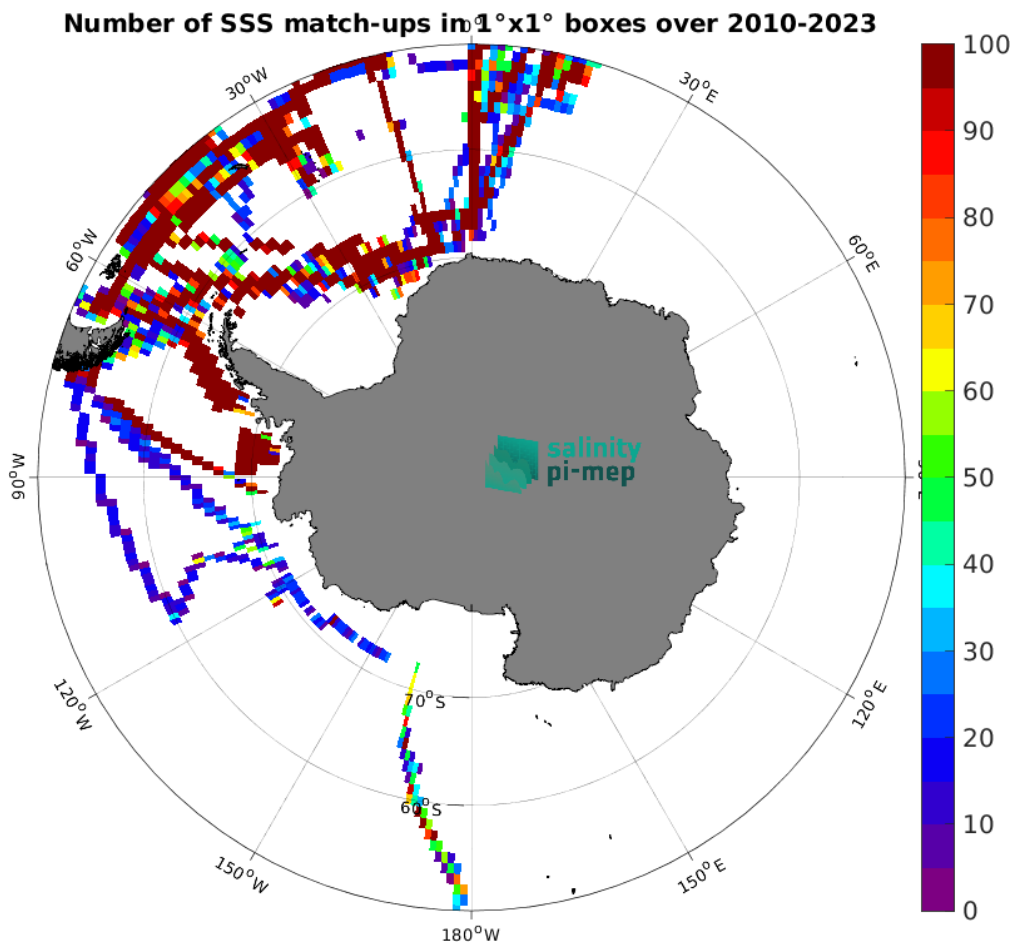
Figure 5: Number of SSS match-ups between TSG (Polarstern) SSS and the CCI SSS L4 Merged-OI v5.5 - 7-day running (ESA) SSS product for the Southern Ocean Pi-MEP region over 1^\circ \times 1^\circ boxes and for the full satellite product period.
