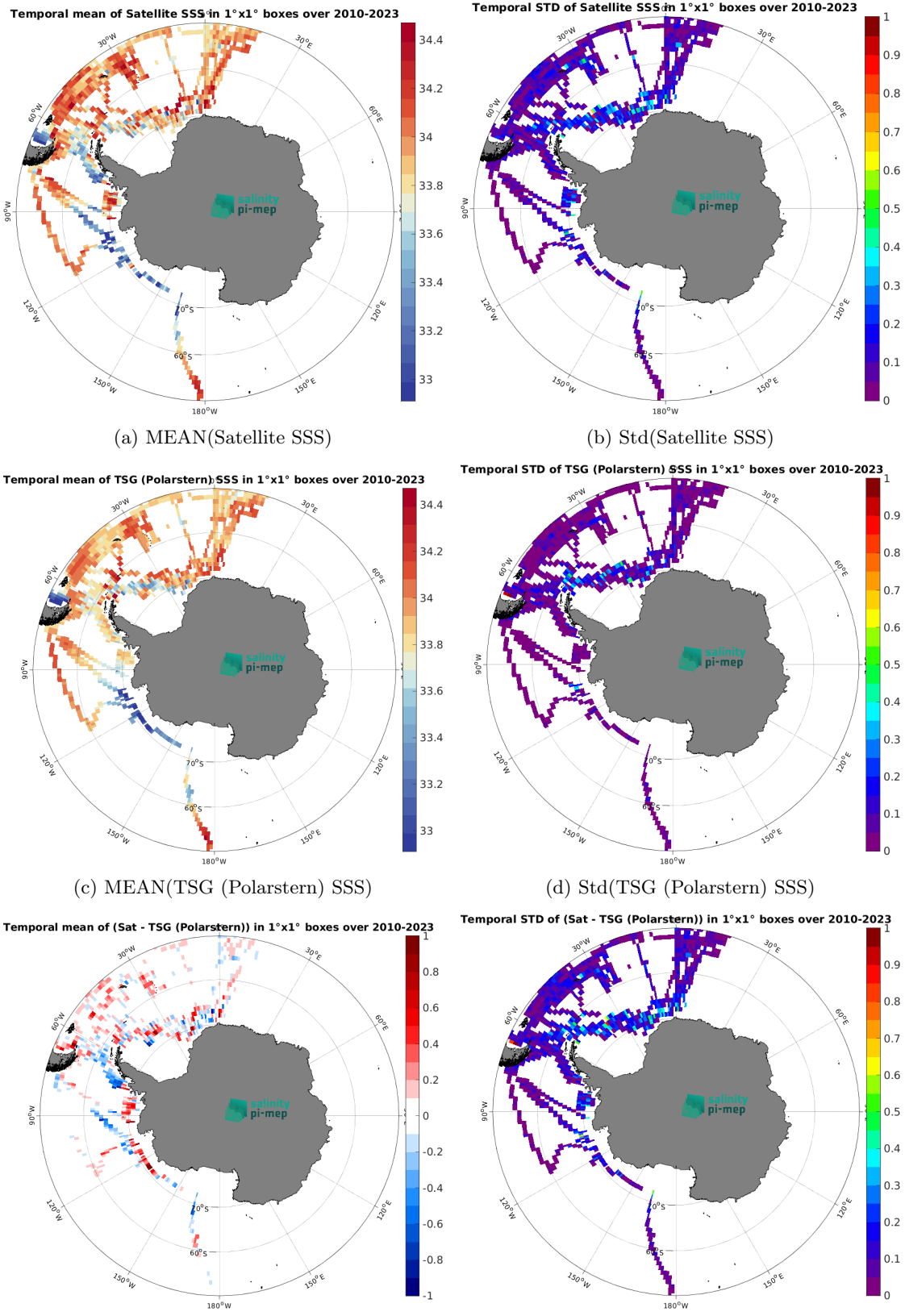
Figure 7: Temporal mean (left) and Std (right) of SSS from CCI SSS L4 Merged-OI v5.5 - 7-day running (ESA) (top), TSG (Polarstern) (middle), and of \Delta SSS (Satellite - TSG (Polarstern)). Only match-up pairs are used to generate these maps.
