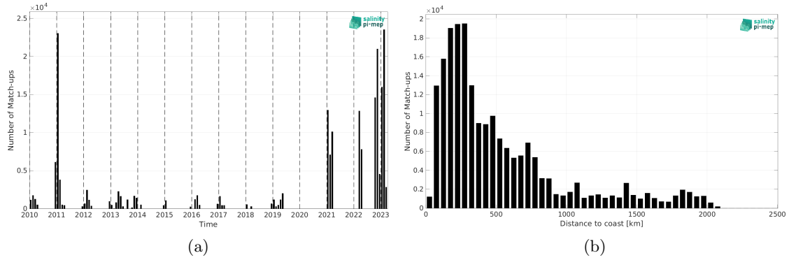
Figure 2: Number of match-ups between TSG (Polarstern) and CCI SSS L4 Merged-OI v5.5 - 7-day running (ESA) SSS as a function of time (a) and as function of the distance to coast (b) over the Southern Ocean Pi-MEP region and for the full satellite product period.
