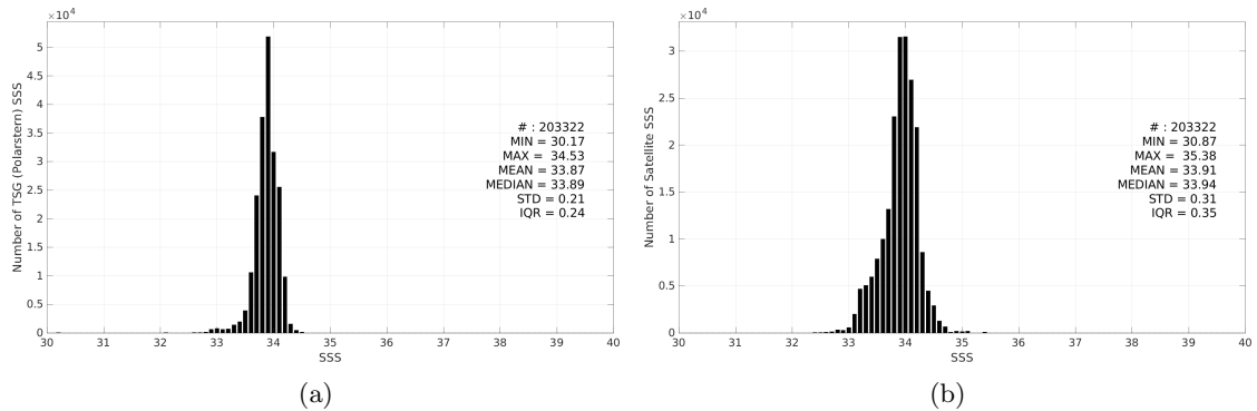
Figure 3: Histograms of SSS from TSG (Polarstern) (a) and CCI SSS L4 Merged-OI v5.5 - 7-day running (ESA) (b) considering all match-up pairs per bins of 0.1 over the Southern Ocean Pi-MEP region and for the full satellite product period.
