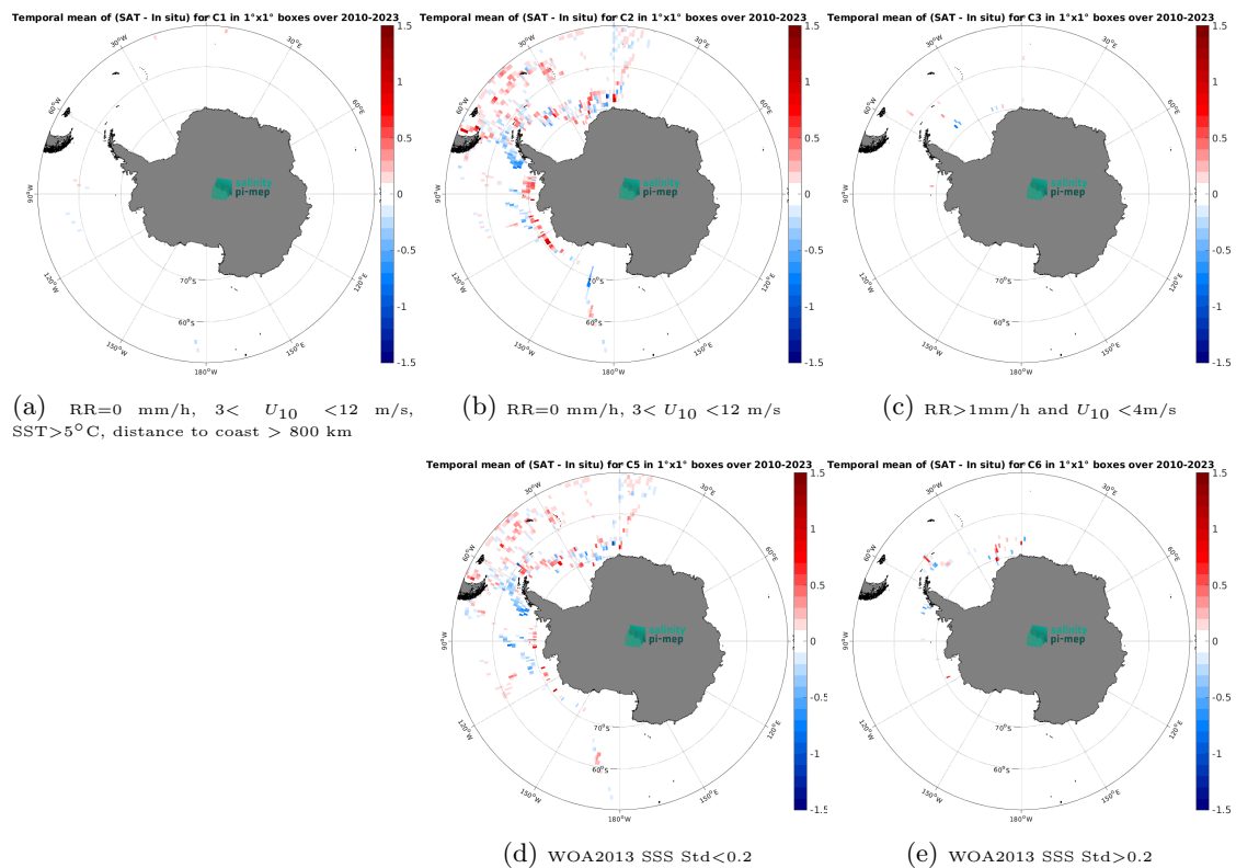
Figure 14: Temporal mean gridded over spatial boxes of size 1^\circ \times 1^\circ of \Delta\text{SSS} (CCI SSS L4 Merged-OI v5.5 - 7-day running (ESA) - TSG (Polarstern)) for 5 different subdatasets corresponding to:RR=0 mm/h, 3 < U_{10} < 12 m/s, SST > 5^\circ\text{C} , distance to coast > 800 km (a), RR=0 mm/h, 3 < U_{10} < 12 m/s (b), RR > 1 mm/h and U_{10} < 4 m/s (c), WOA2013 SSS Std < 0.2 (d), WOA2013 SSS Std > 0.2 (e).
