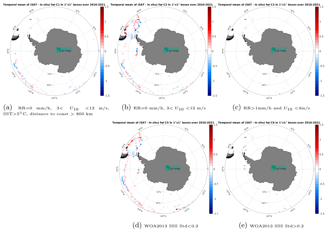
Figure 14: Temporal mean gridded over spatial boxes of size 1^\circ \times 1^\circ of \Delta\text{SSS} (CCI SSS L4 Merged-OI v5.5 - 7-day running (ESA) - TSG (GOSUD-Sailing-ship)) for 5 different subdatasets corresponding to:RR=0 mm/h, 3 < U_{10} < 12 m/s, SST >5^\circ\text{C} , distance to coast > 800 km (a), RR=0 mm/h, 3 < U_{10} < 12 m/s (b), RR >1 mm/h and U_{10} < 4 m/s (c), WOA2013 SSS Std <0.2 (d), WOA2013 SSS Std >0.2 (e).
