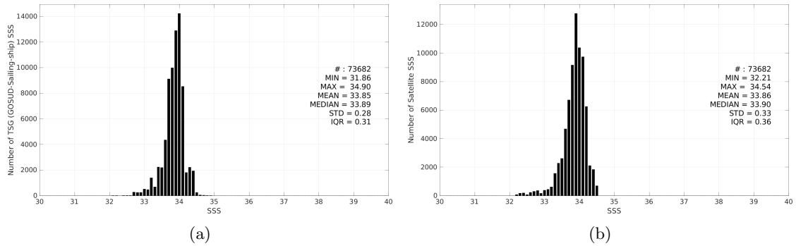
Figure 3: Histograms of SSS from TSG (GOSUD-Sailing-ship) (a) and CCI SSS L4 Merged-OI v5.5 - 7-day running (ESA) (b) considering all match-up pairs per bins of 0.1 over the Southern Ocean Pi-MEP region and for the full satellite product period.
