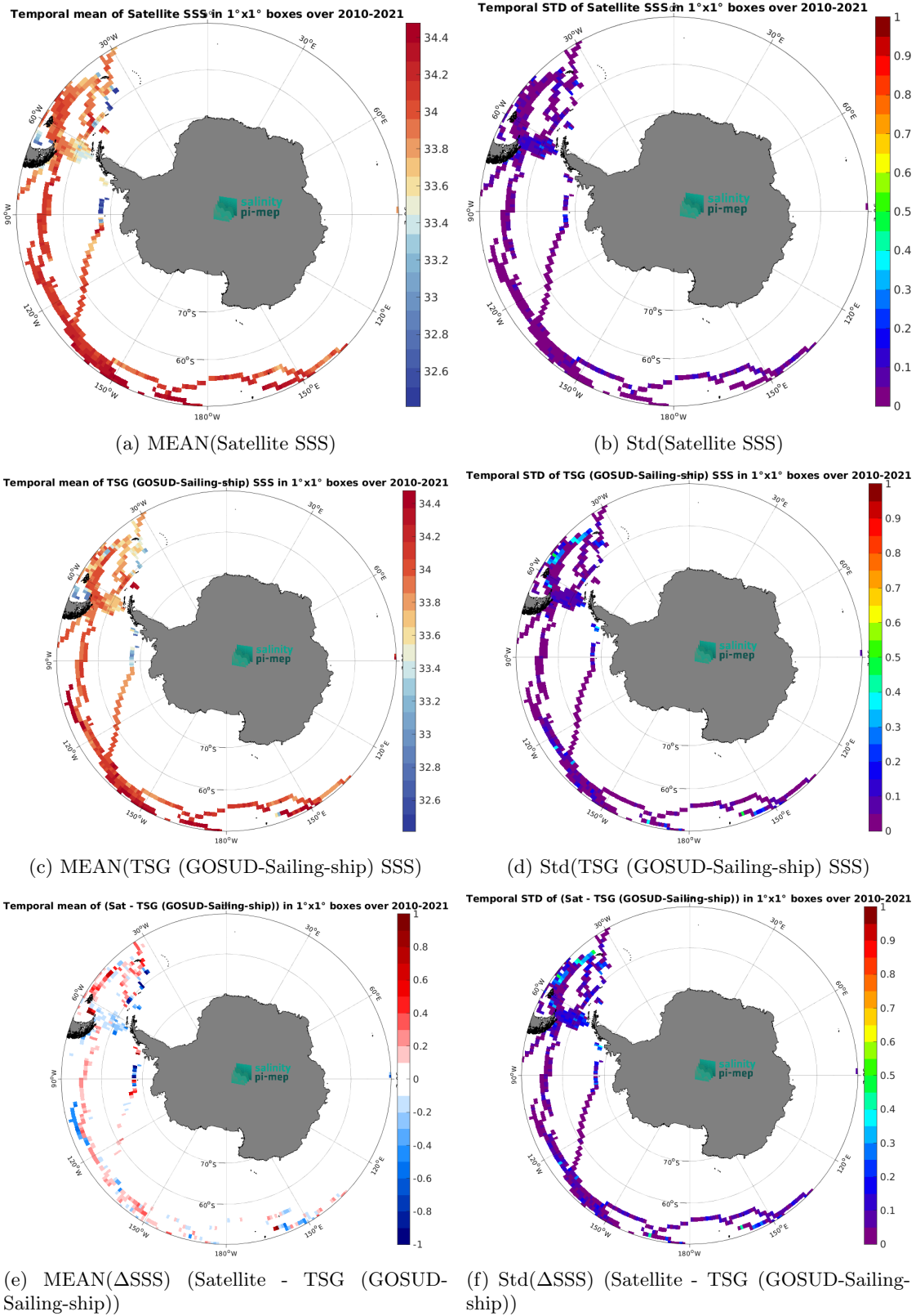
Figure 7: Temporal mean (left) and Std (right) of SSS from CCI SSS L4 Merged-OI v5.5 - 7-day running (ESA) (top), TSG (GOSUD-Sailing-ship) (middle), and of \Delta SSS (Satellite - TSG (GOSUD-Sailing-ship)). Only match-up pairs are used to generate these maps.
