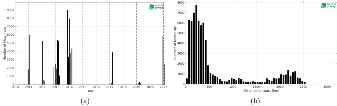
Figure 2: Number of match-ups between TSG (GOSUD-Sailing-ship) and CCI SSS L4 Merged-OI v5.5 - 7-day running (ESA) SSS as a function of time (a) and as function of the distance to coast (b) over the Southern Ocean Pi-MEP region and for the full satellite product period.
