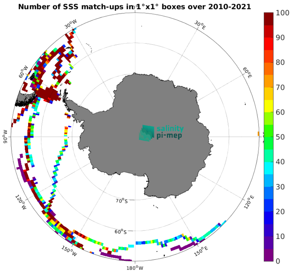
Figure 5: Number of SSS match-ups between TSG (GOSUD-Sailing-ship) SSS and the CCI SSS L4 Merged-OI v5.5 - 7-day running (ESA) SSS product for the Southern Ocean Pi-MEP region over 1^\circ \times 1^\circ boxes and for the full satellite product period.
